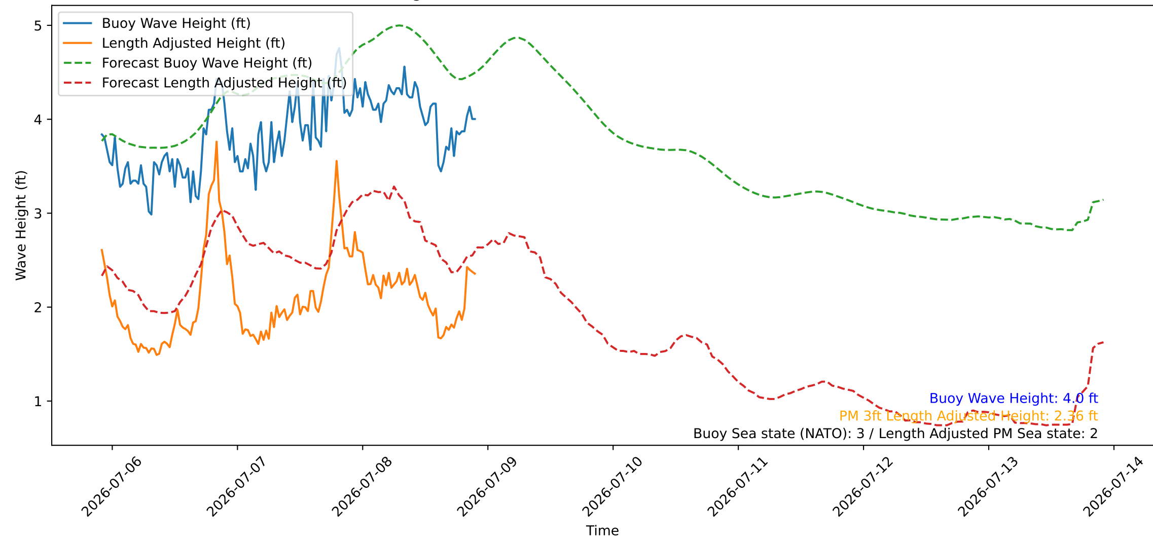
Wave Heights over Time for Green Beach at 2026-07-08 22:11:10
