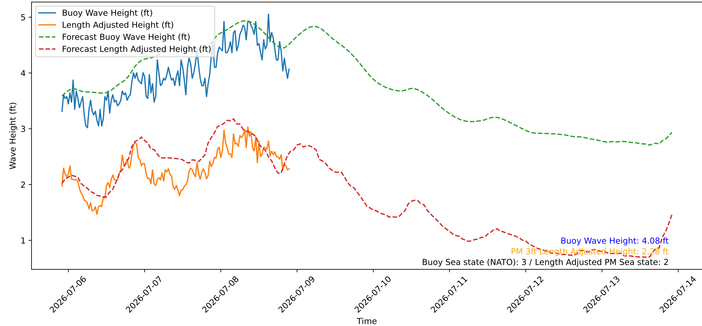
Wave Heights over Time for Oceanside Harbor at 2026-07-08 22:10:27
