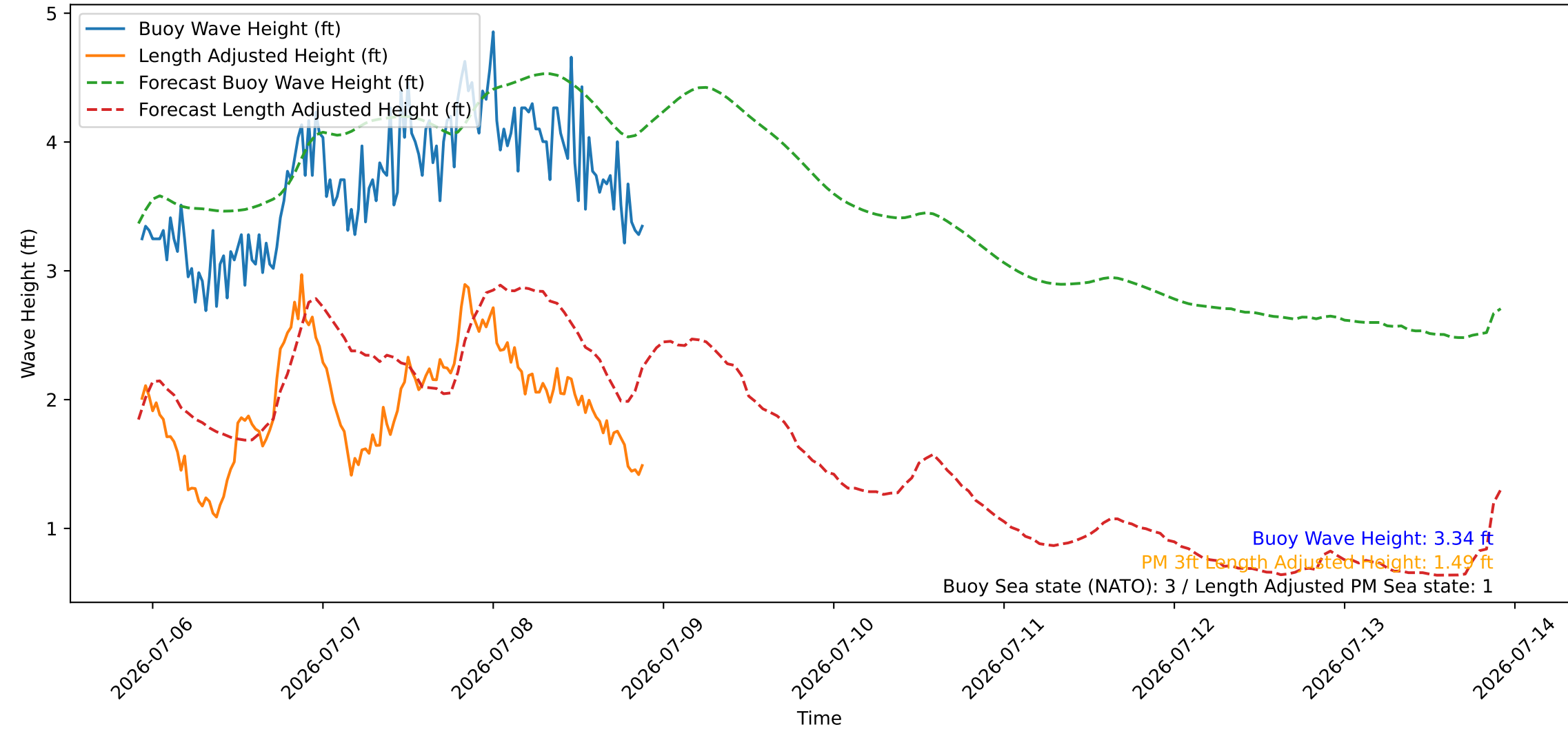
Wave Heights over Time for Red Beach at 2026-07-08 22:10:47
