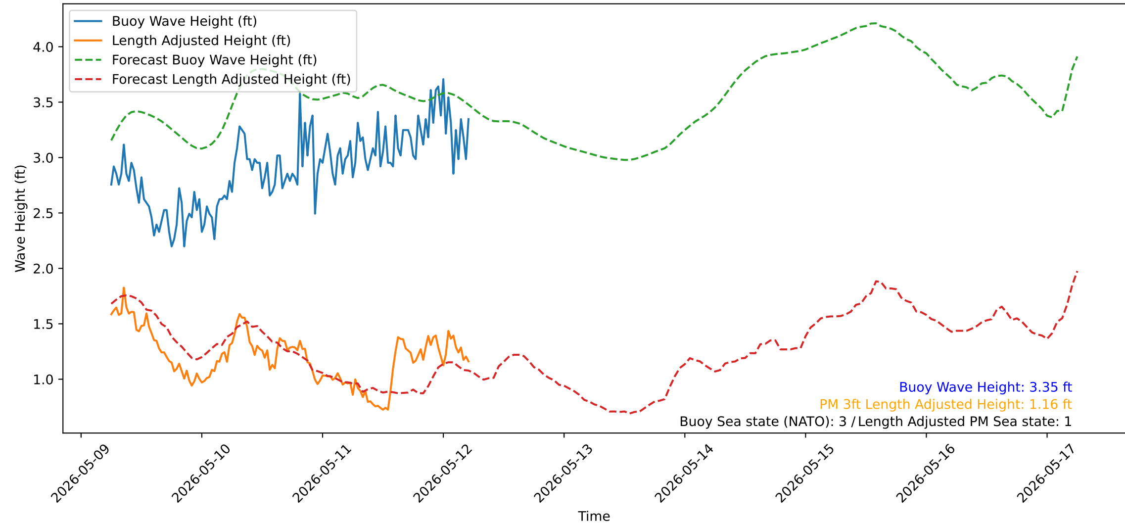
Wave Heights over Time for Oceanside Harbor at 2026-05-12 06:00:31
