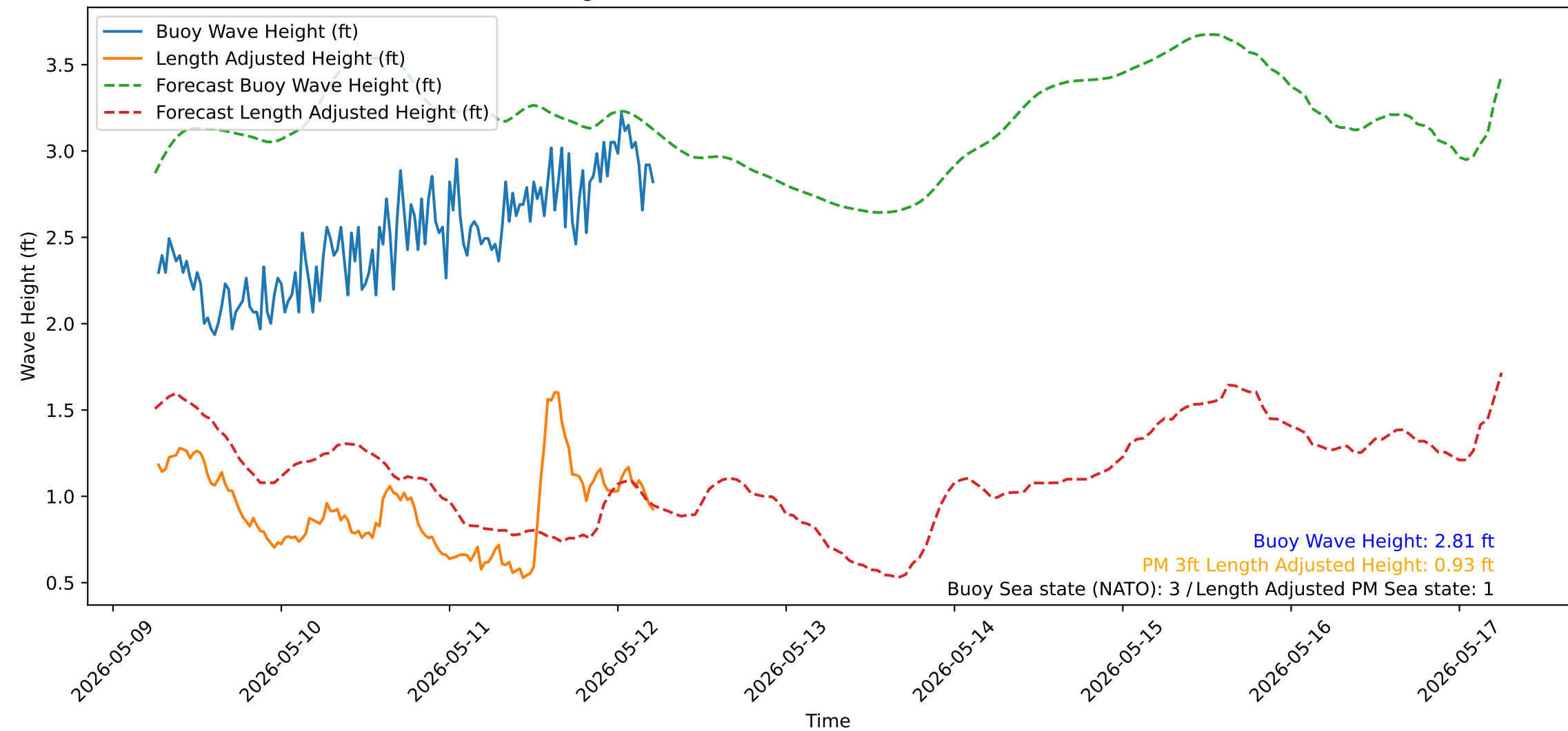
Wave Heights over Time for Red Beach at 2026-05-12 06:00:50
