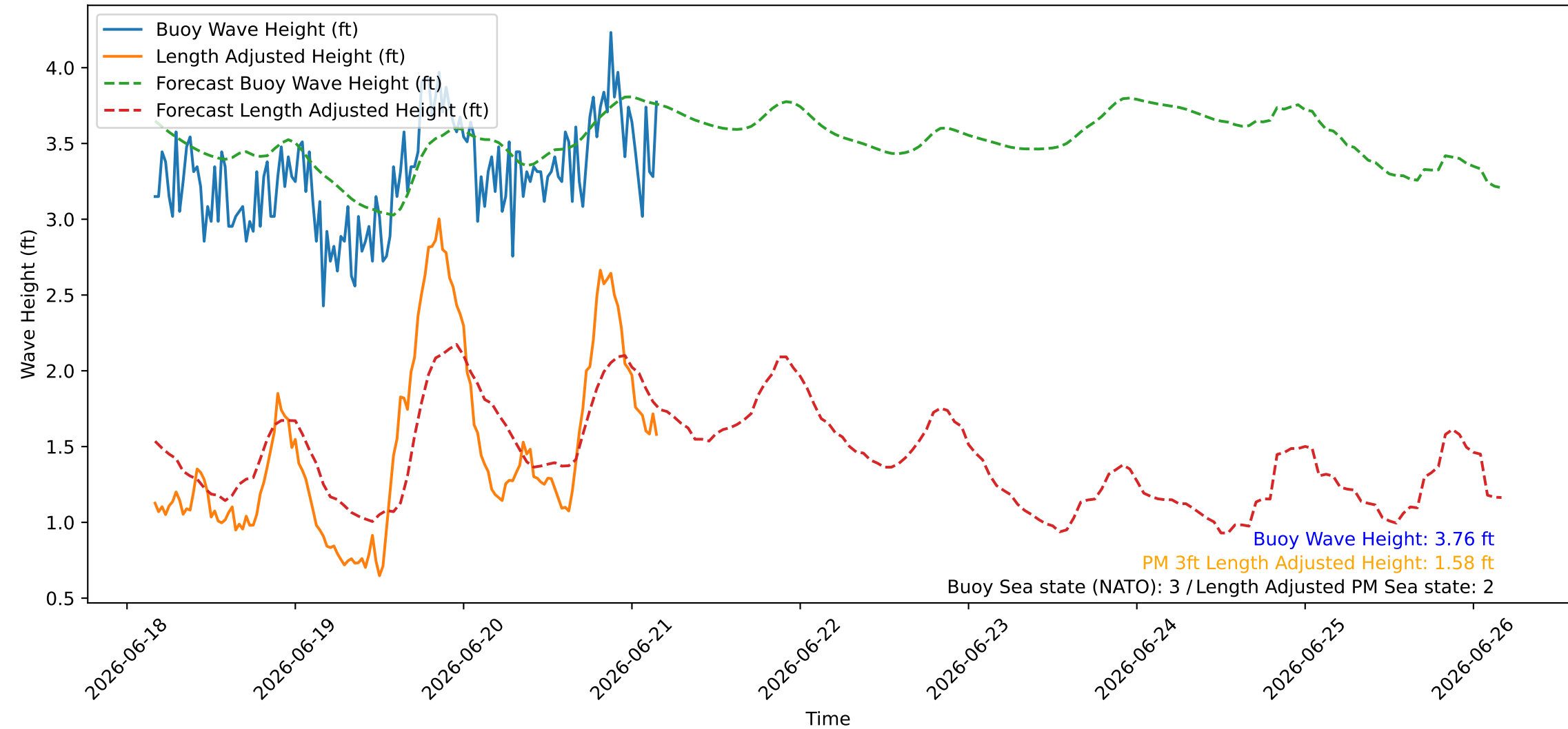
Wave Heights over Time for Green Beach at 2026-06-21 04:11:08
