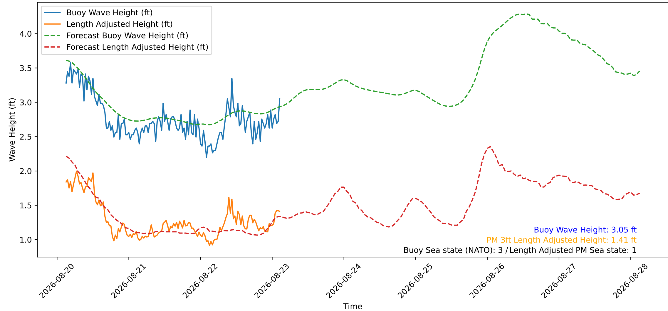
Wave Heights over Time for Oceanside Harbor at 2026-08-23 03:10:29
