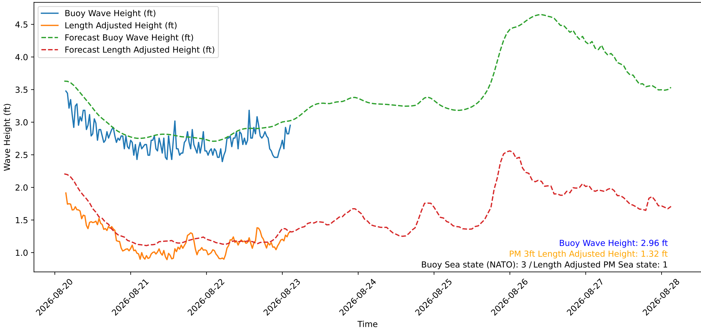
Wave Heights over Time for Green Beach at 2026-08-23 03:11:11
