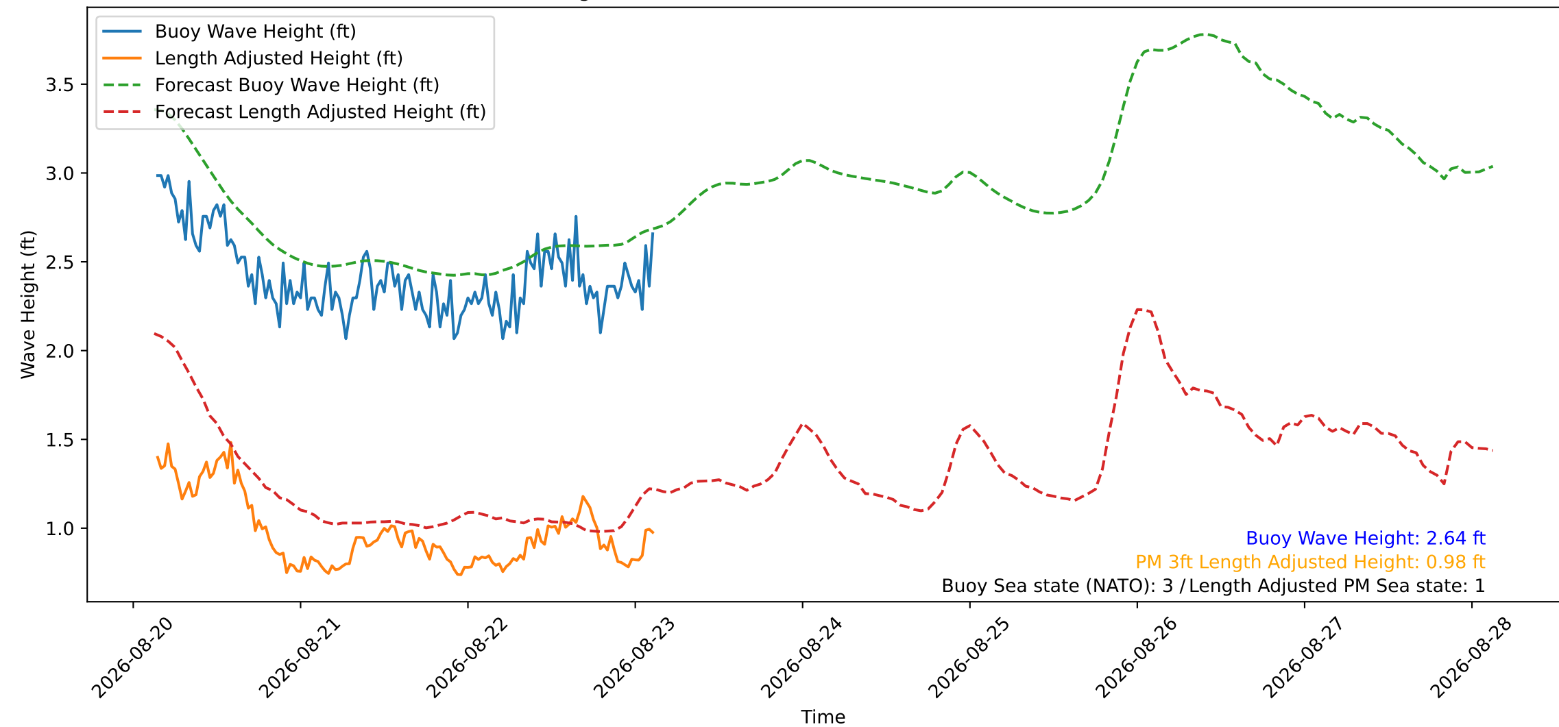
Wave Heights over Time for Red Beach at 2026-08-23 03:10:49
