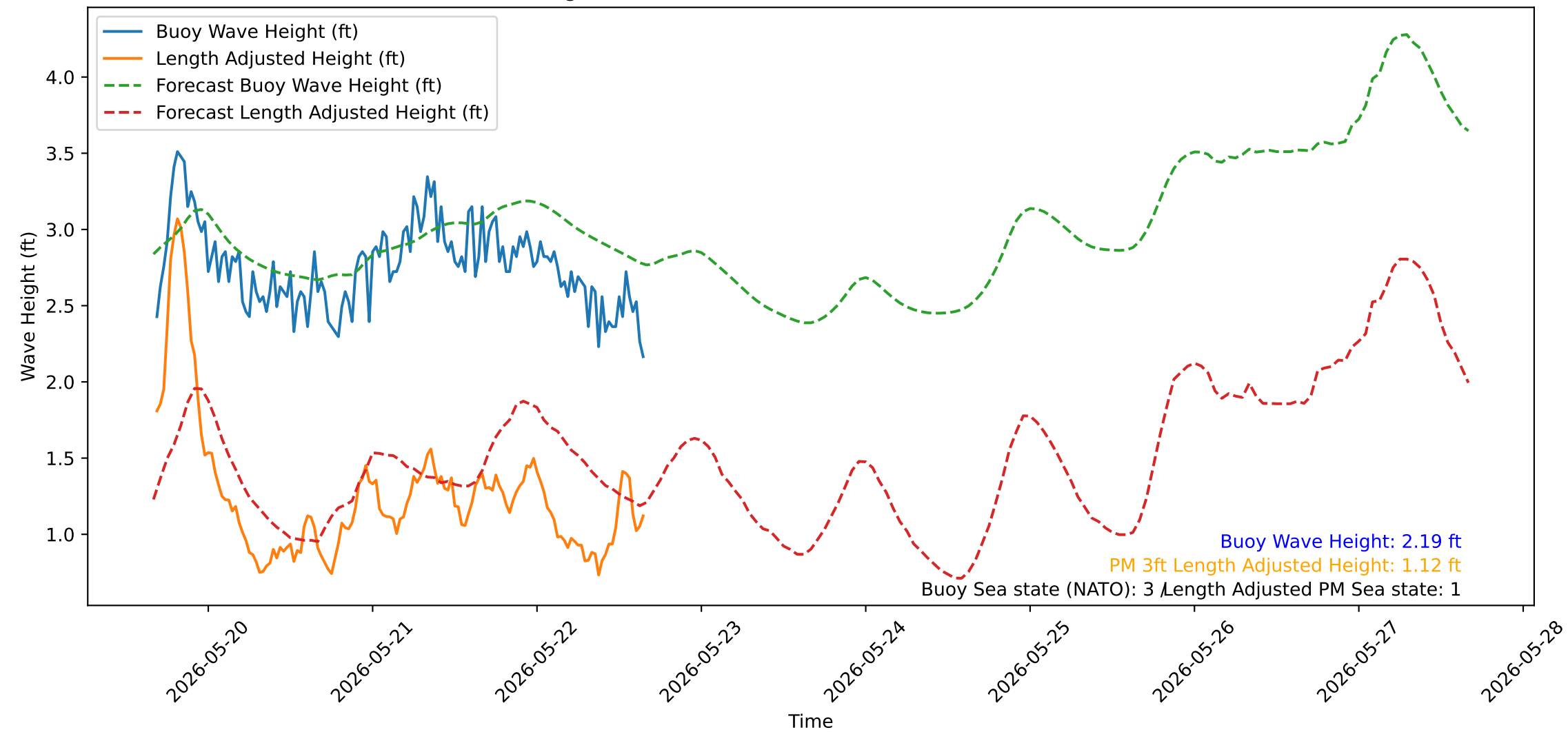
Wave Heights over Time for Red Beach at 2026-05-22 16:20:52
