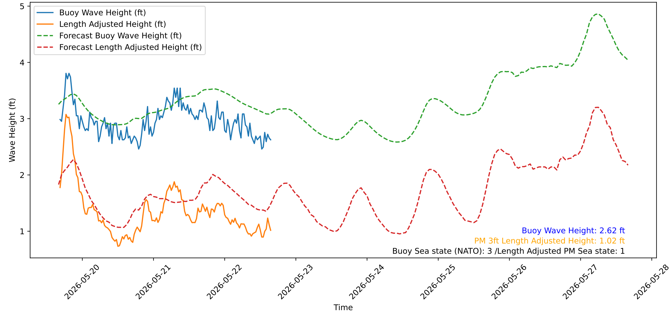
Wave Heights over Time for Green Beach at 2026-05-22 16:21:15
