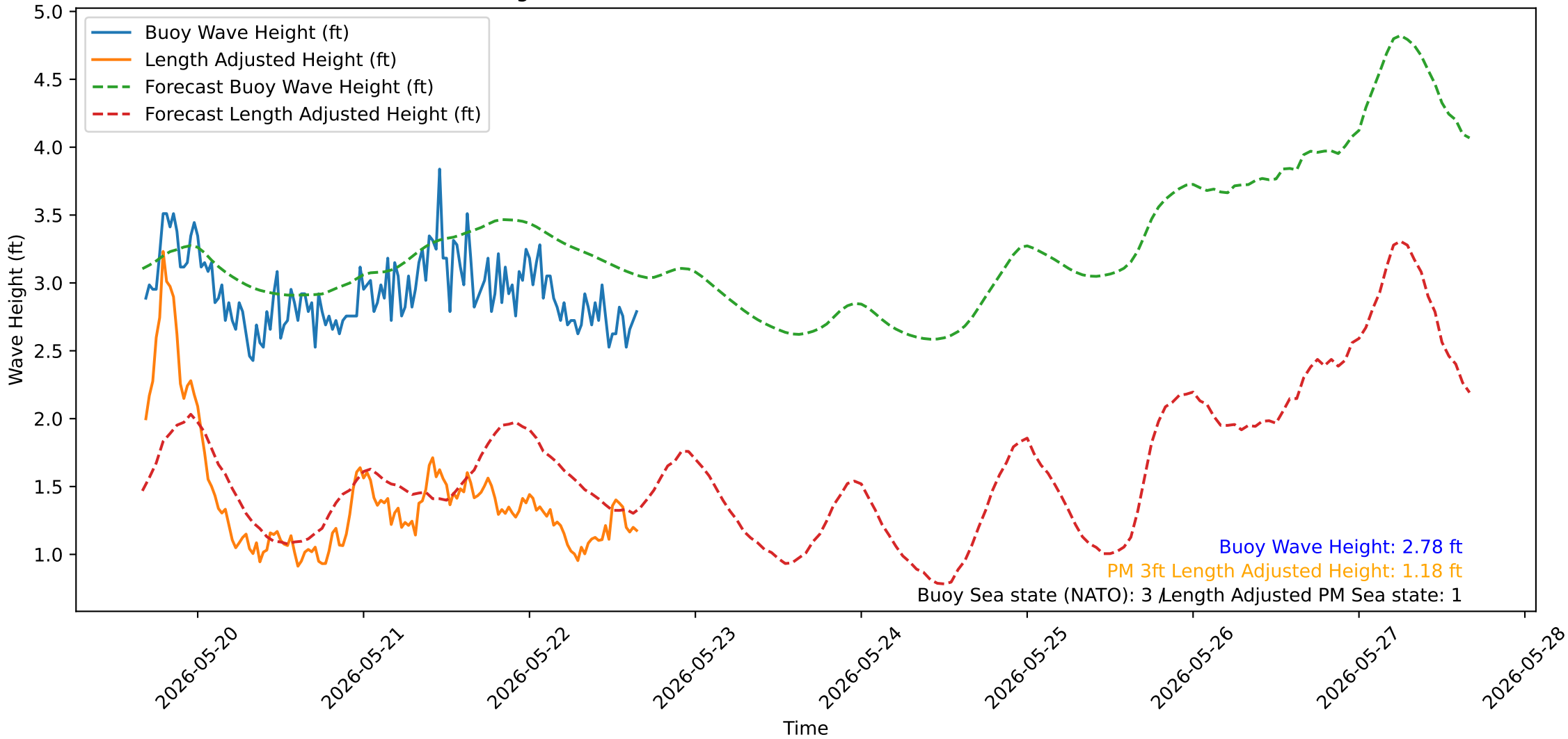
Wave Heights over Time for Oceanside Harbor at 2026-05-22 16:20:31
