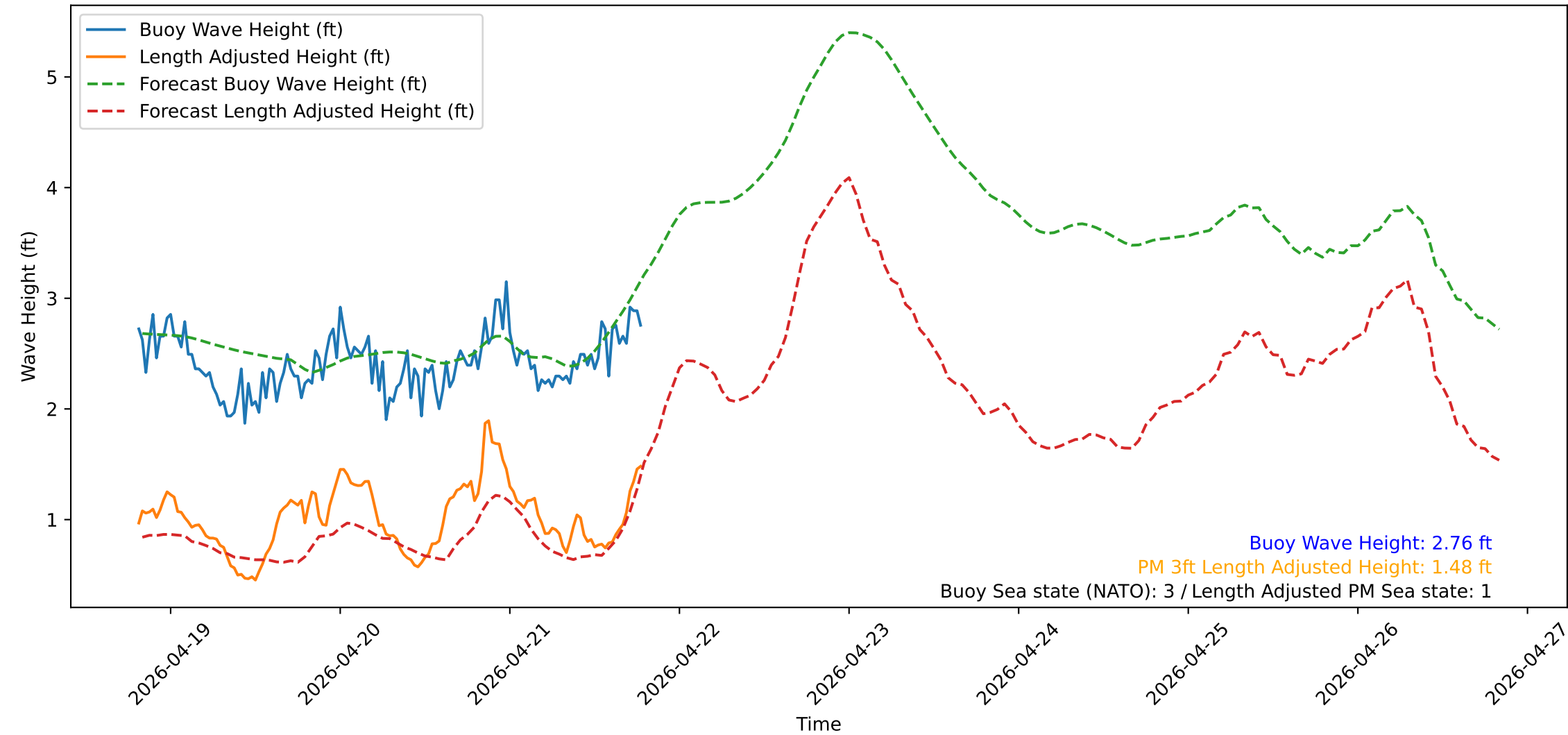
Wave Heights over Time for Green Beach at 2026-04-21 19:31:12
