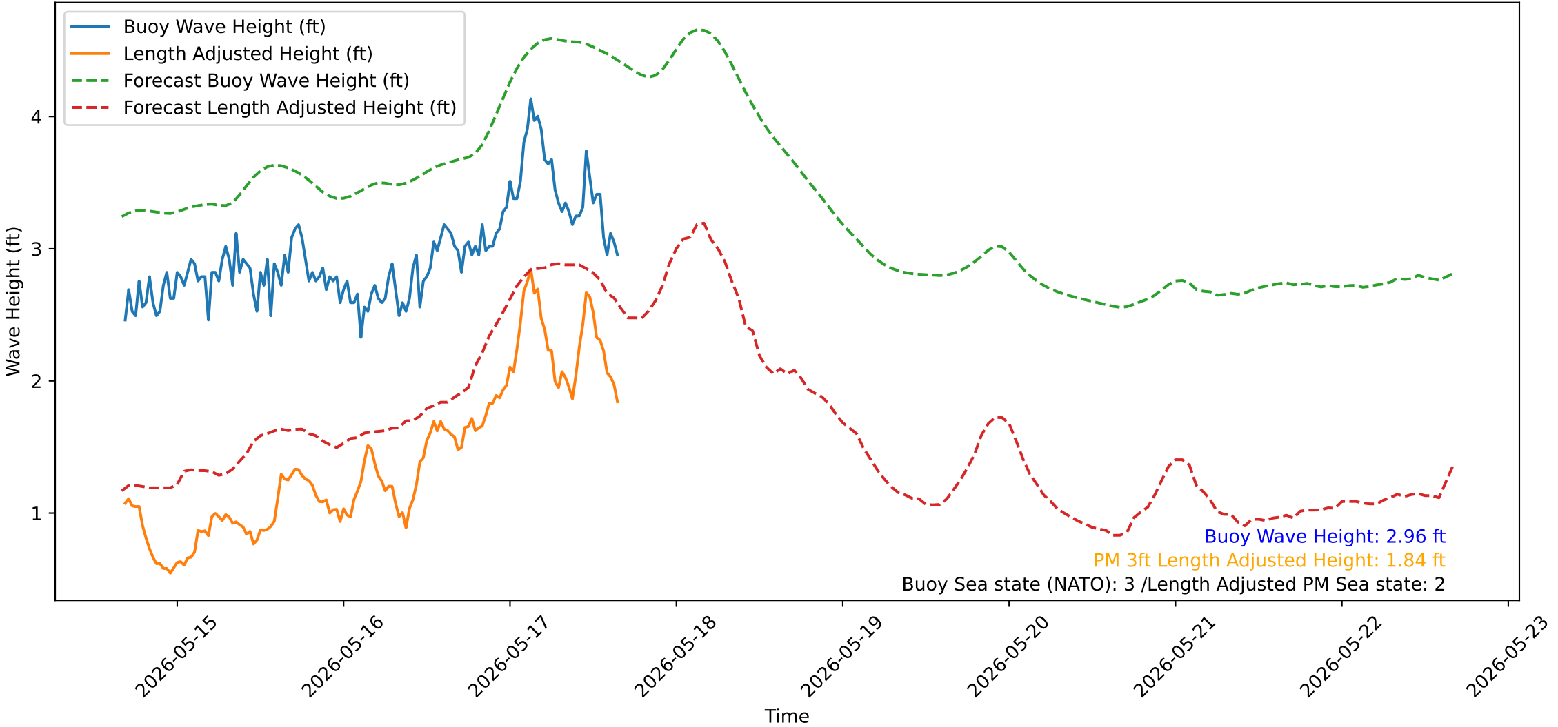
Wave Heights over Time for Red Beach at 2026-05-17 16:20:52
