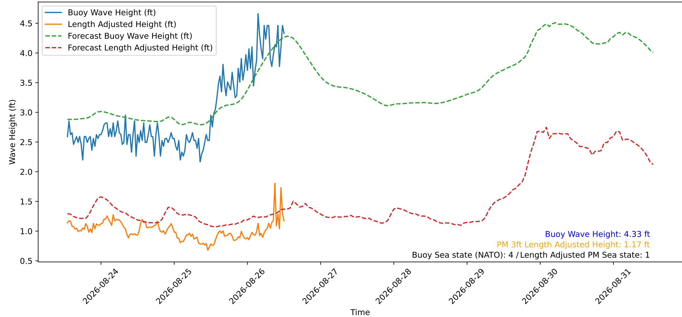
Wave Heights over Time for Red Beach at 2026-08-26 12:40:53
