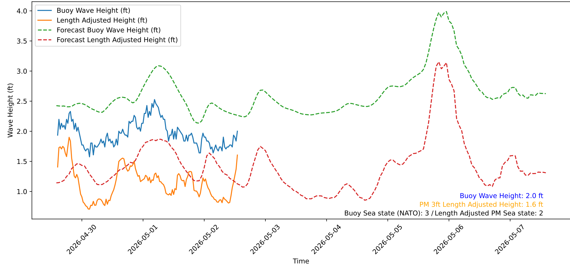
Wave Heights over Time for Red Beach at 2026-05-02 14:00:50
