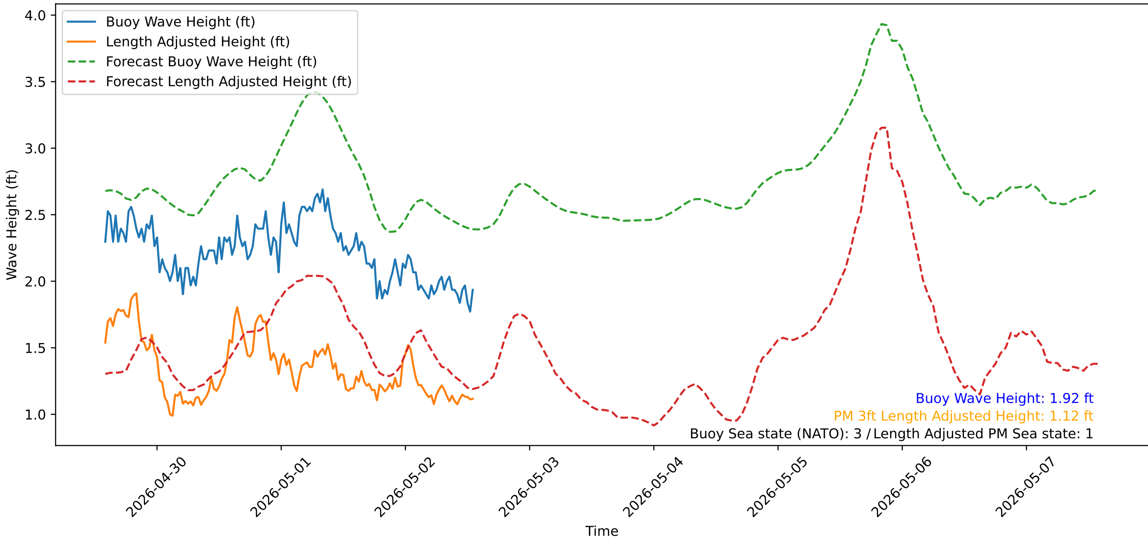
Wave Heights over Time for Oceanside Harbor at 2026-05-02 14:00:31
