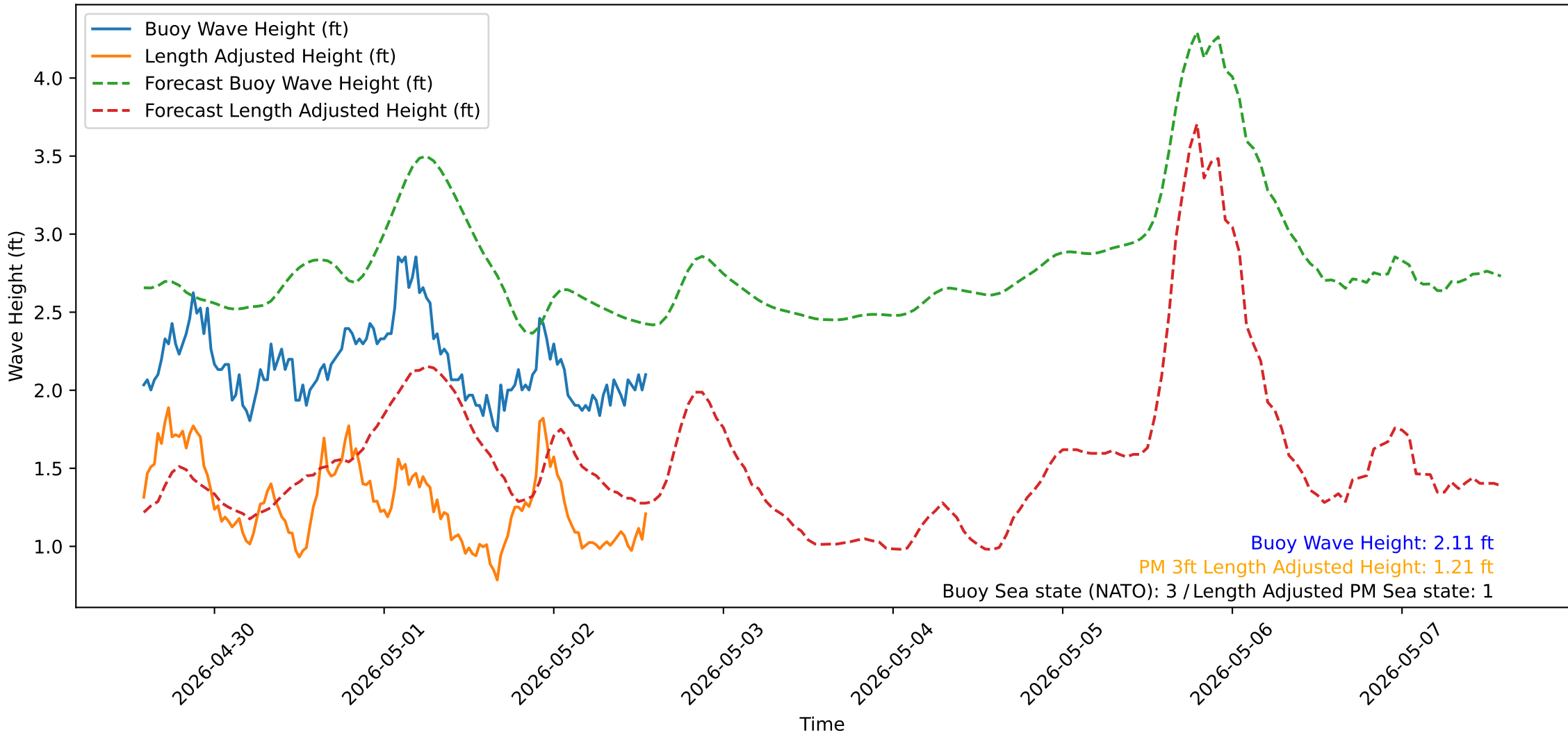
Wave Heights over Time for Green Beach at 2026-05-02 14:01:13
