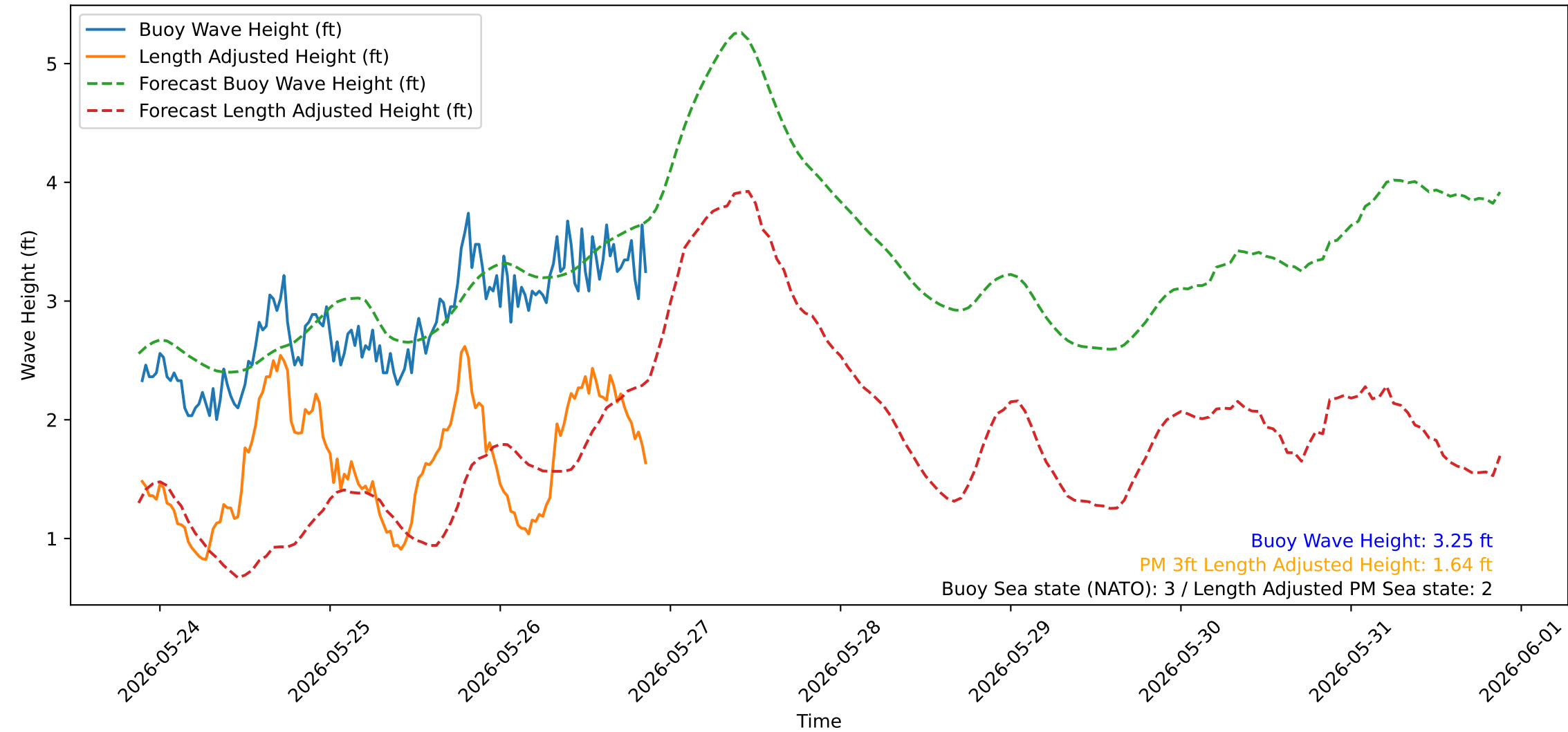
Wave Heights over Time for Red Beach at 2026-05-26 21:20:48
