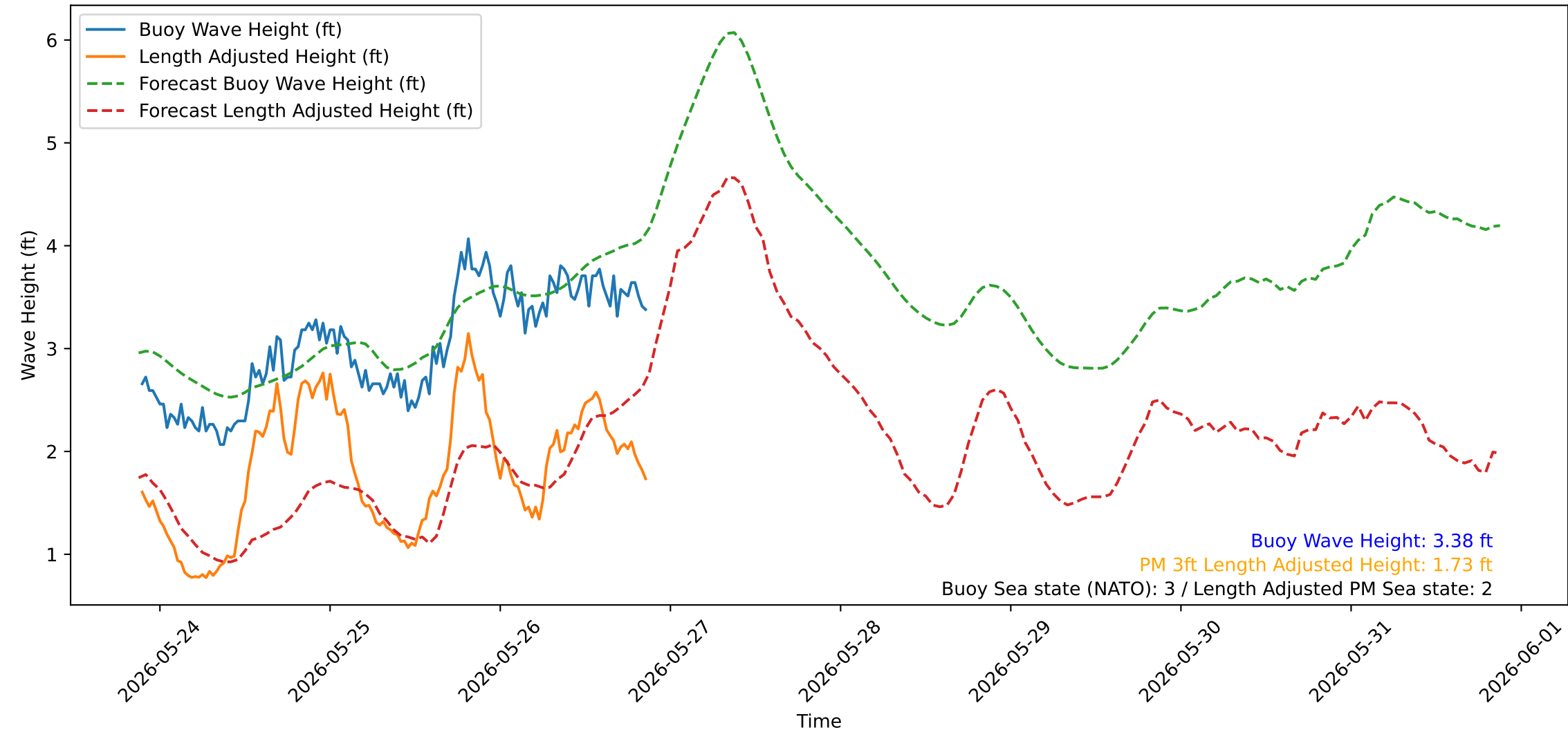
Wave Heights over Time for Green Beach at 2026-05-26 21:21:10
