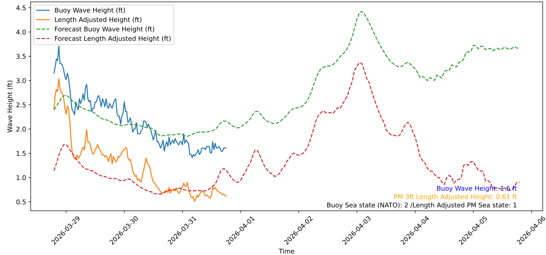
Wave Heights over Time for Green Beach at 2026-03-31 19:01:10
