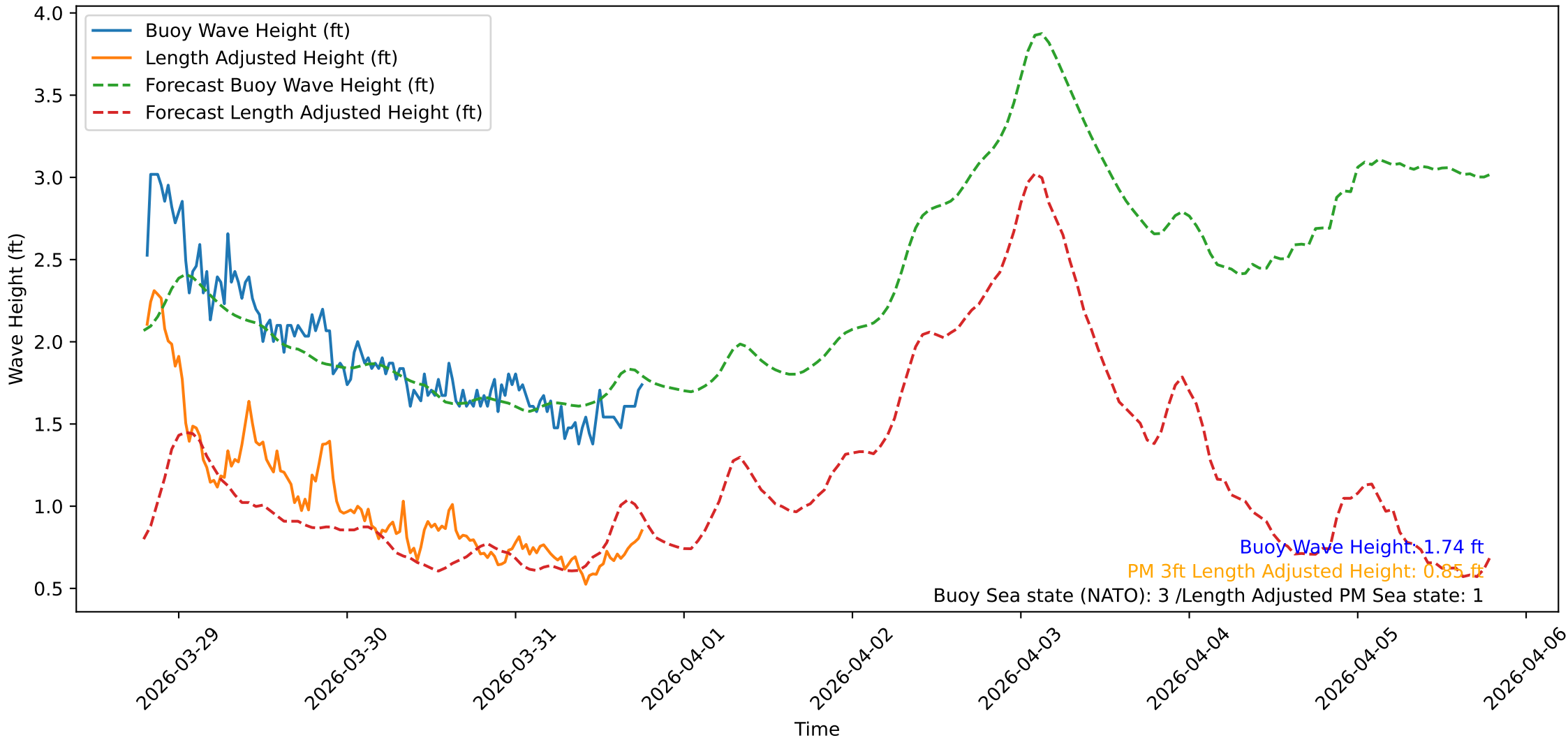
Wave Heights over Time for Red Beach at 2026-03-31 19:00:48
