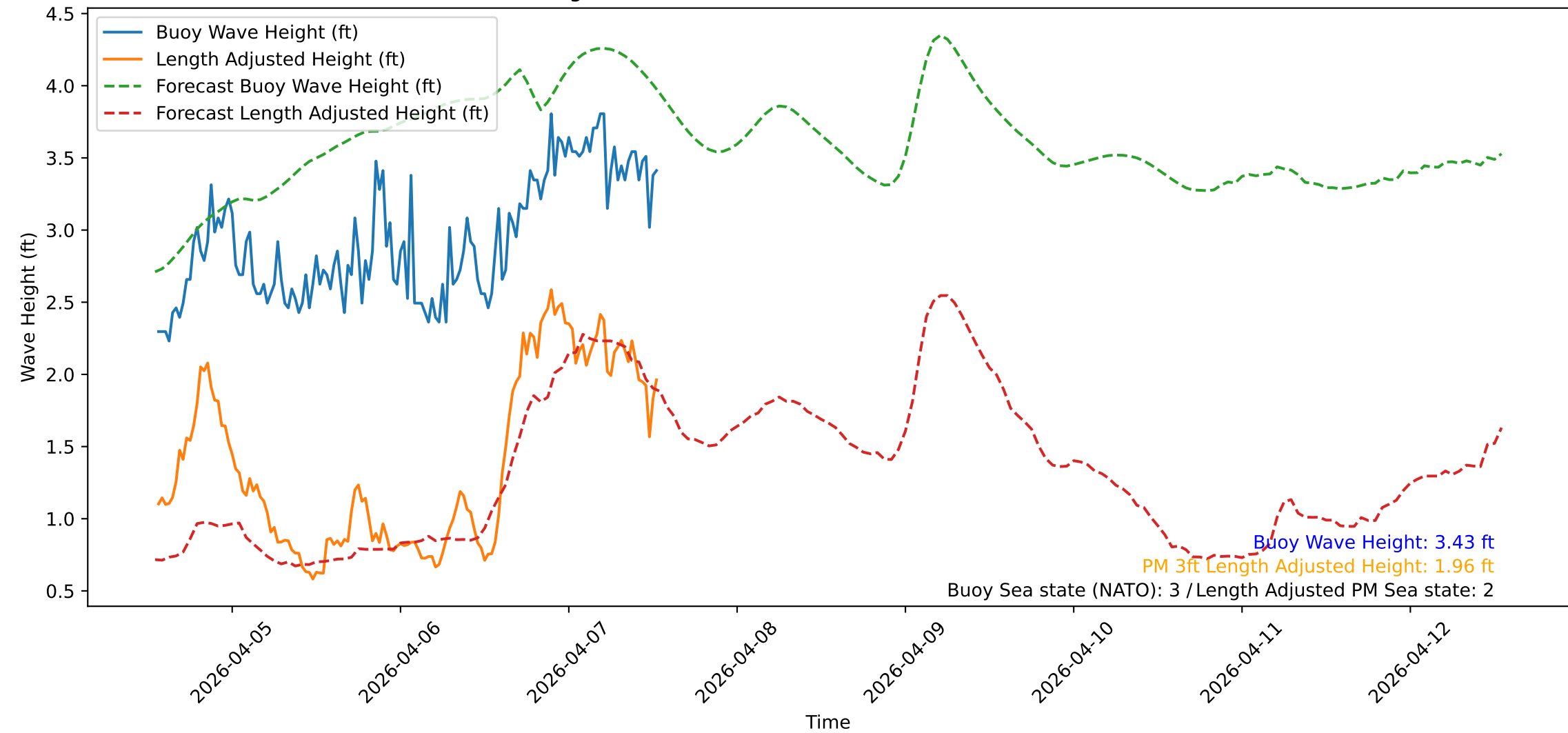
Wave Heights over Time for Green Beach at 2026-04-07 13:21:10
