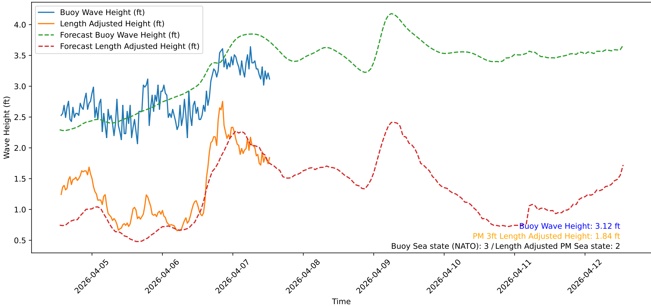
Wave Heights over Time for Oceanside Harbor at 2026-04-07 13:20:31
