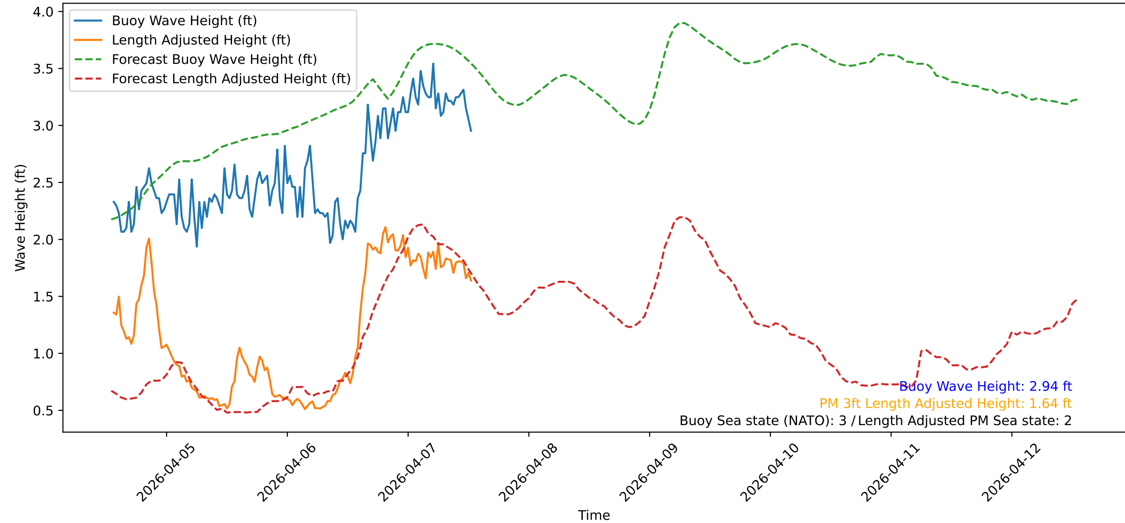
Wave Heights over Time for Red Beach at 2026-04-07 13:20:47
