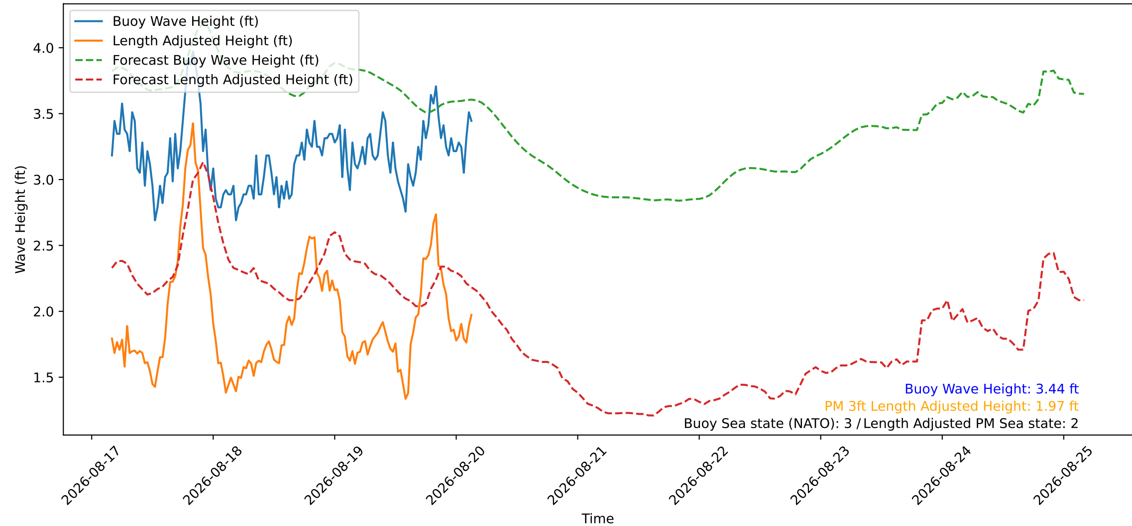
Wave Heights over Time for Green Beach at 2026-08-20 03:51:10
