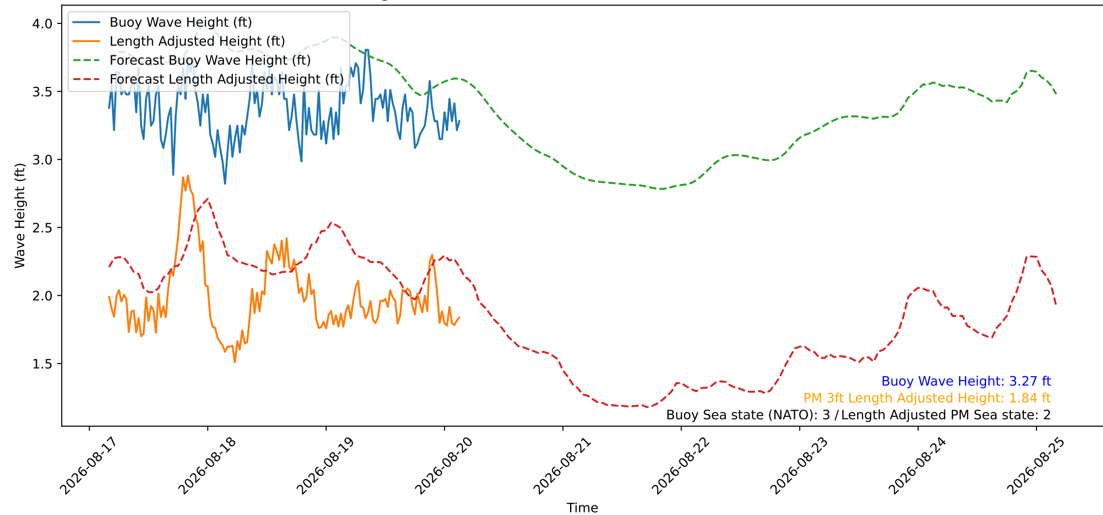
Wave Heights over Time for Oceanside Harbor at 2026-08-20 03:50:26
