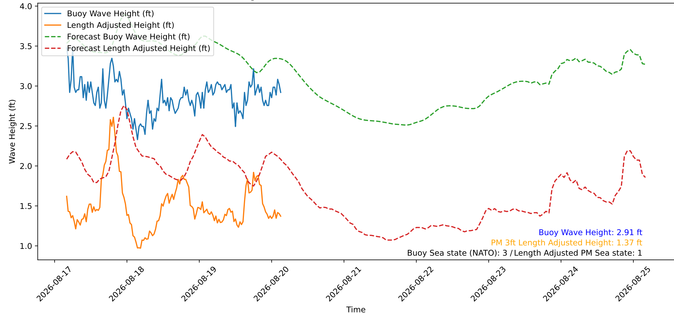
Wave Heights over Time for Red Beach at 2026-08-20 03:50:46
