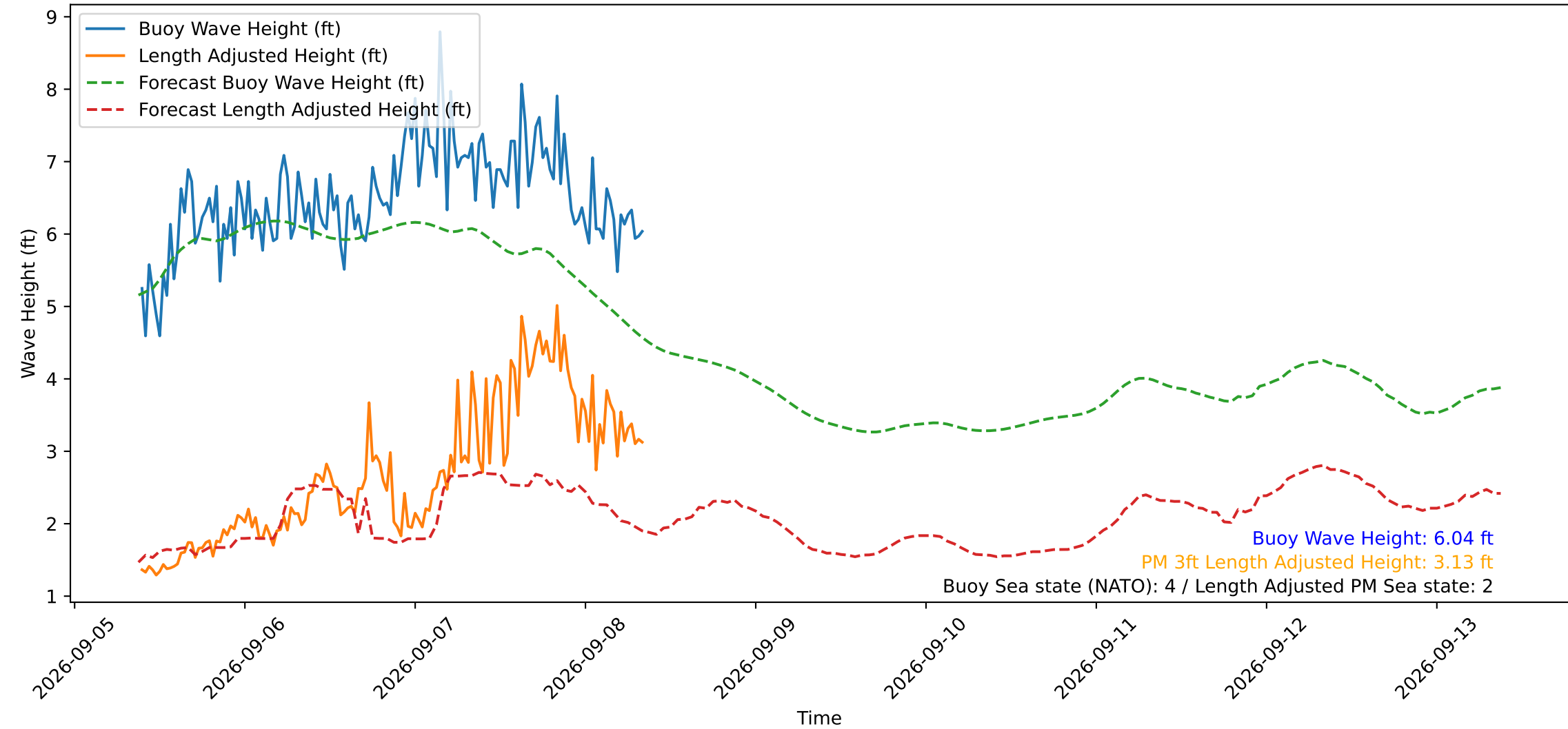
Wave Heights over Time for Green Beach at 2026-09-08 09:01:13
