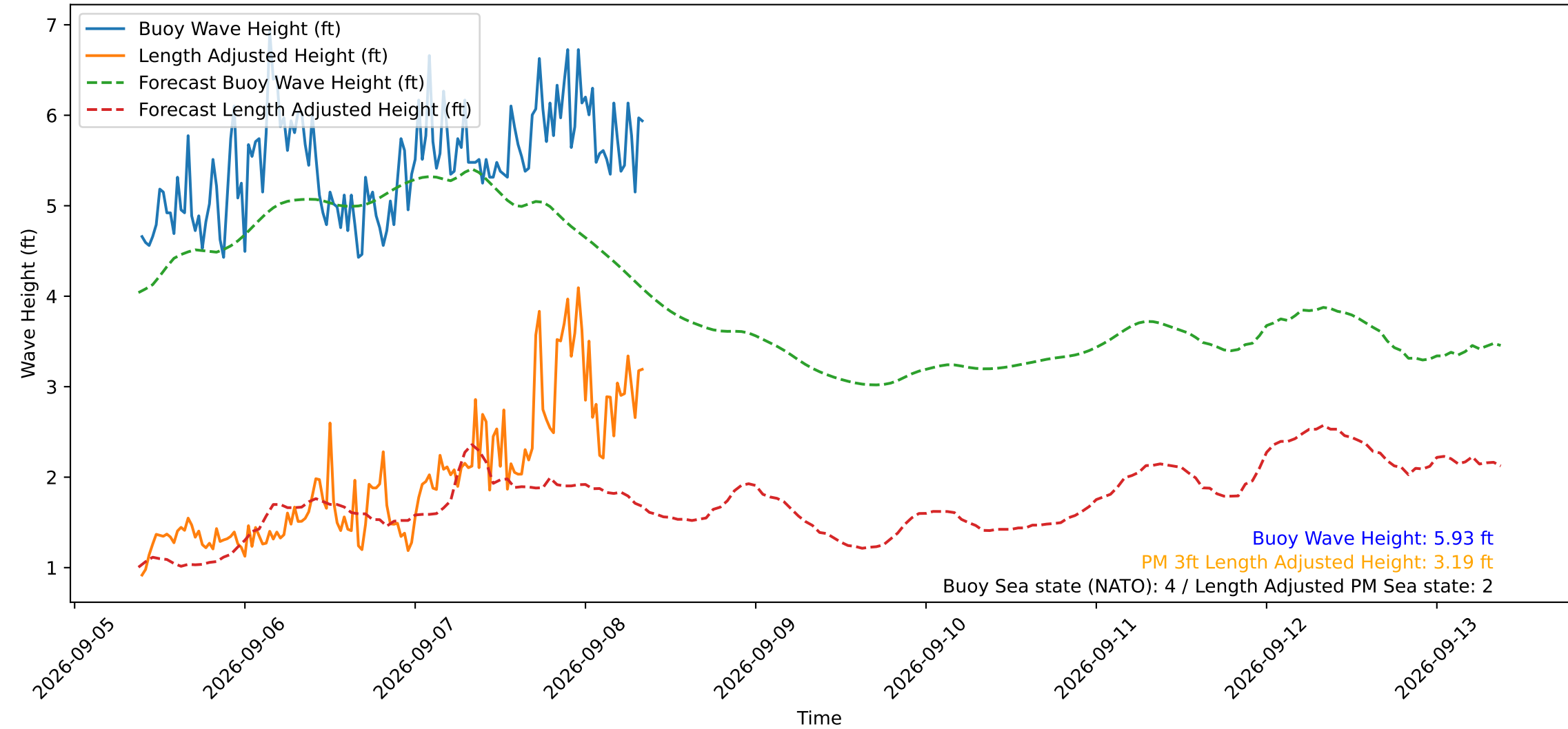
Wave Heights over Time for Red Beach at 2026-09-08 09:00:50
