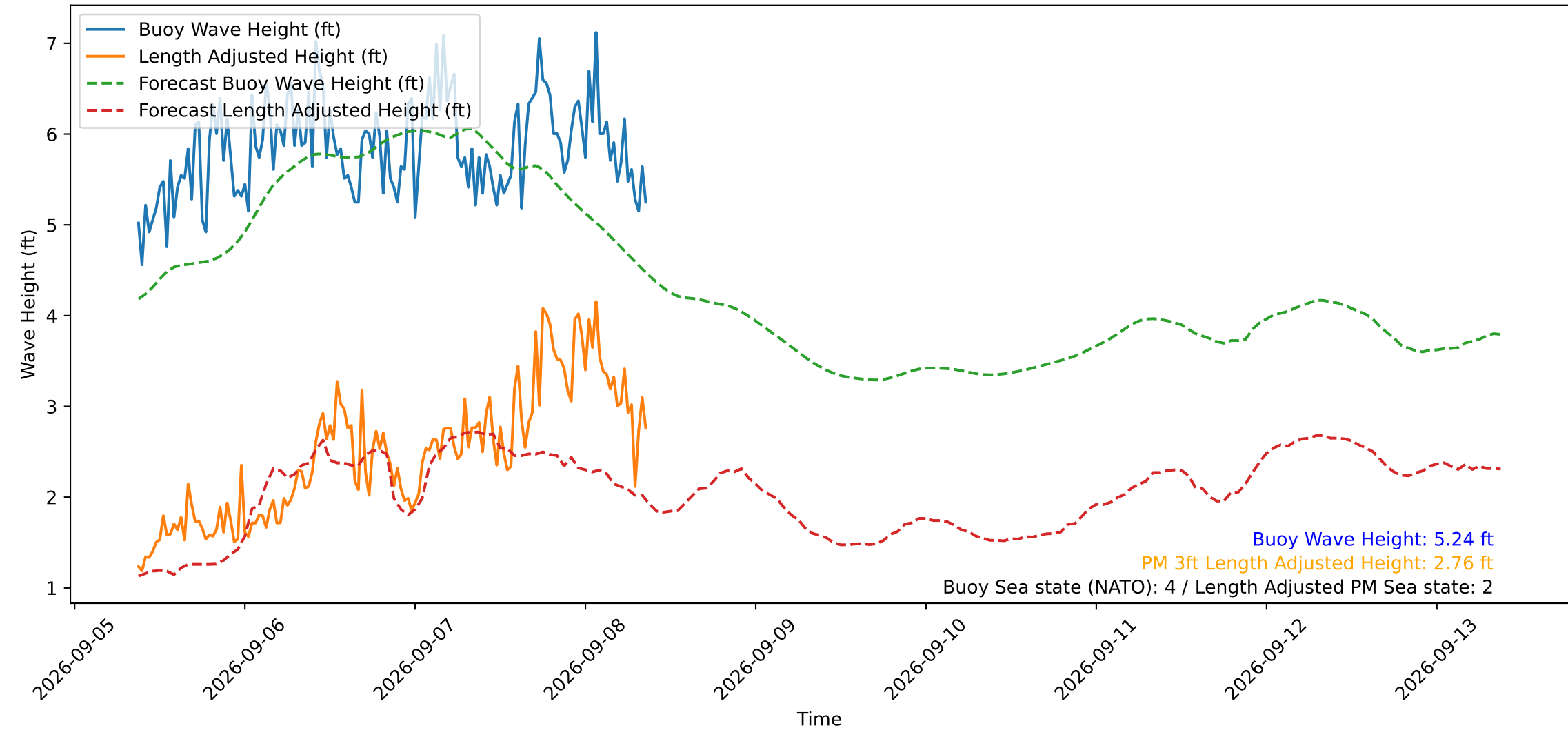
Wave Heights over Time for Oceanside Harbor at 2026-09-08 09:00:30
