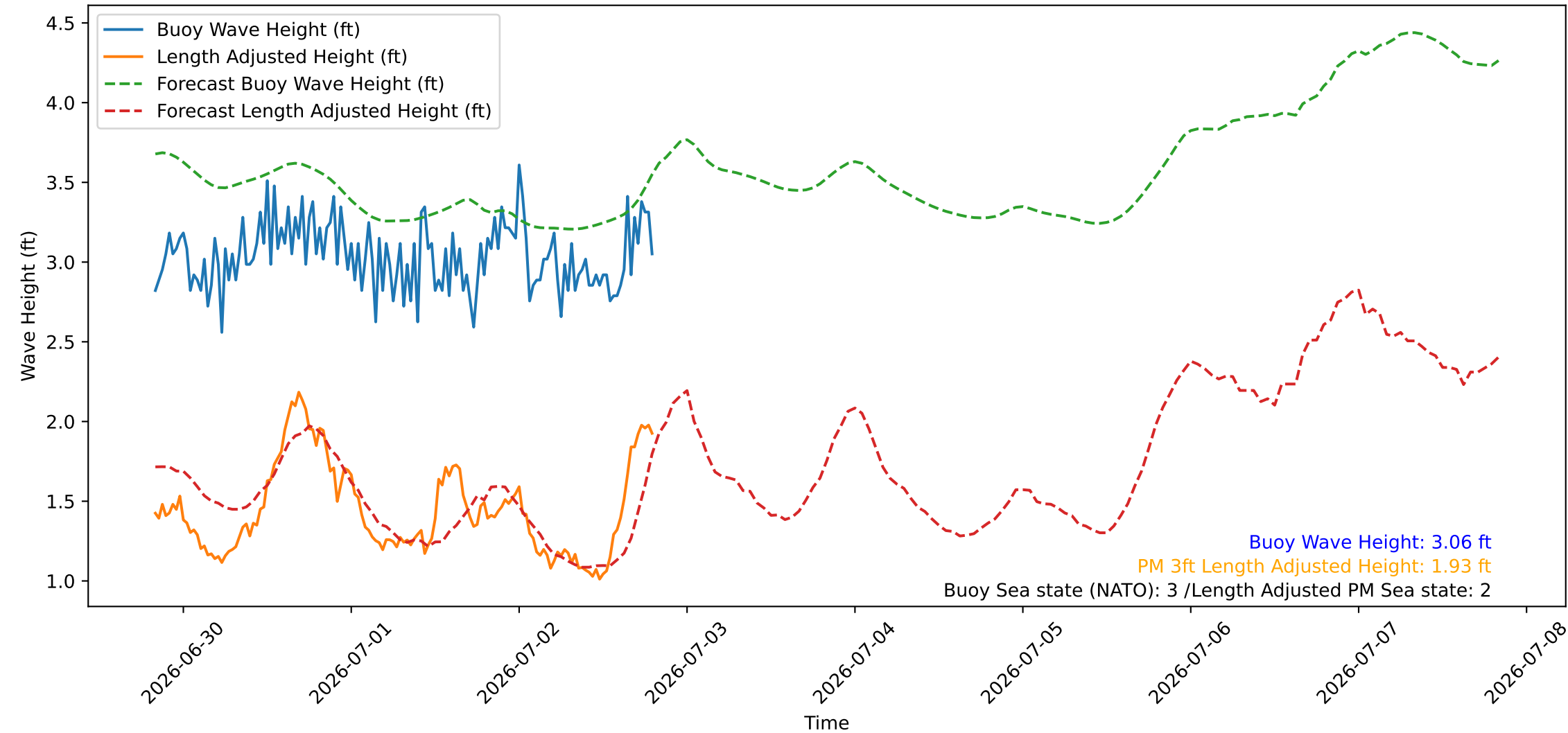
Wave Heights over Time for Oceanside Harbor at 2026-07-02 20:00:27
