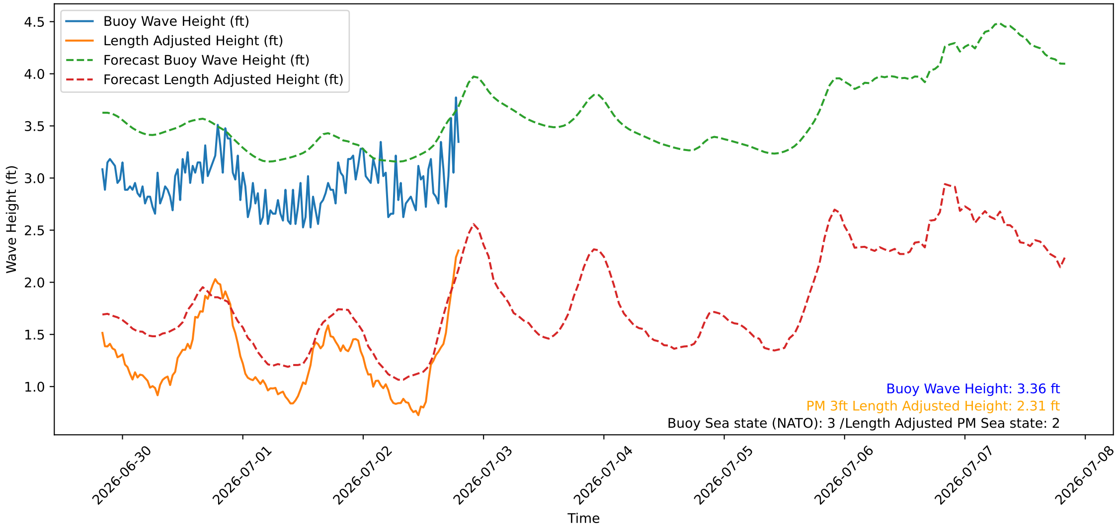
Wave Heights over Time for Green Beach at 2026-07-02 20:01:08
