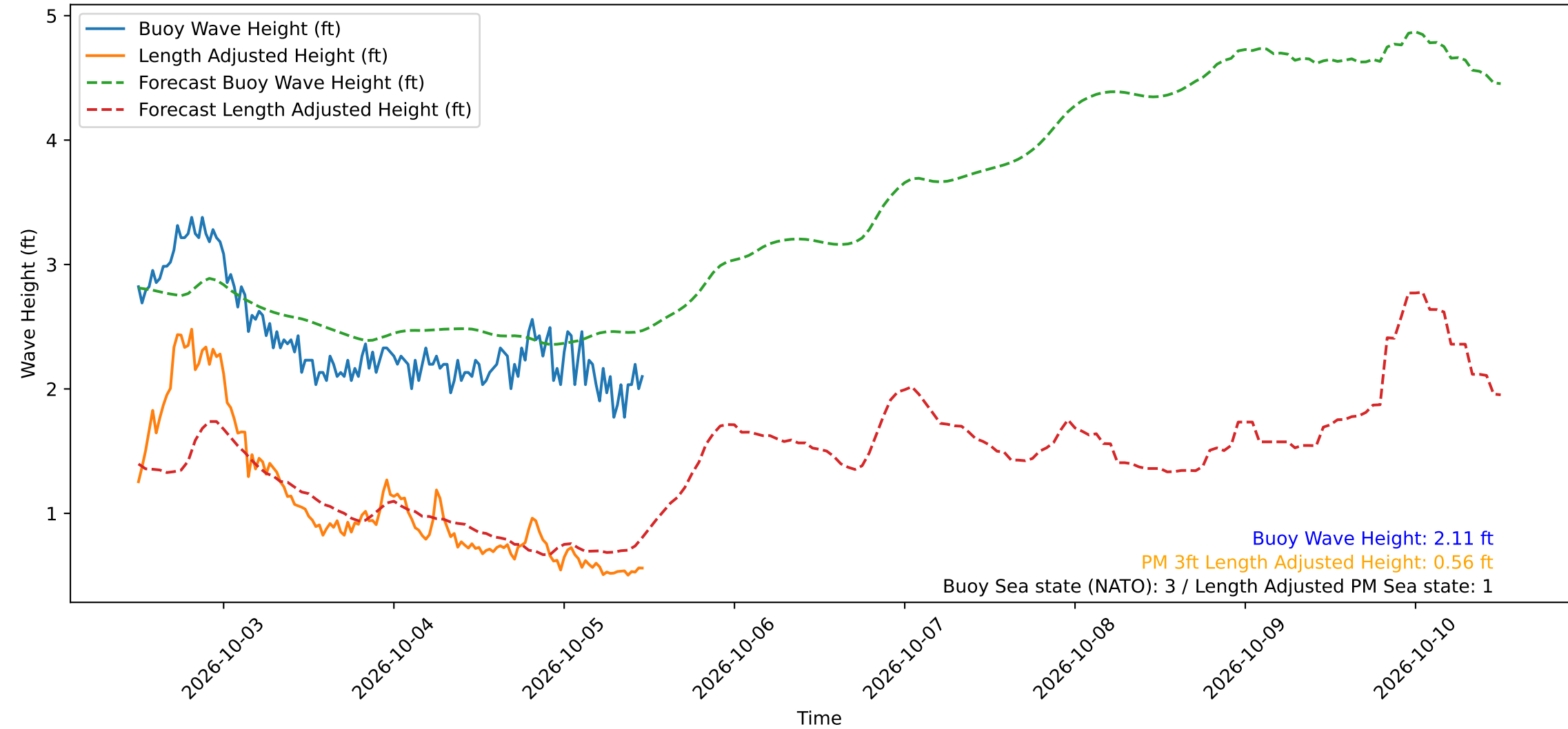
Wave Heights over Time for Green Beach at 2026-10-05 11:51:14
