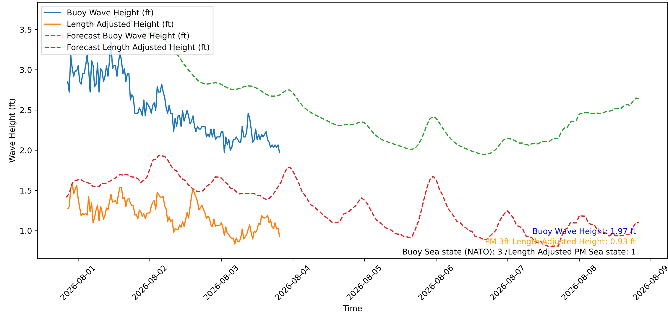
Wave Heights over Time for Red Beach at 2026-08-03 20:20:46
