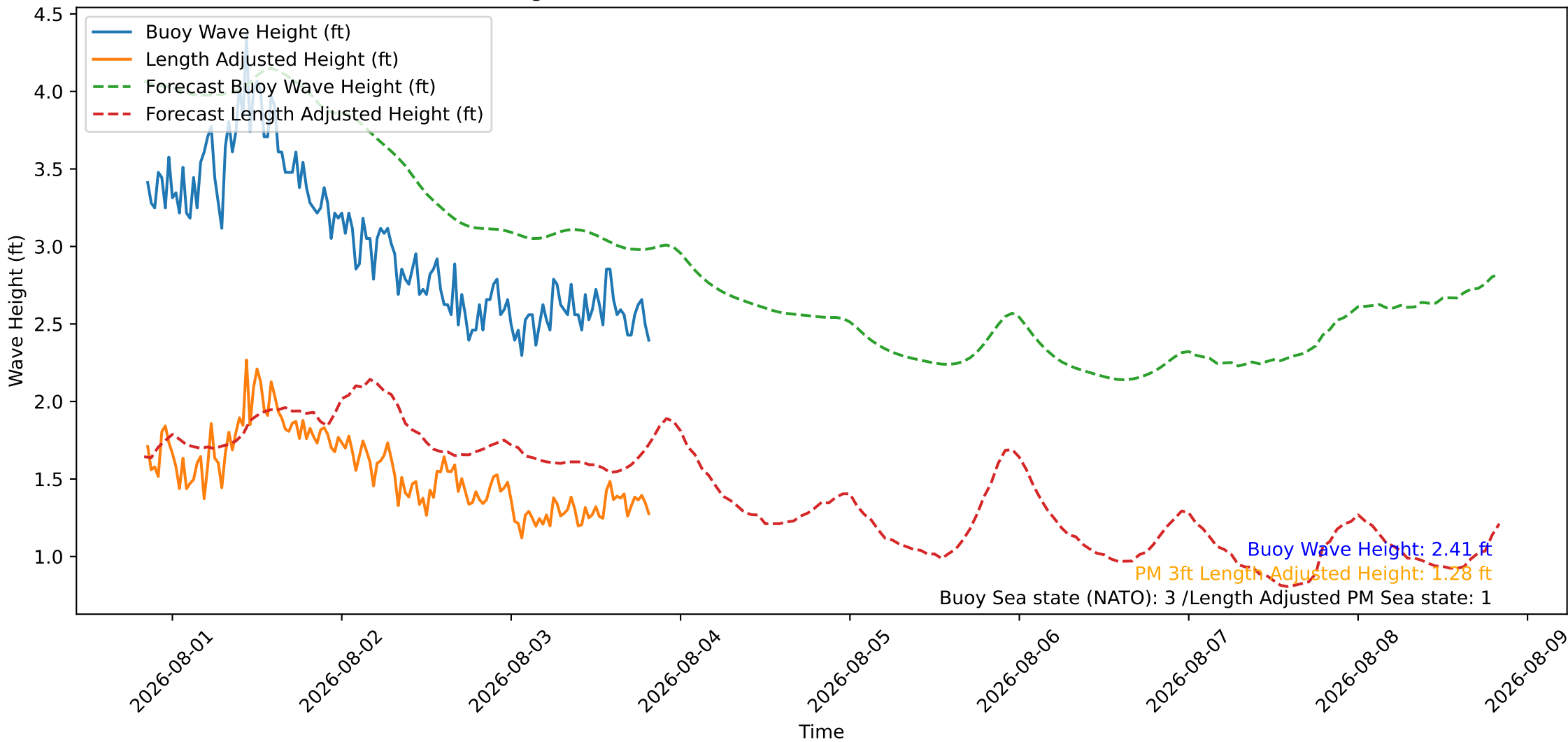
Wave Heights over Time for Oceanside Harbor at 2026-08-03 20:20:26
