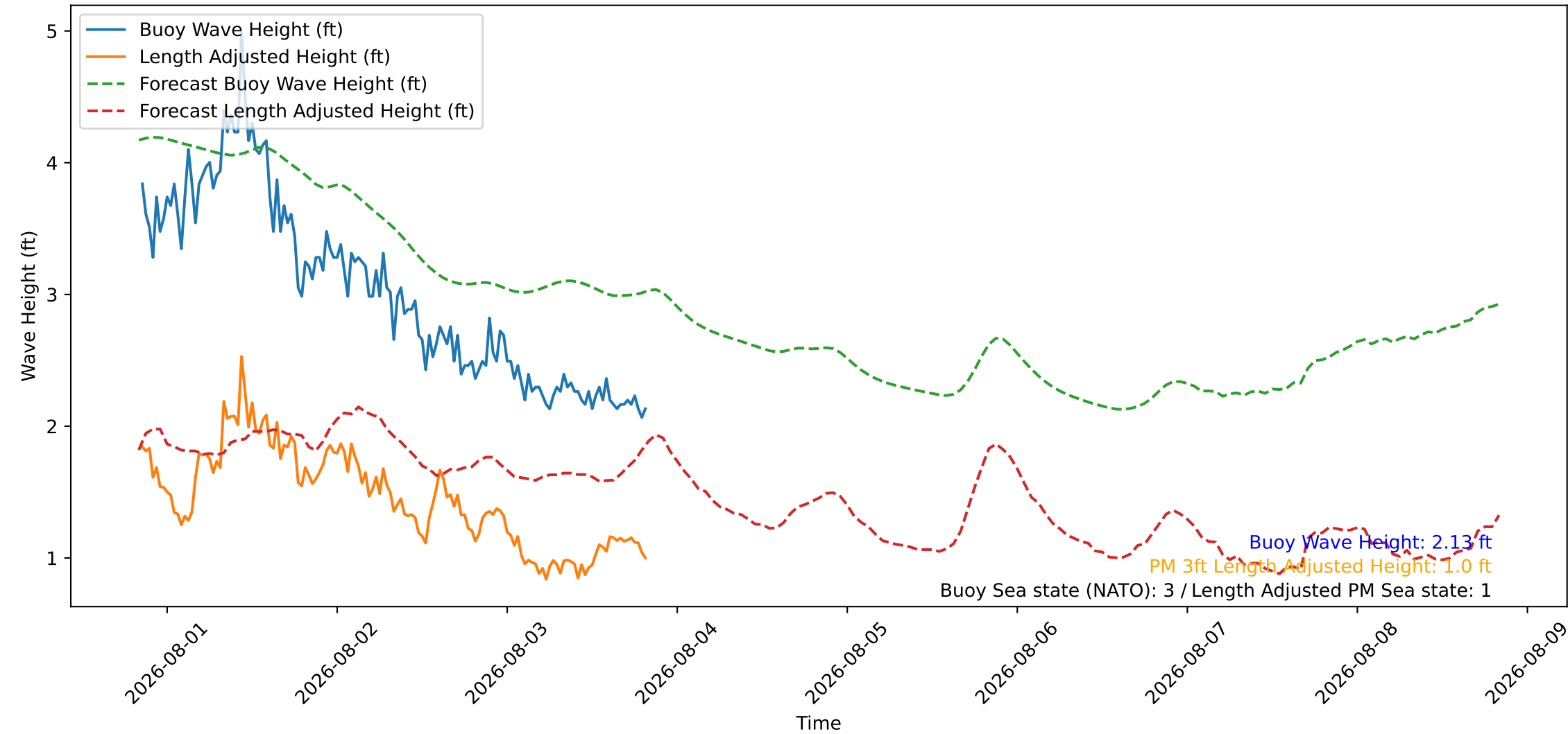
Wave Heights over Time for Green Beach at 2026-08-03 20:21:09
