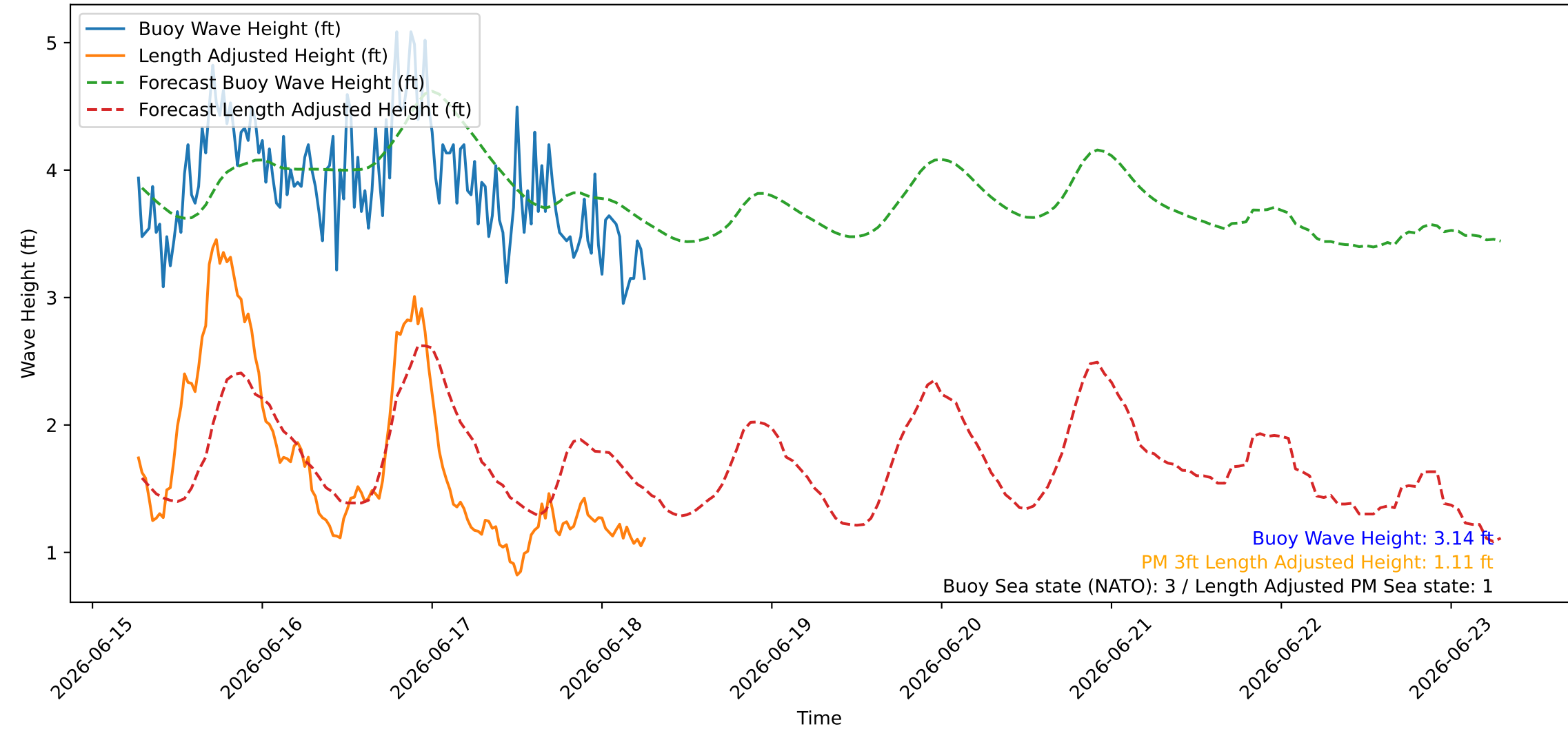
Wave Heights over Time for Green Beach at 2026-06-18 06:41:09
