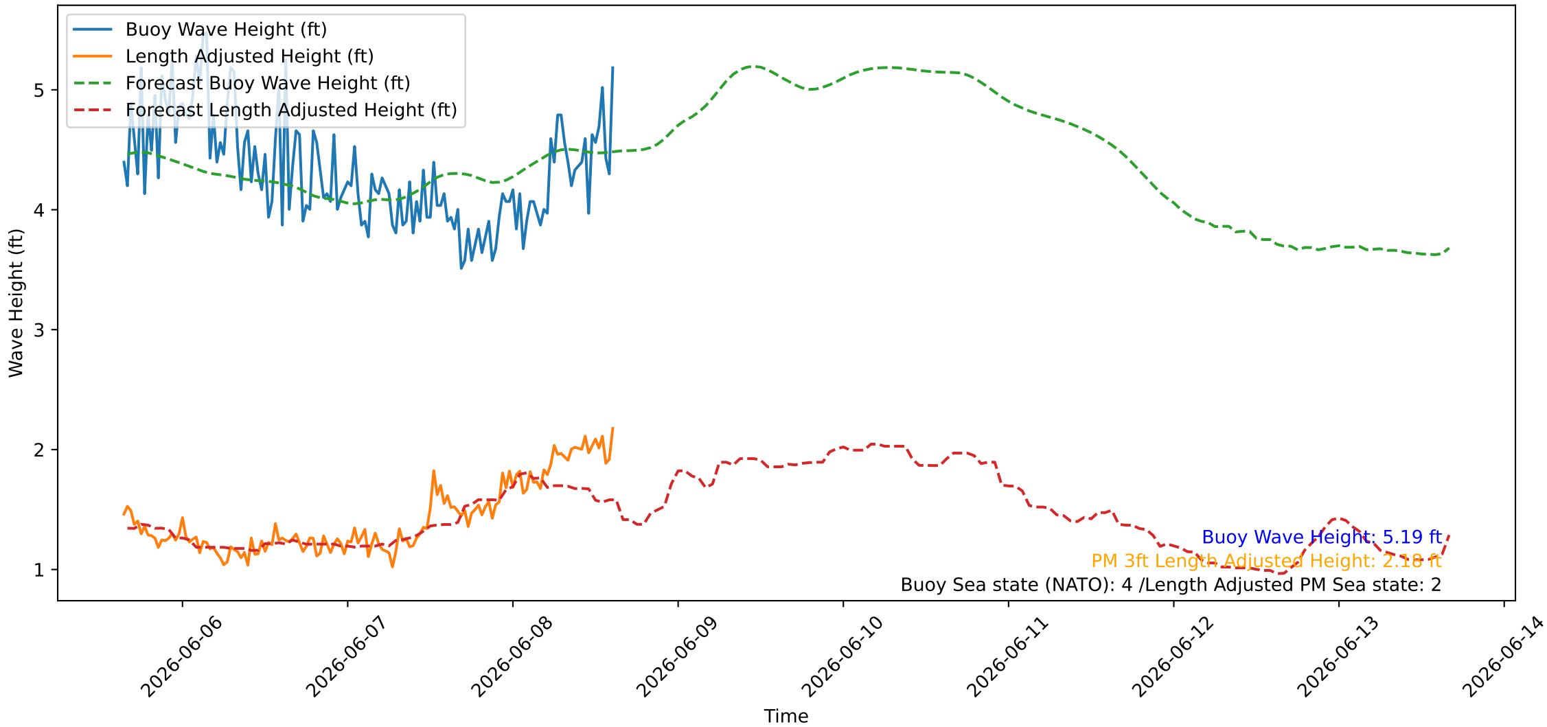
Wave Heights over Time for Oceanside Harbor at 2026-06-08 15:30:26
