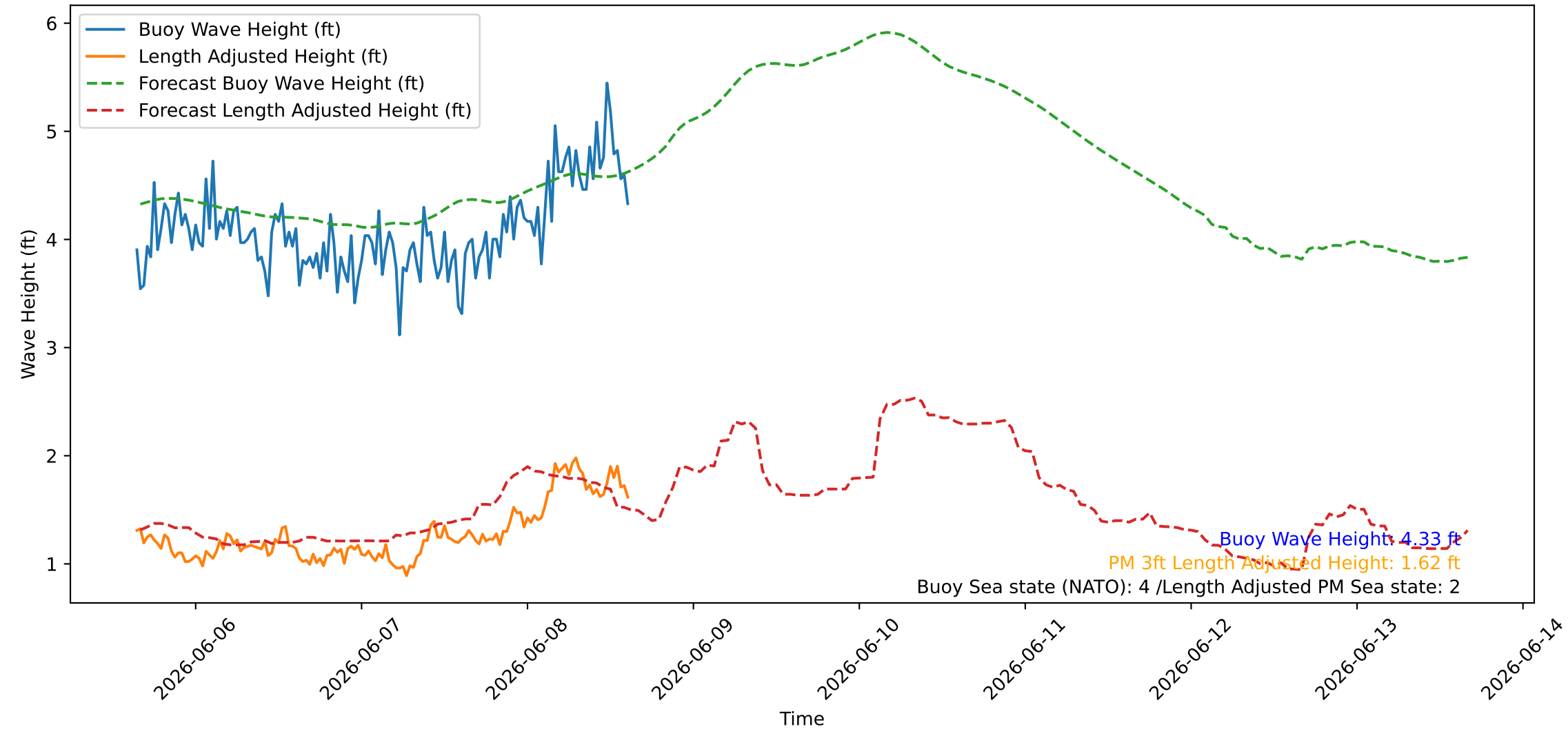
Wave Heights over Time for Green Beach at 2026-06-08 15:31:08
