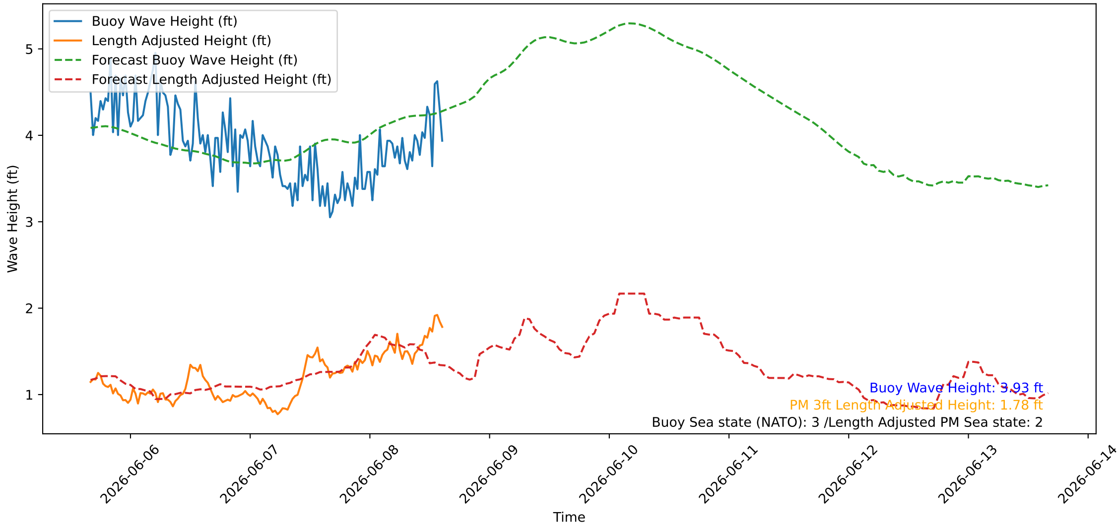
Wave Heights over Time for Red Beach at 2026-06-08 15:30:45
