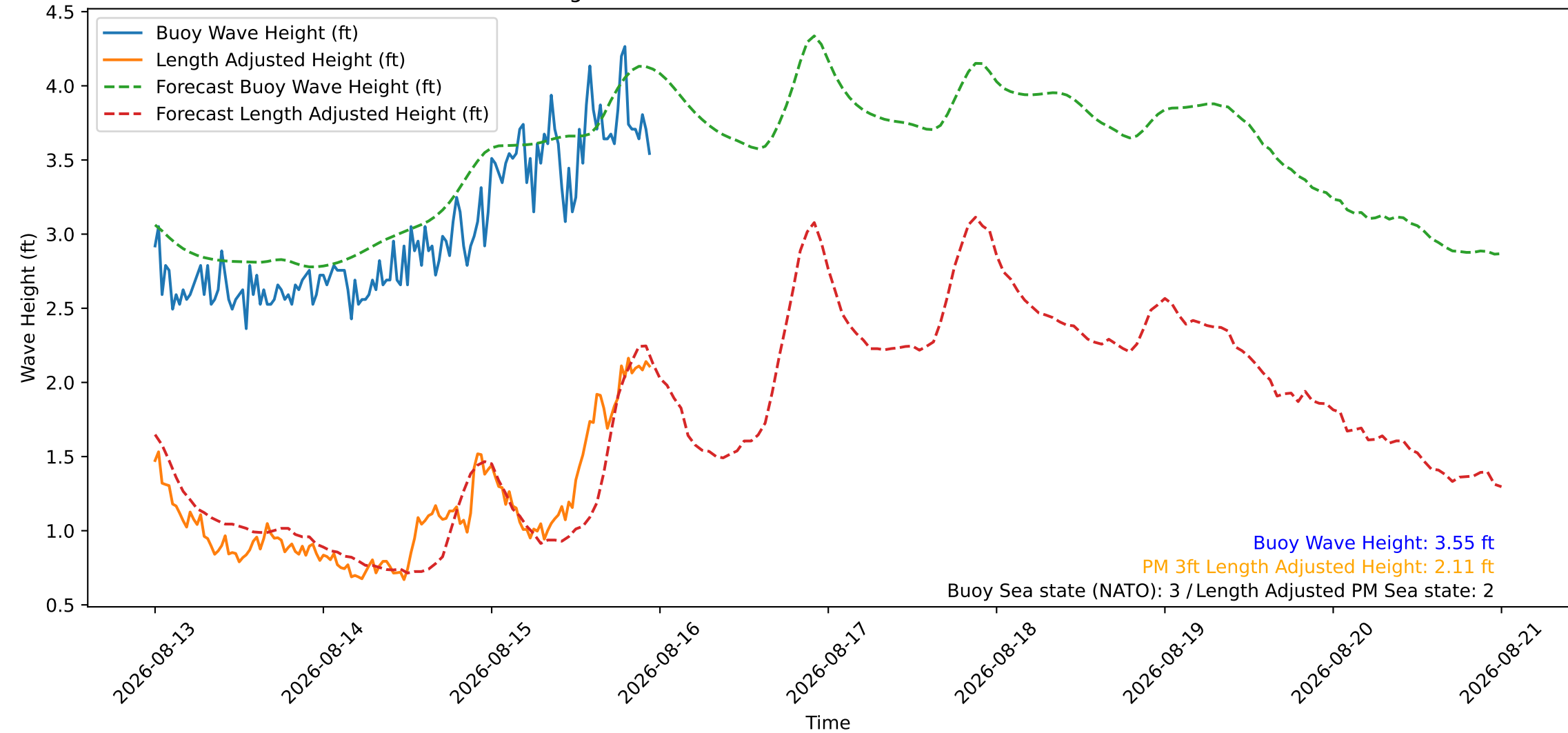
Wave Heights over Time for Green Beach at 2026-08-15 23:31:08
