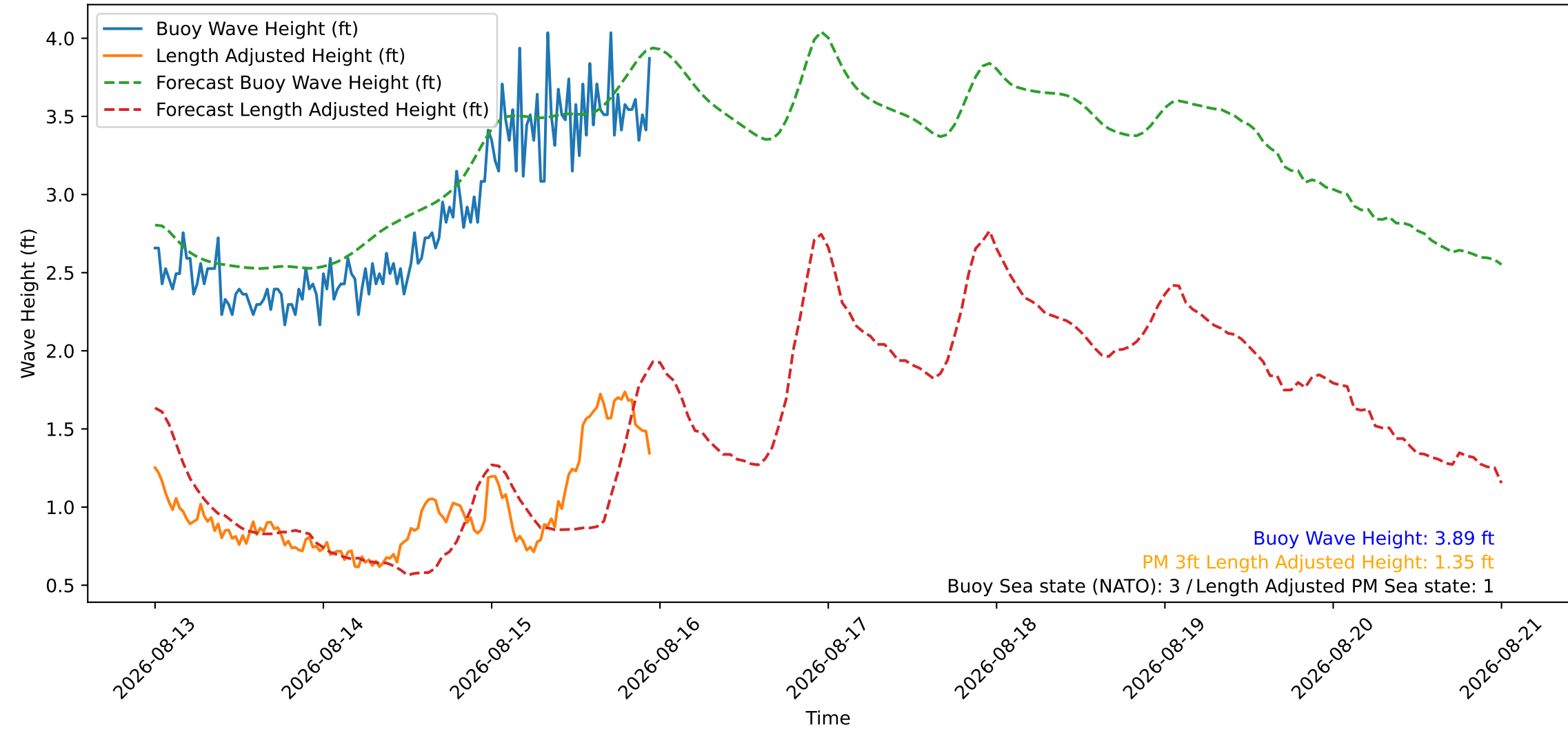
Wave Heights over Time for Red Beach at 2026-08-15 23:30:46
