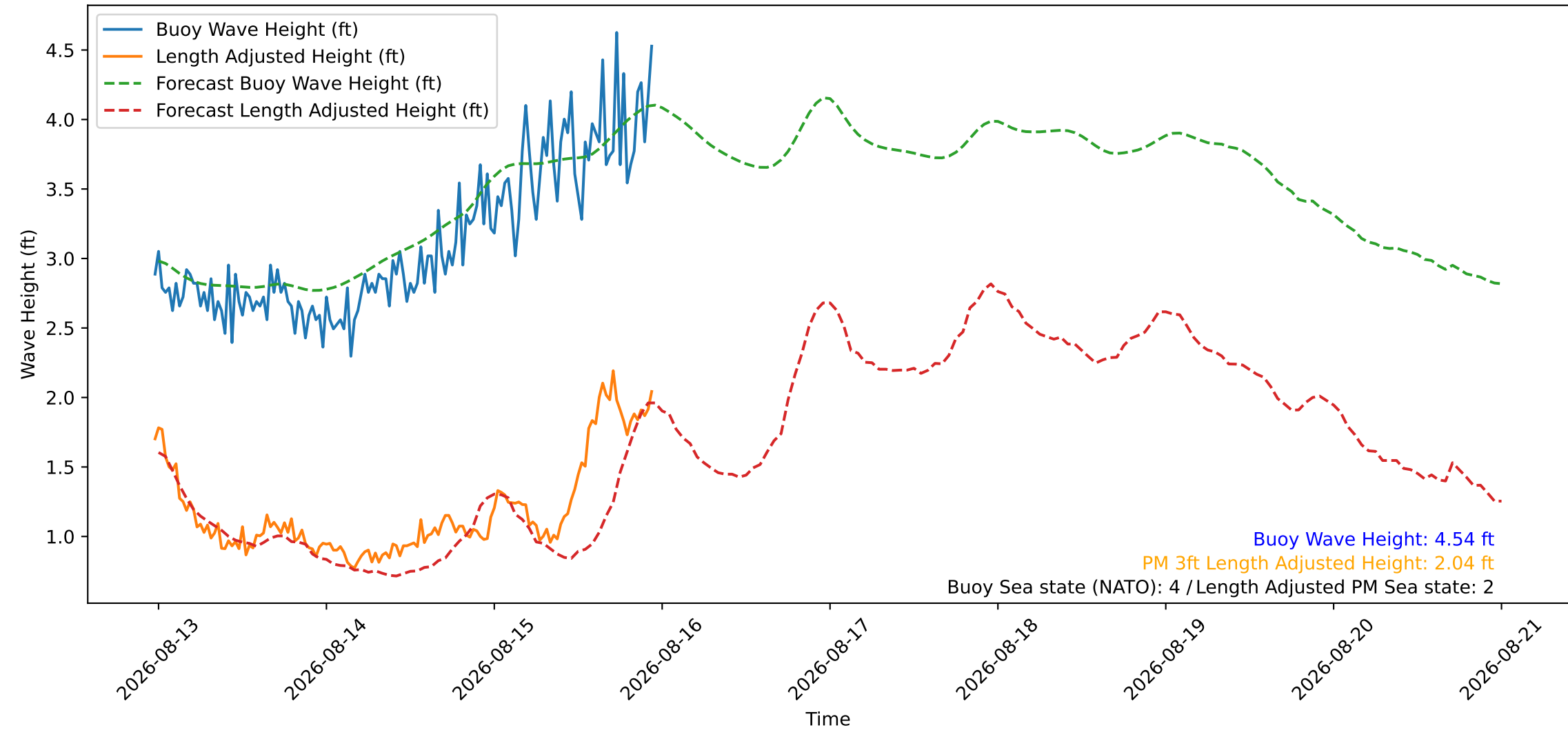
Wave Heights over Time for Oceanside Harbor at 2026-08-15 23:30:26
