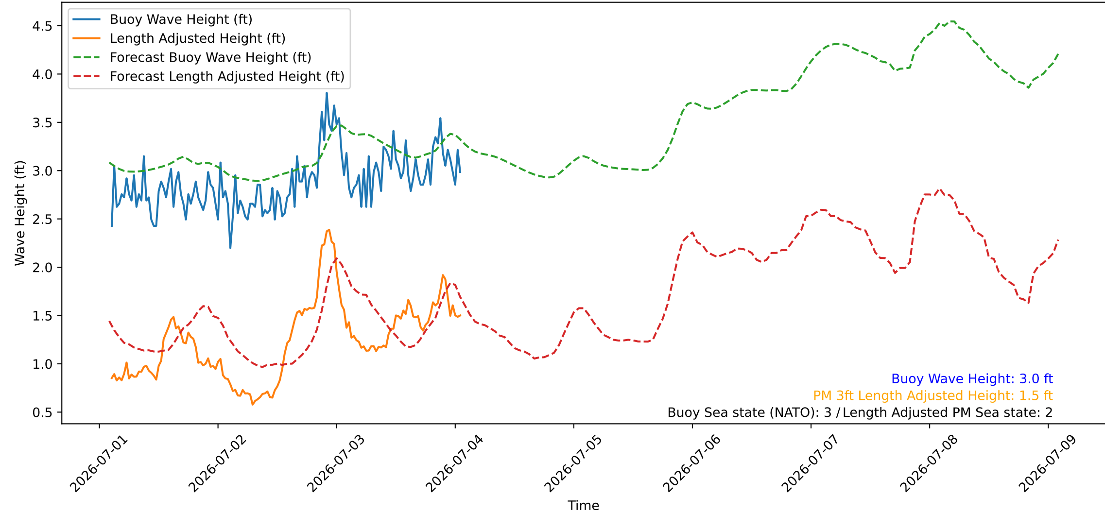
Wave Heights over Time for Red Beach at 2026-07-04 02:00:45
