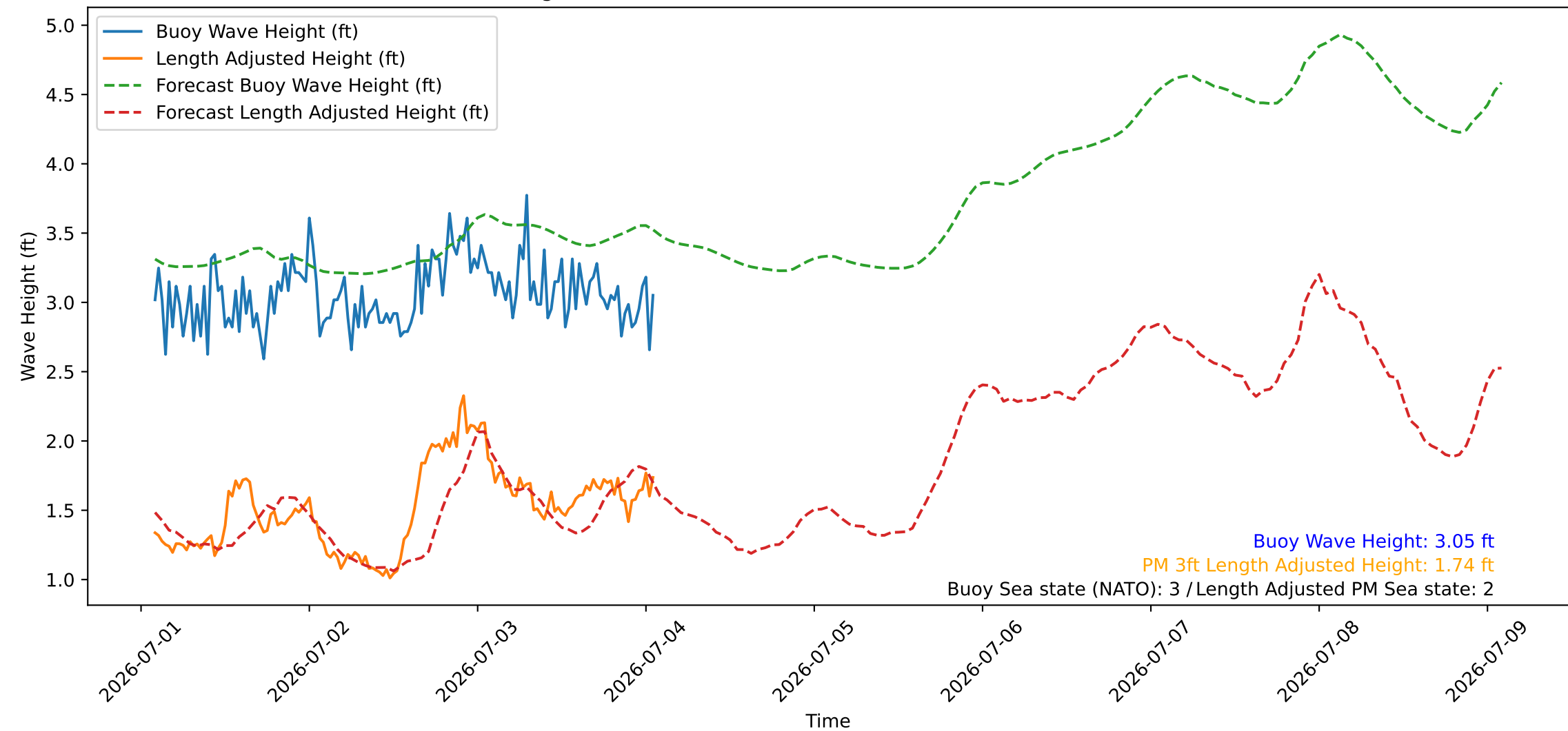
Wave Heights over Time for Oceanside Harbor at 2026-07-04 02:00:26
