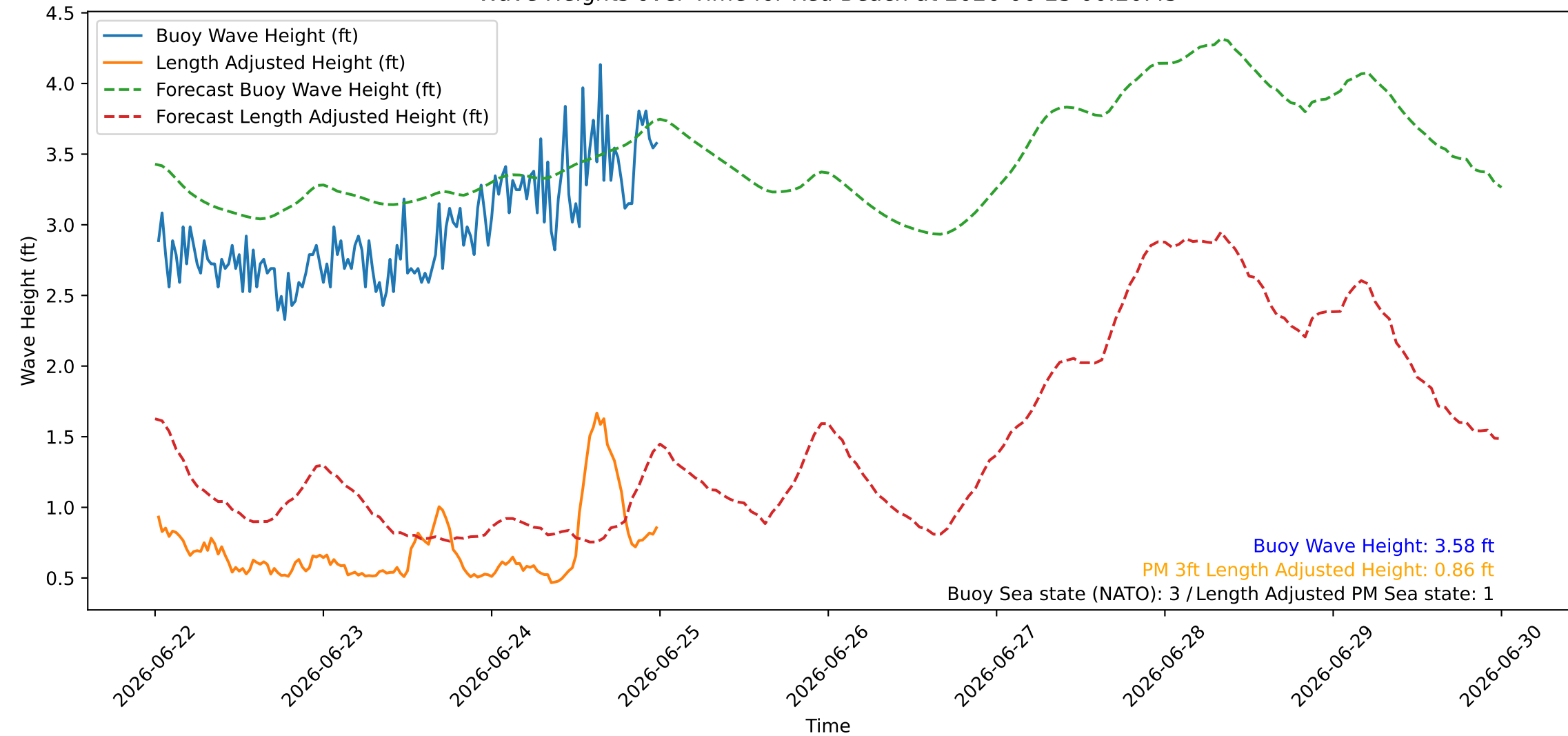
Wave Heights over Time for Red Beach at 2026-06-25 00:20:45
