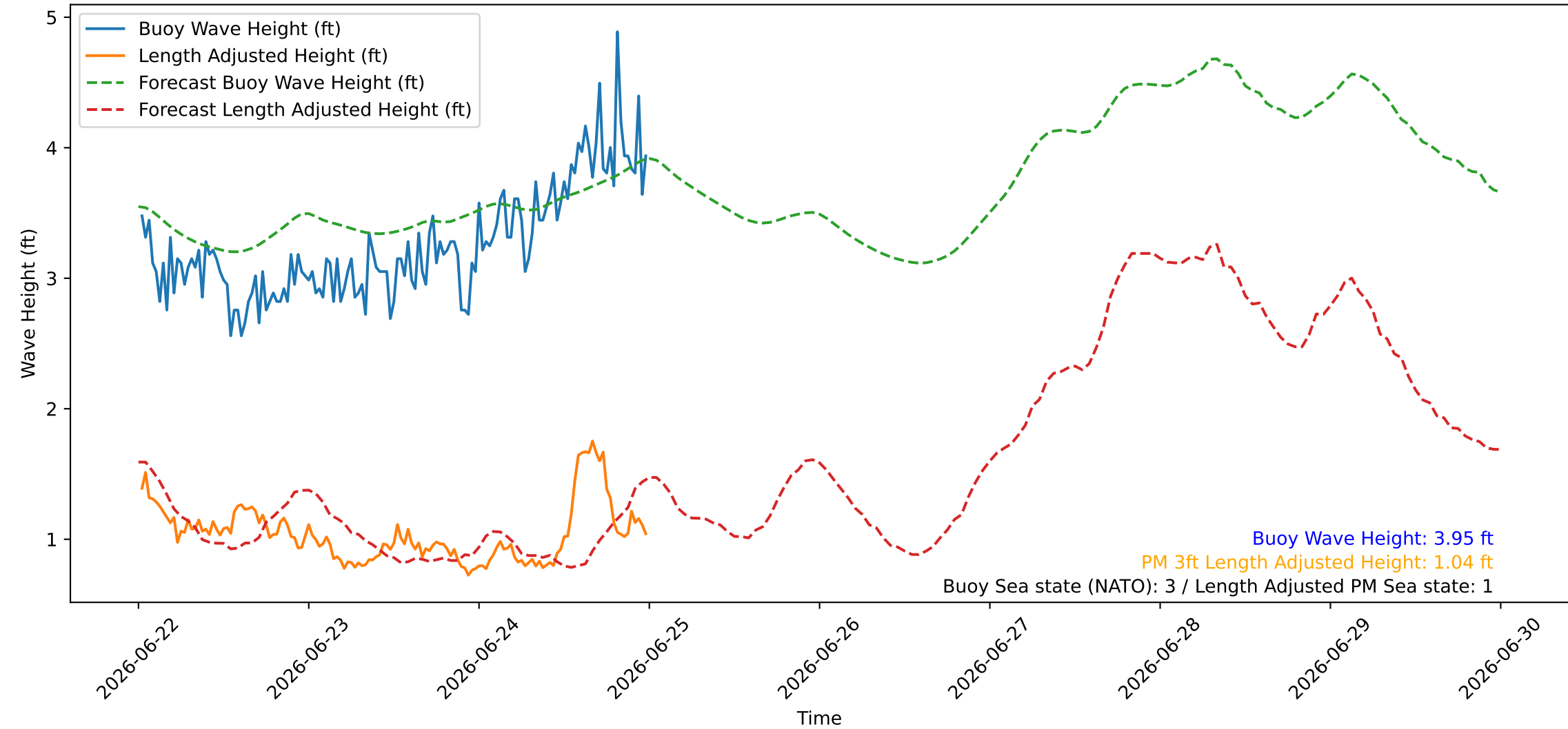
Wave Heights over Time for Oceanside Harbor at 2026-06-25 00:20:25
