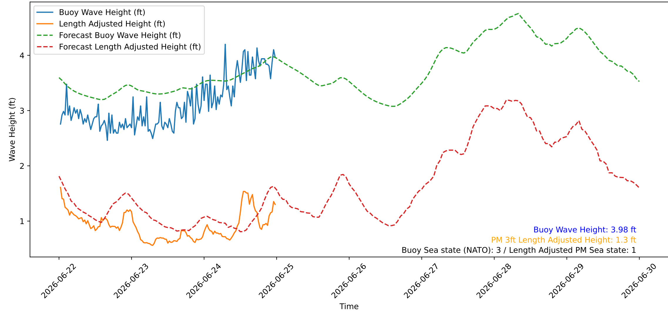
Wave Heights over Time for Green Beach at 2026-06-25 00:21:08
