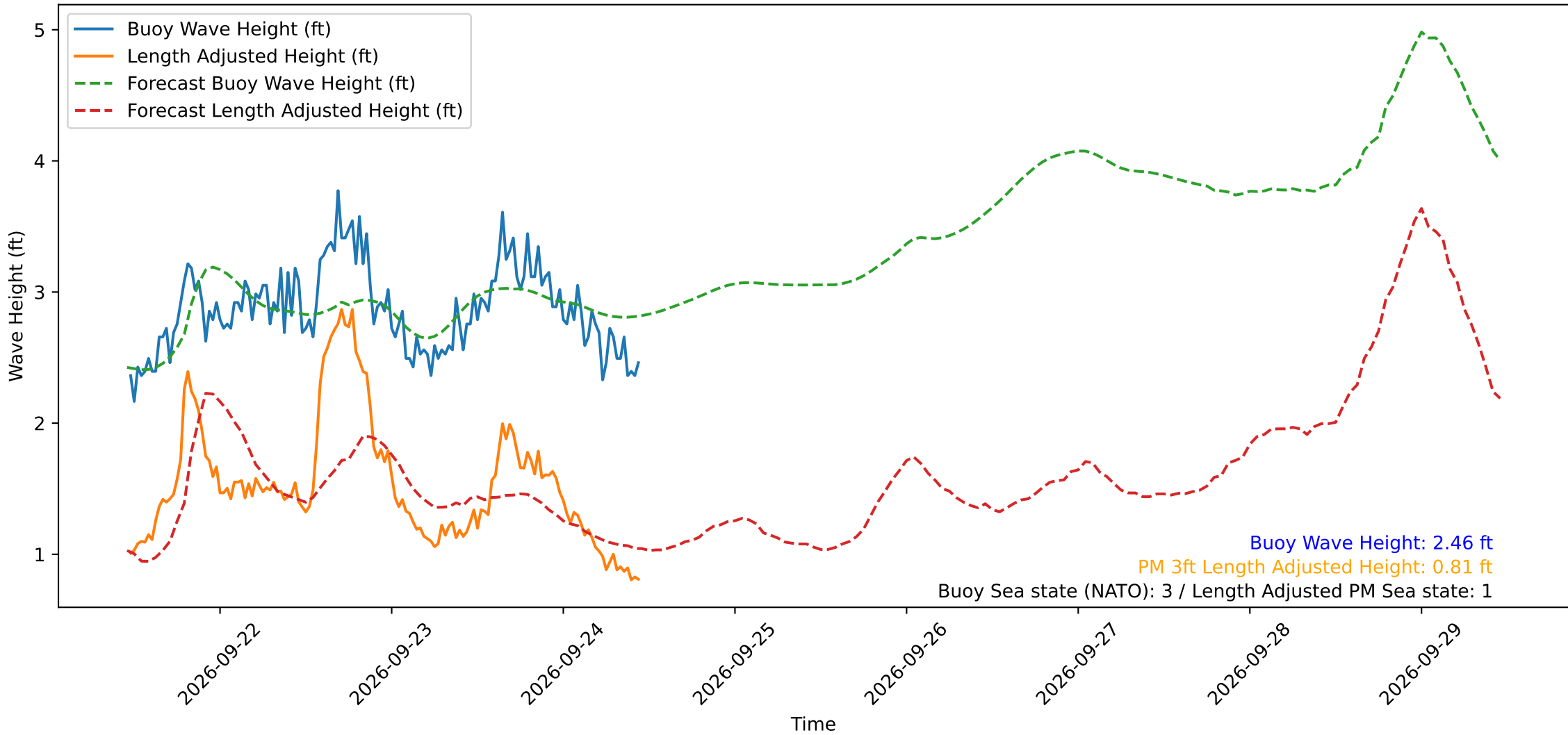
Wave Heights over Time for Oceanside Harbor at 2026-09-24 11:20:29
