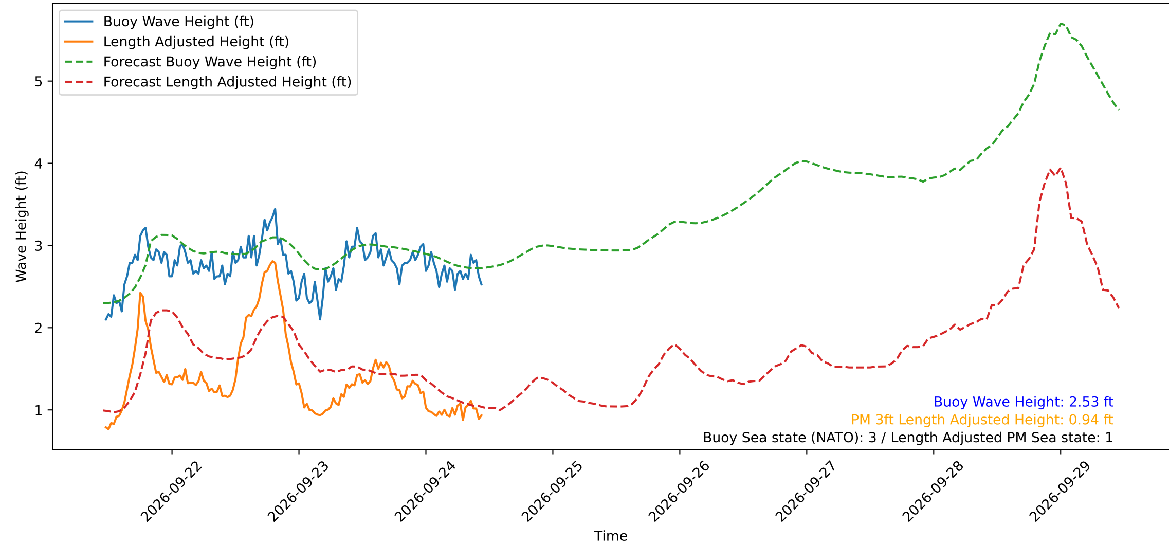
Wave Heights over Time for Green Beach at 2026-09-24 11:21:14
