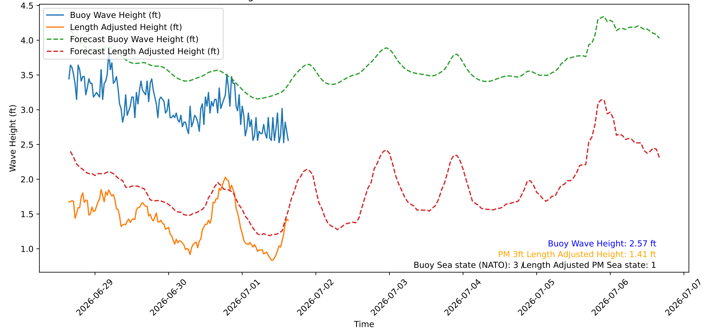
Wave Heights over Time for Green Beach at 2026-07-01 15:41:08
