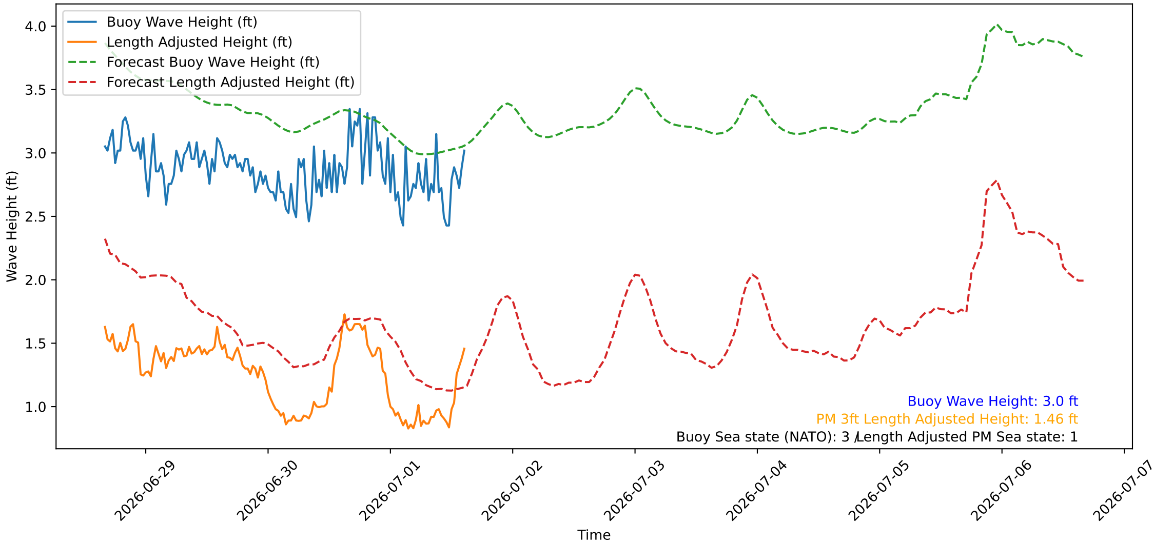
Wave Heights over Time for Red Beach at 2026-07-01 15:40:45
