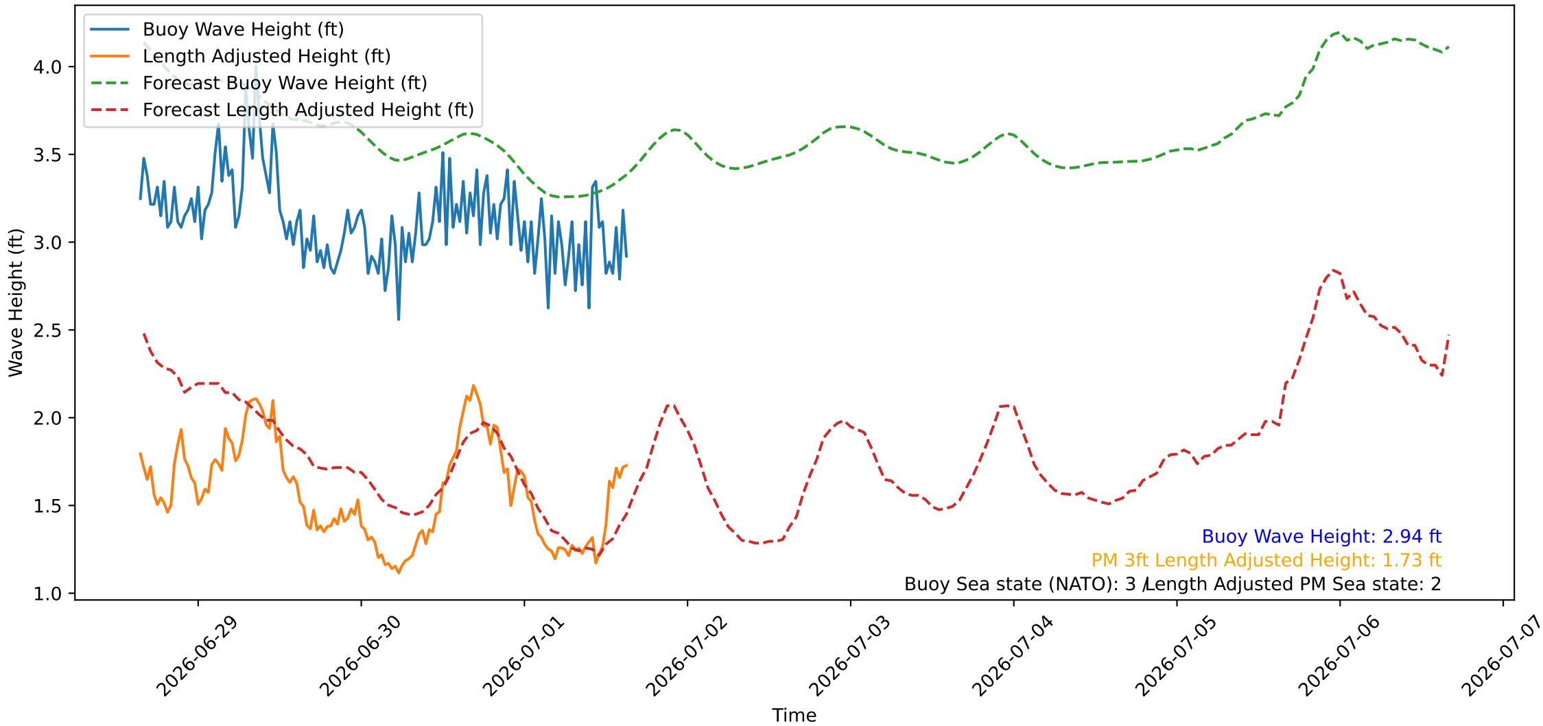
Wave Heights over Time for Oceanside Harbor at 2026-07-01 15:40:26
