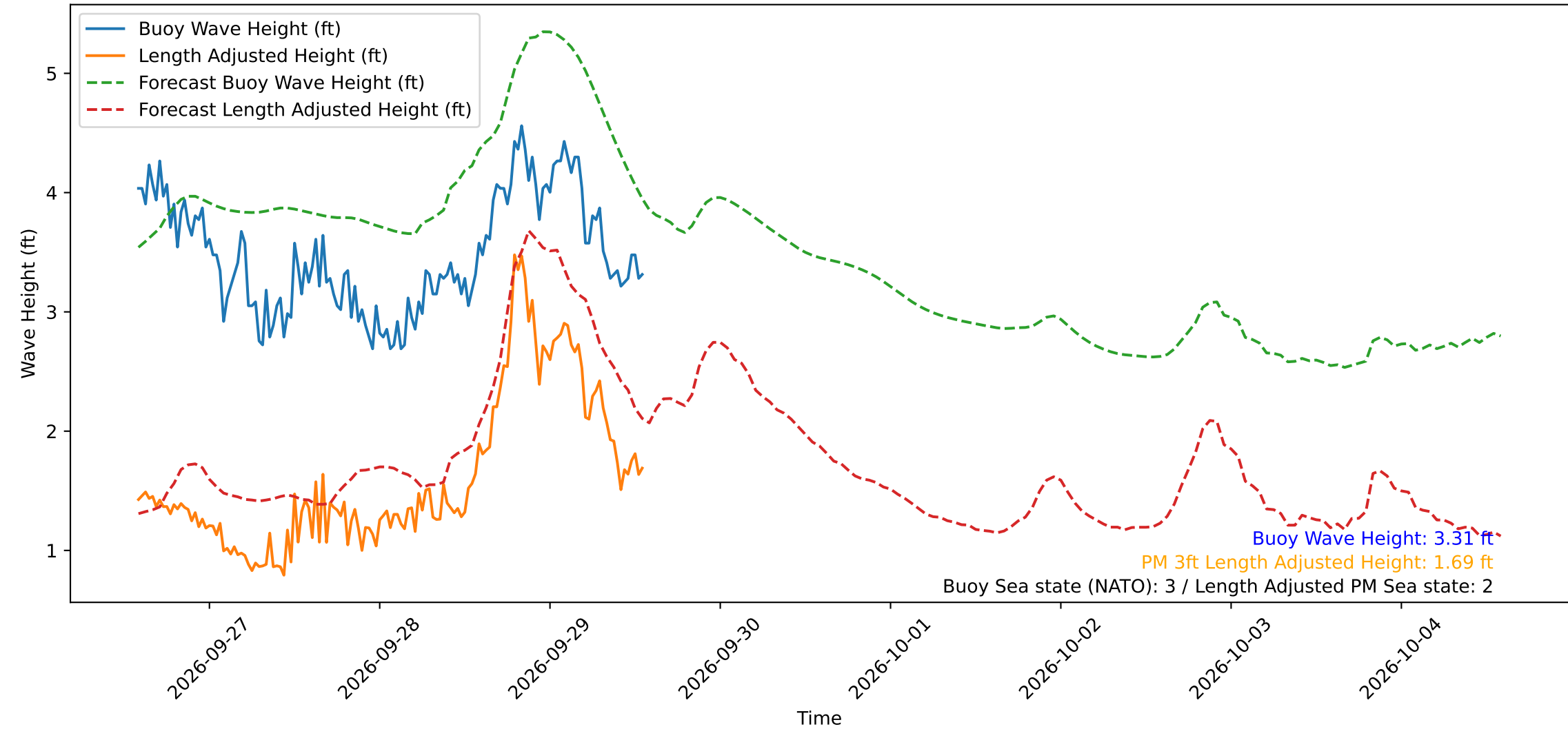
Wave Heights over Time for Green Beach at 2026-09-29 13:41:14
