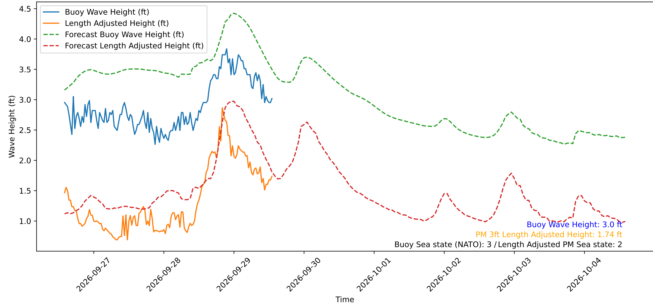
Wave Heights over Time for Red Beach at 2026-09-29 13:40:51
