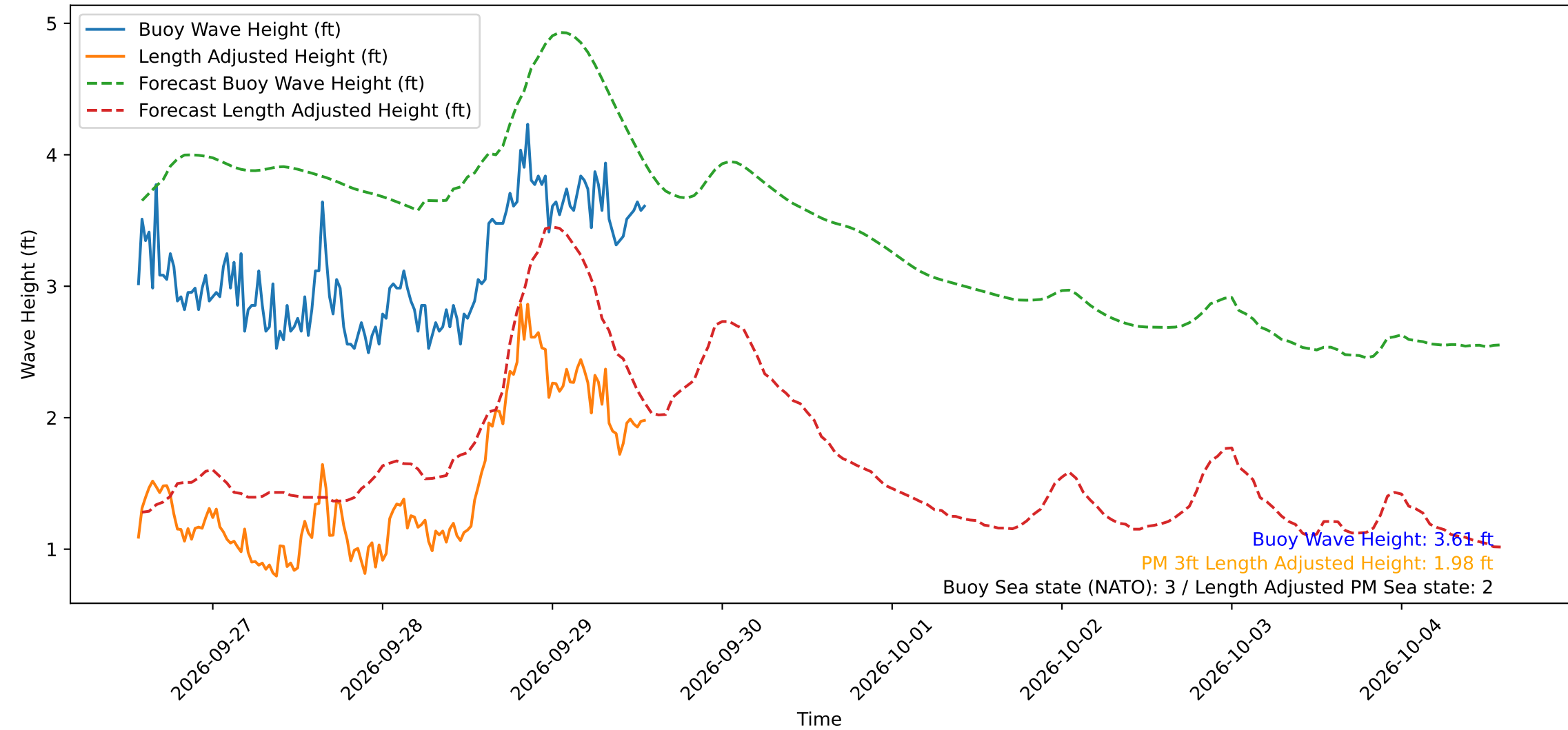
Wave Heights over Time for Oceanside Harbor at 2026-09-29 13:40:31
