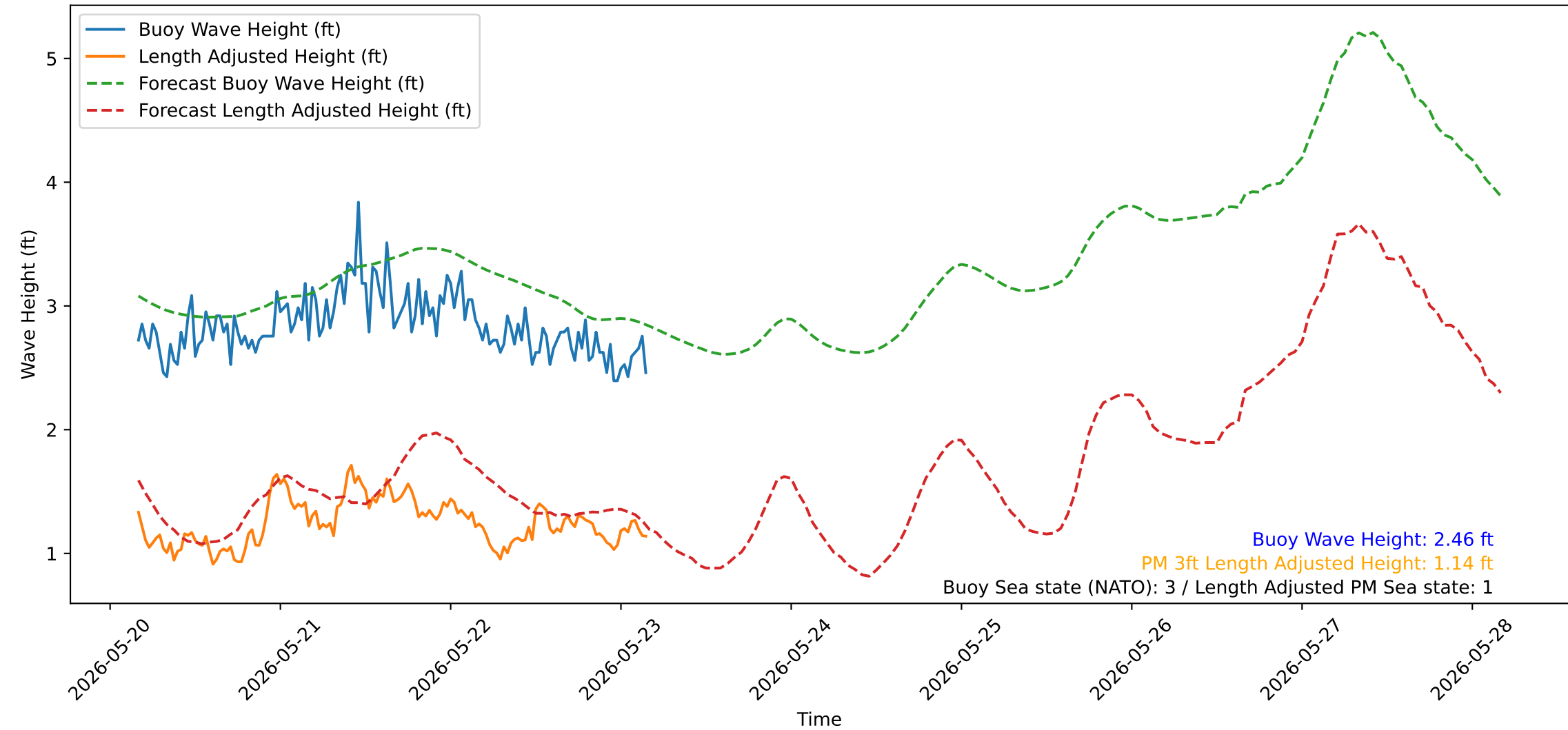
Wave Heights over Time for Oceanside Harbor at 2026-05-23 04:00:32
