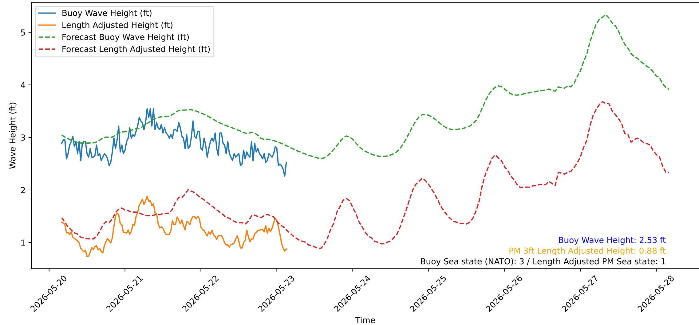
Wave Heights over Time for Green Beach at 2026-05-23 04:01:13
