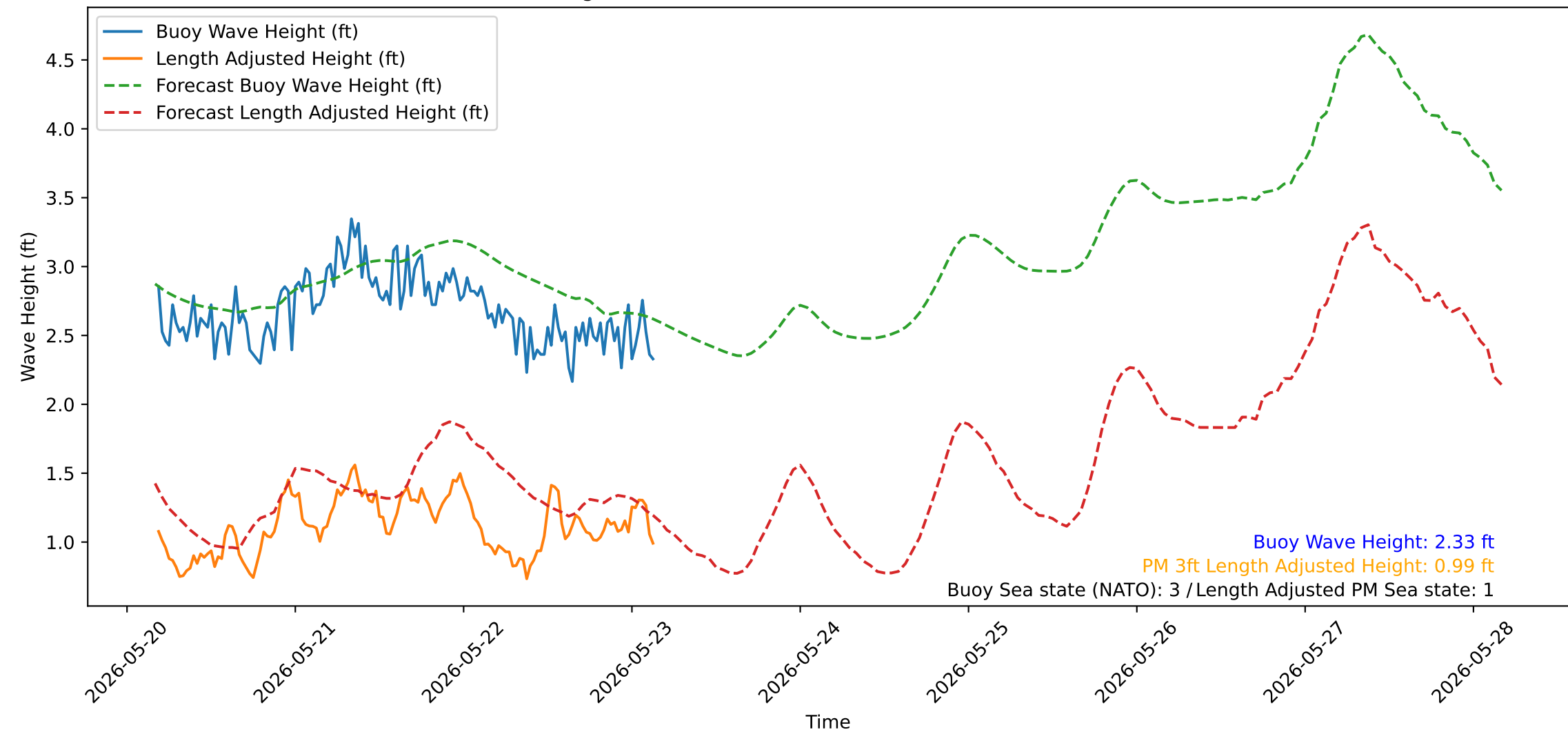
Wave Heights over Time for Red Beach at 2026-05-23 04:00:51
