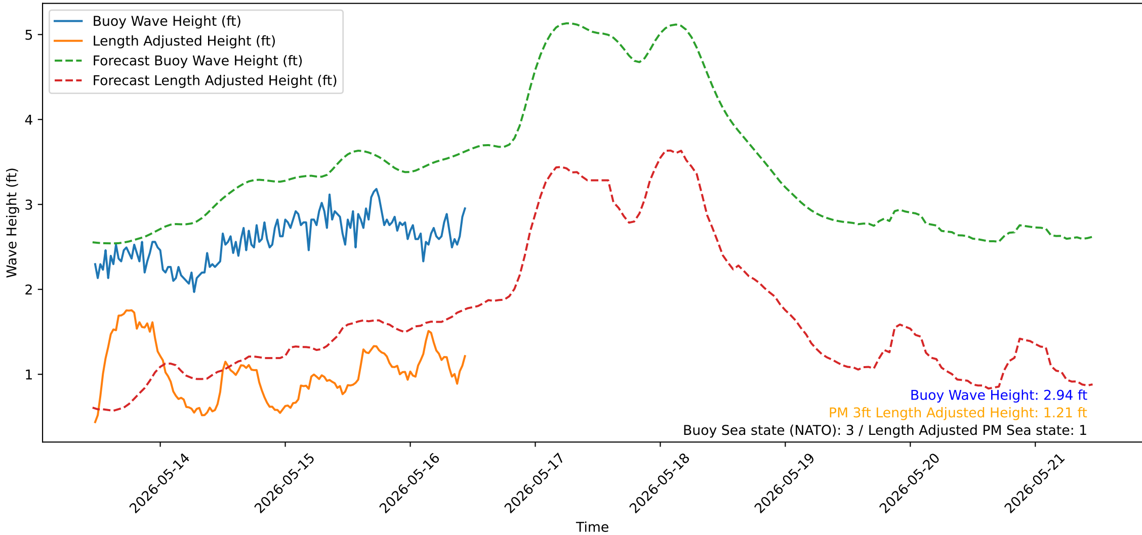
Wave Heights over Time for Red Beach at 2026-05-16 11:20:53
