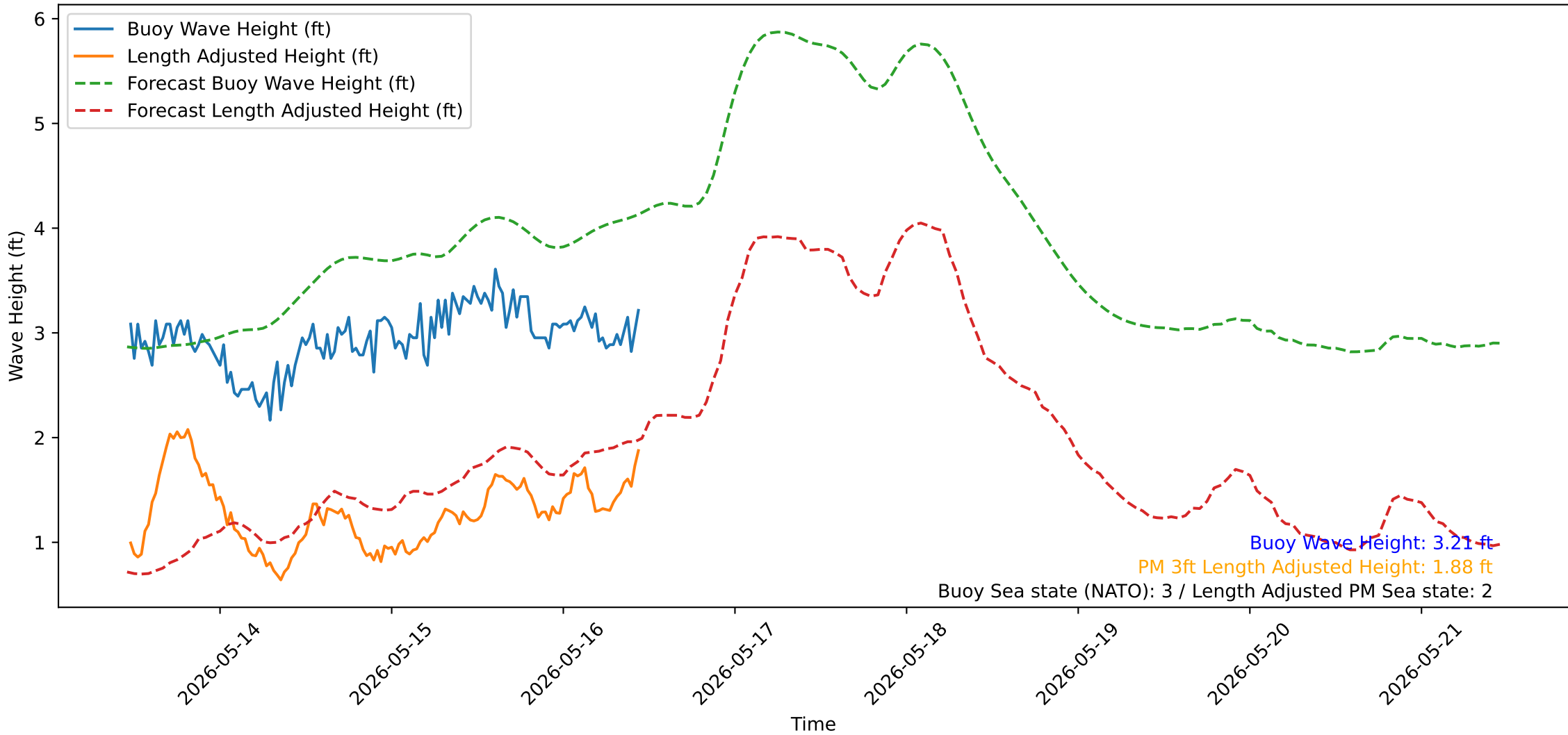
Wave Heights over Time for Oceanside Harbor at 2026-05-16 11:20:32
