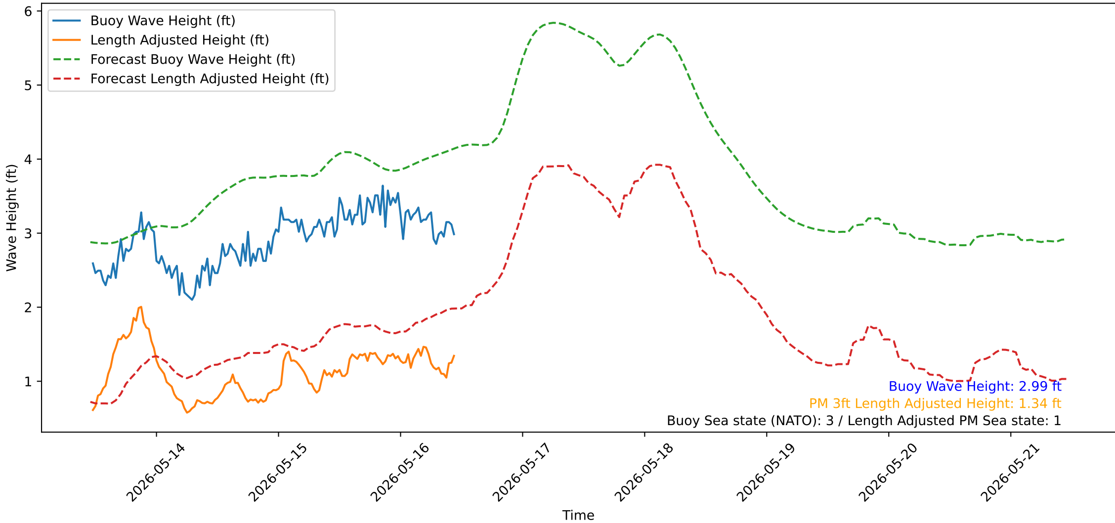
Wave Heights over Time for Green Beach at 2026-05-16 11:21:15
