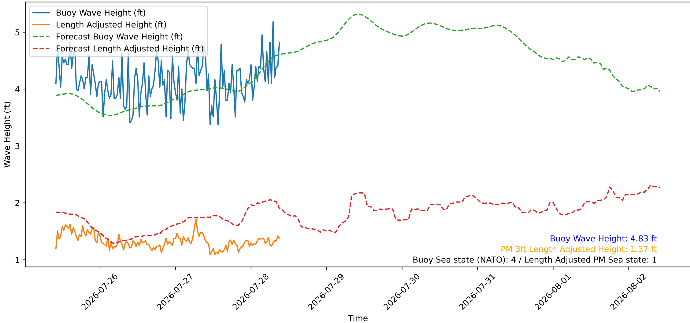
Wave Heights over Time for Green Beach at 2026-07-28 10:01:11
