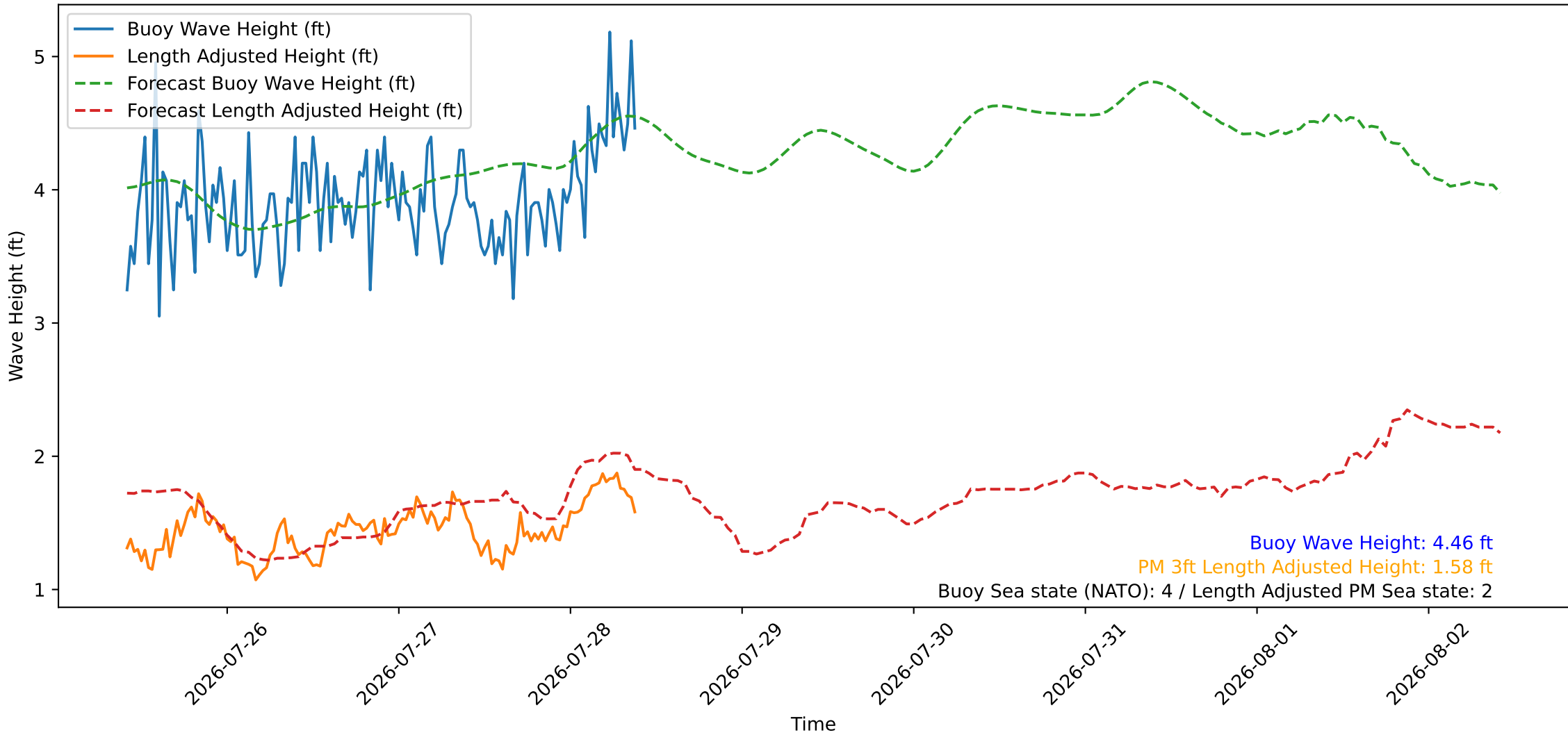
Wave Heights over Time for Oceanside Harbor at 2026-07-28 10:00:27
