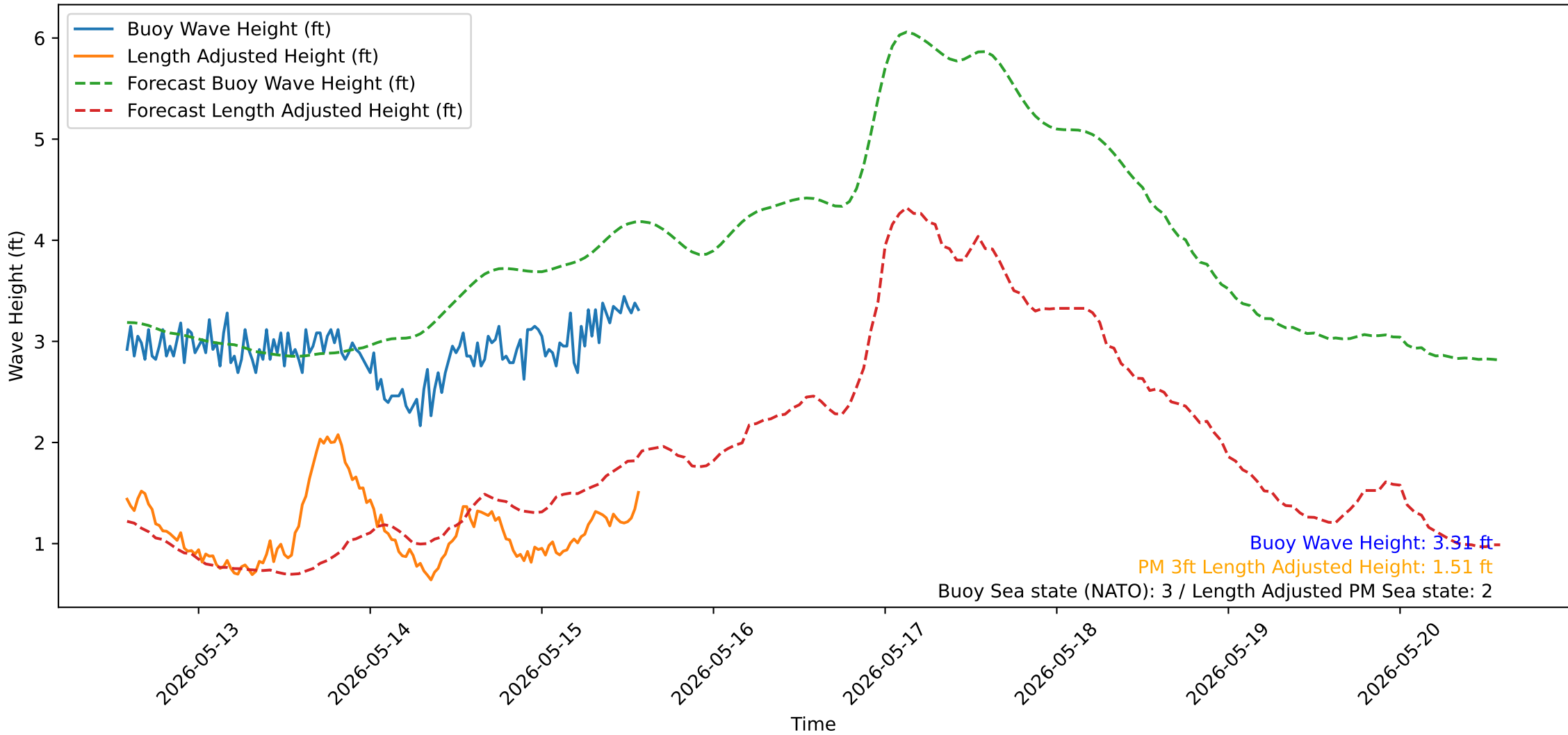
Wave Heights over Time for Oceanside Harbor at 2026-05-15 14:00:32
