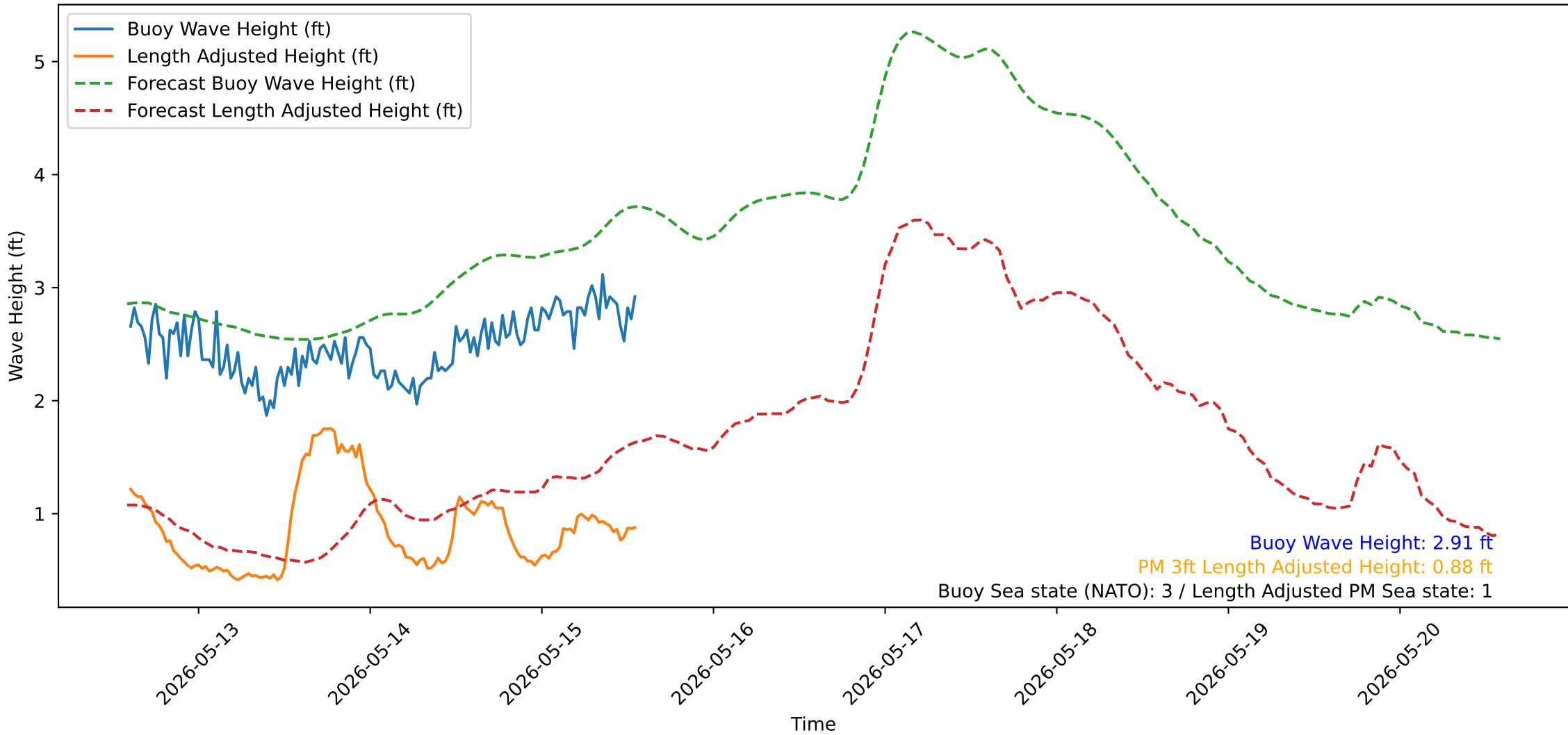
Wave Heights over Time for Red Beach at 2026-05-15 14:00:52
