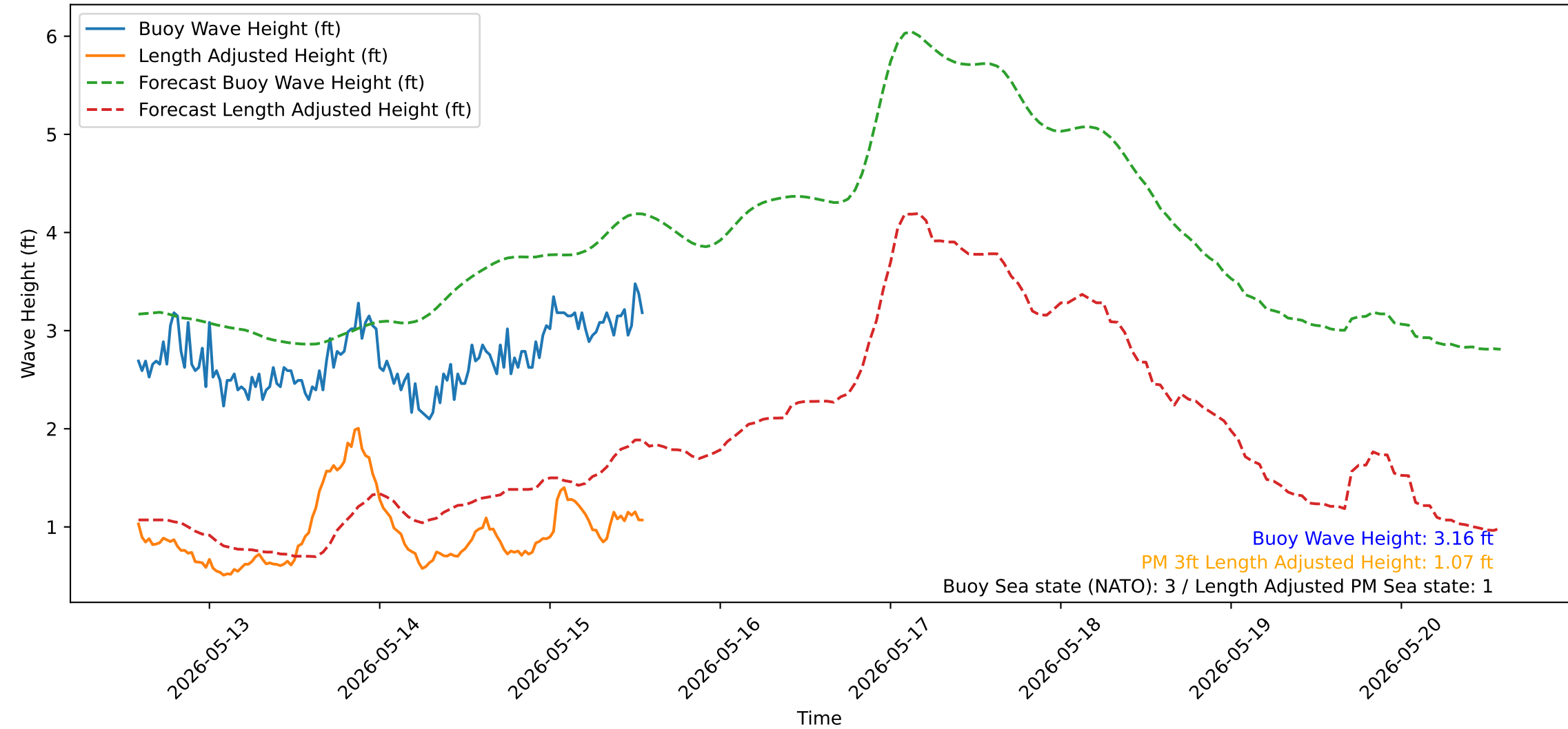
Wave Heights over Time for Green Beach at 2026-05-15 14:01:14
