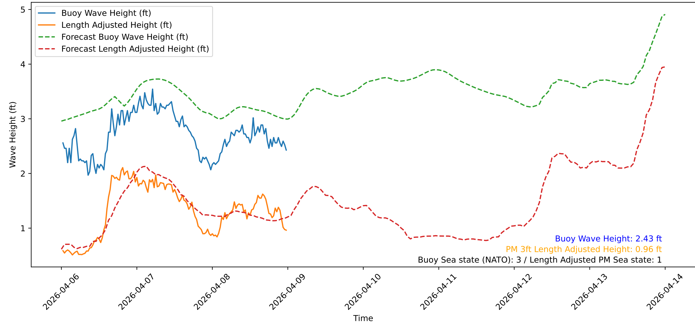
Wave Heights over Time for Red Beach at 2026-04-09 00:20:48
