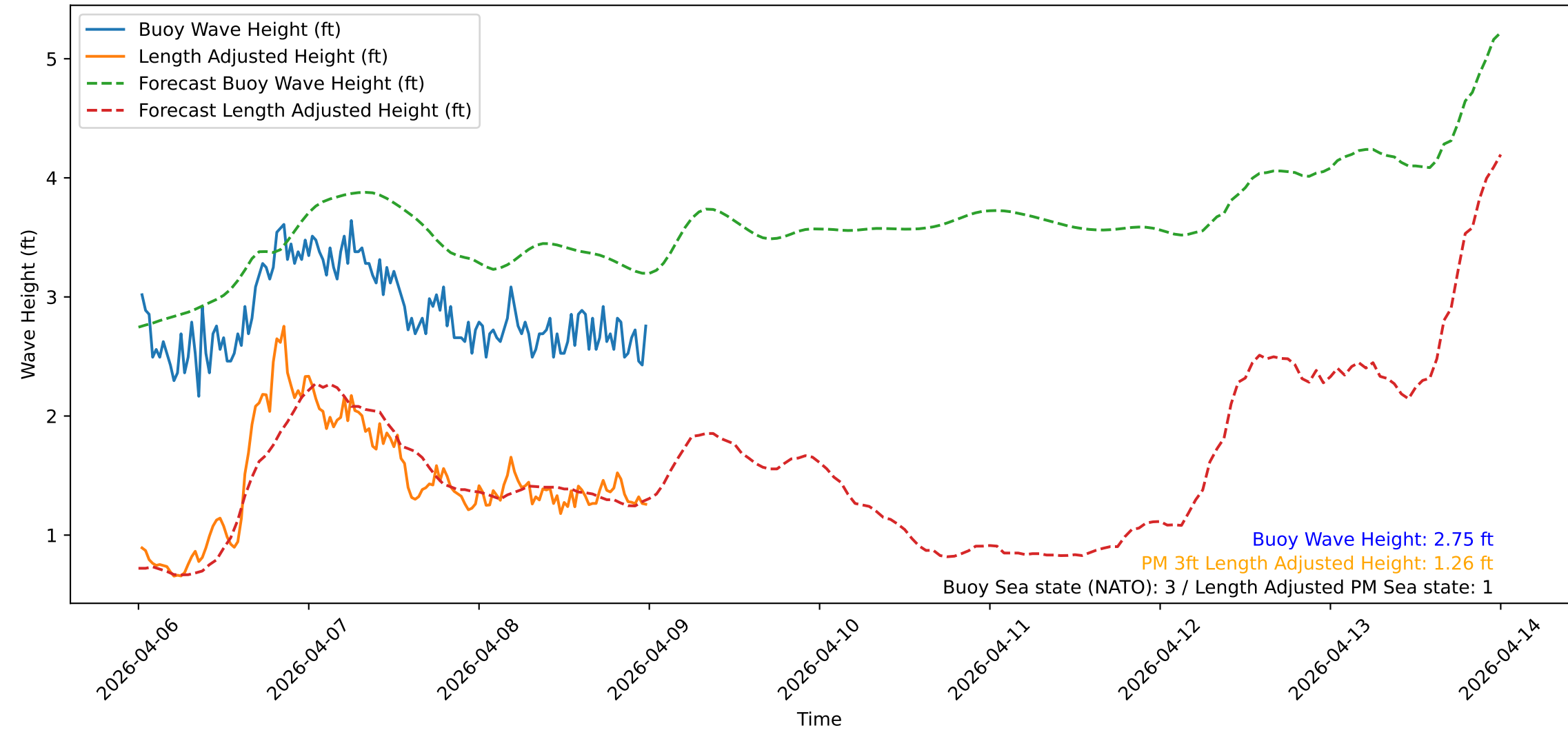
Wave Heights over Time for Oceanside Harbor at 2026-04-09 00:20:32
