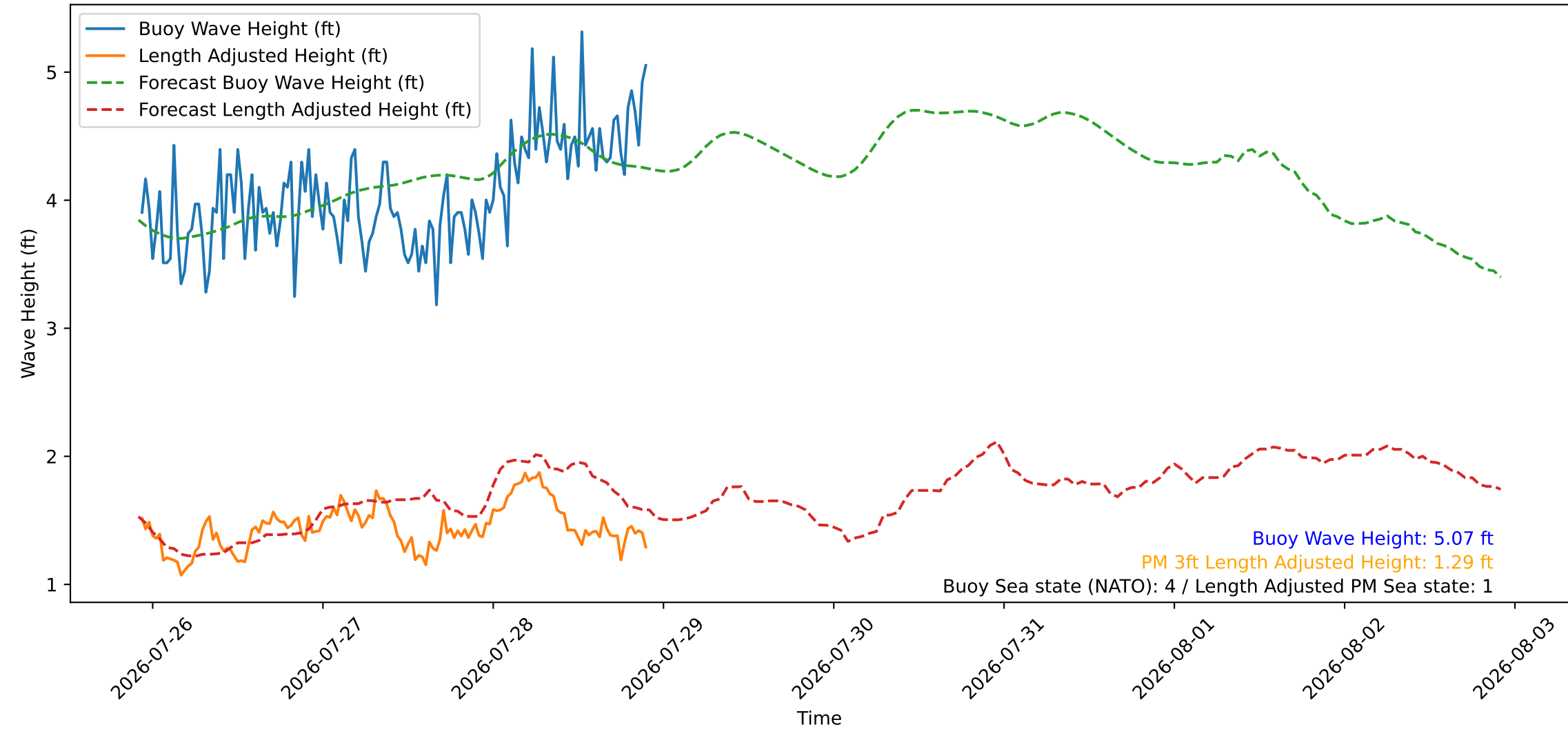
Wave Heights over Time for Oceanside Harbor at 2026-07-28 22:20:26
