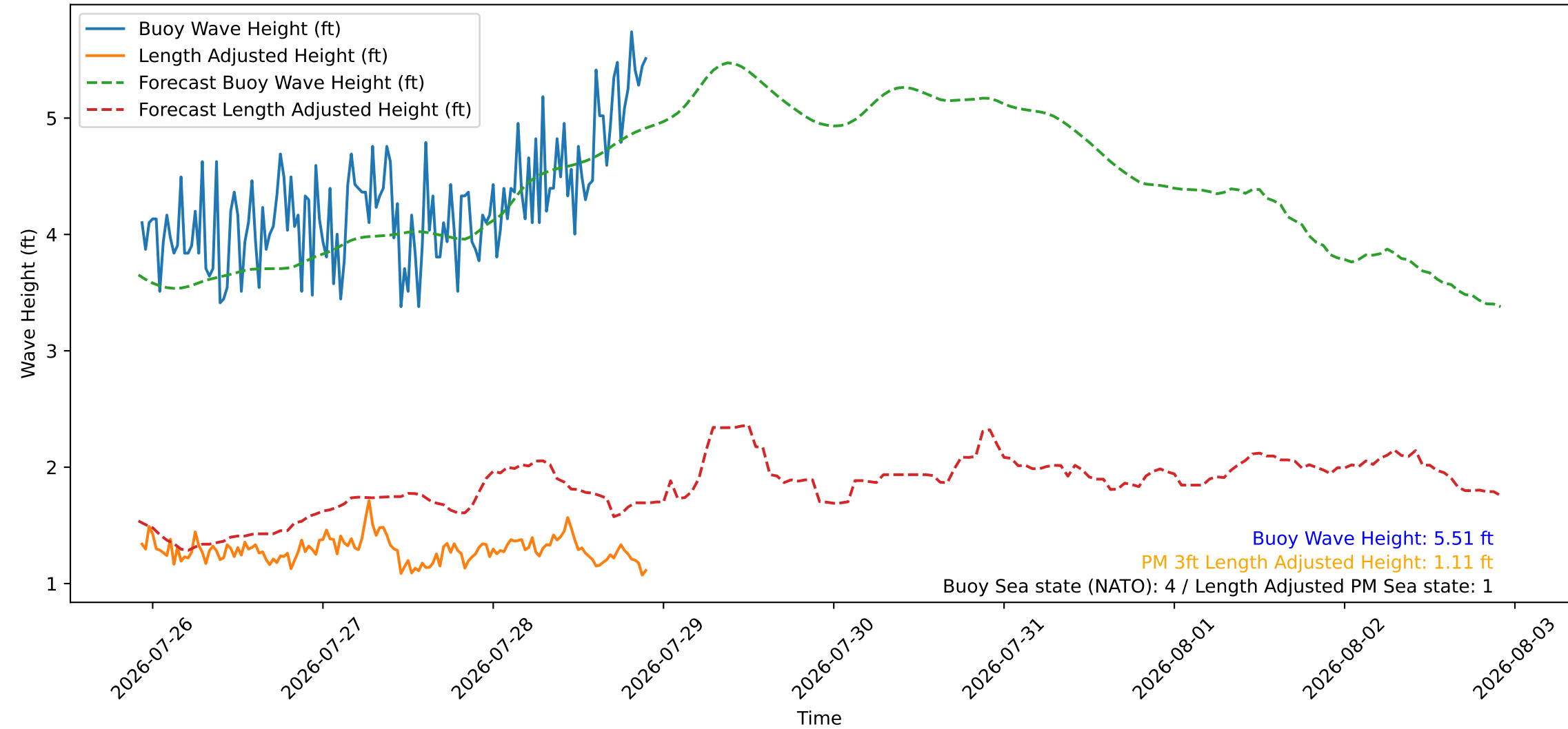
Wave Heights over Time for Green Beach at 2026-07-28 22:21:10
