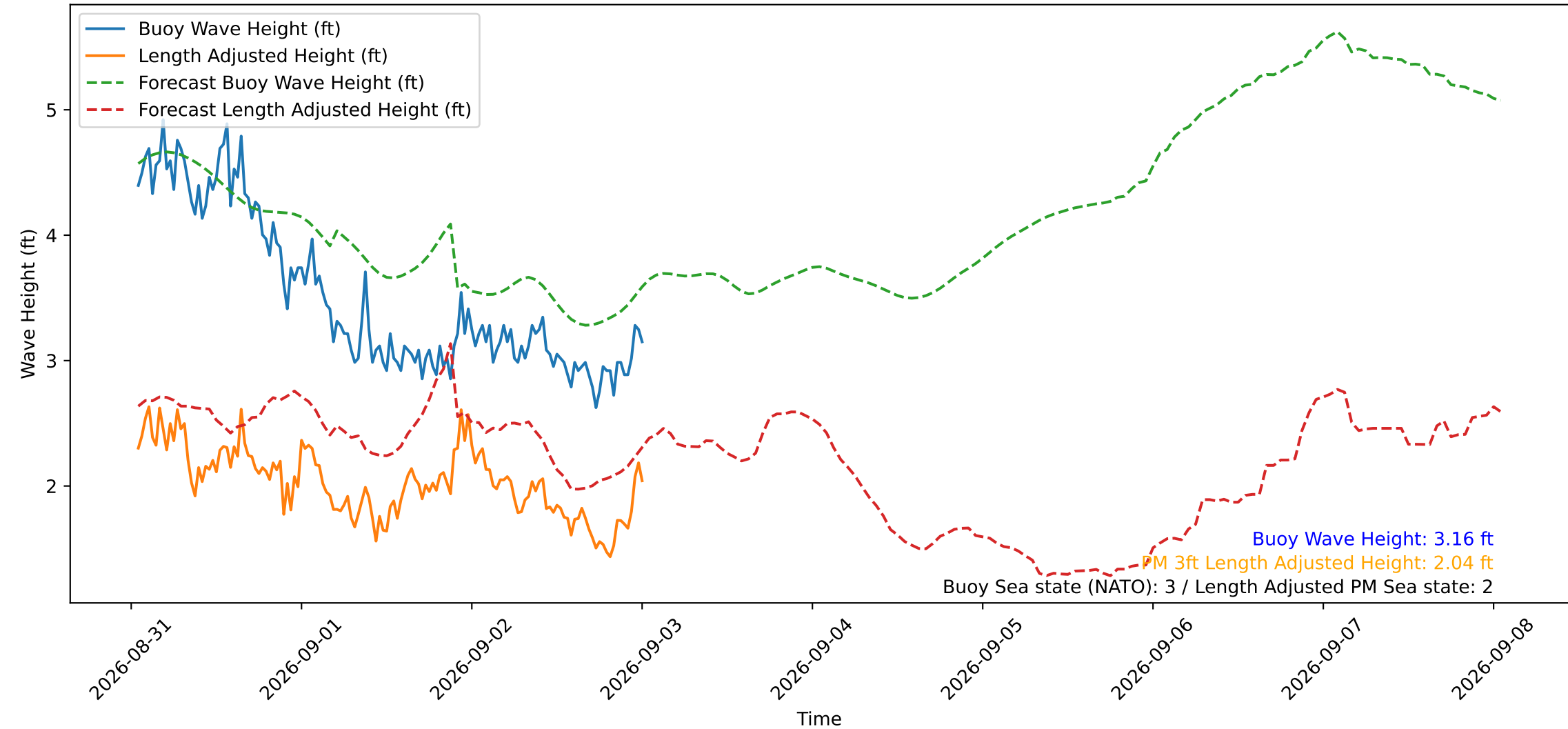
Wave Heights over Time for Oceanside Harbor at 2026-09-03 01:10:30
