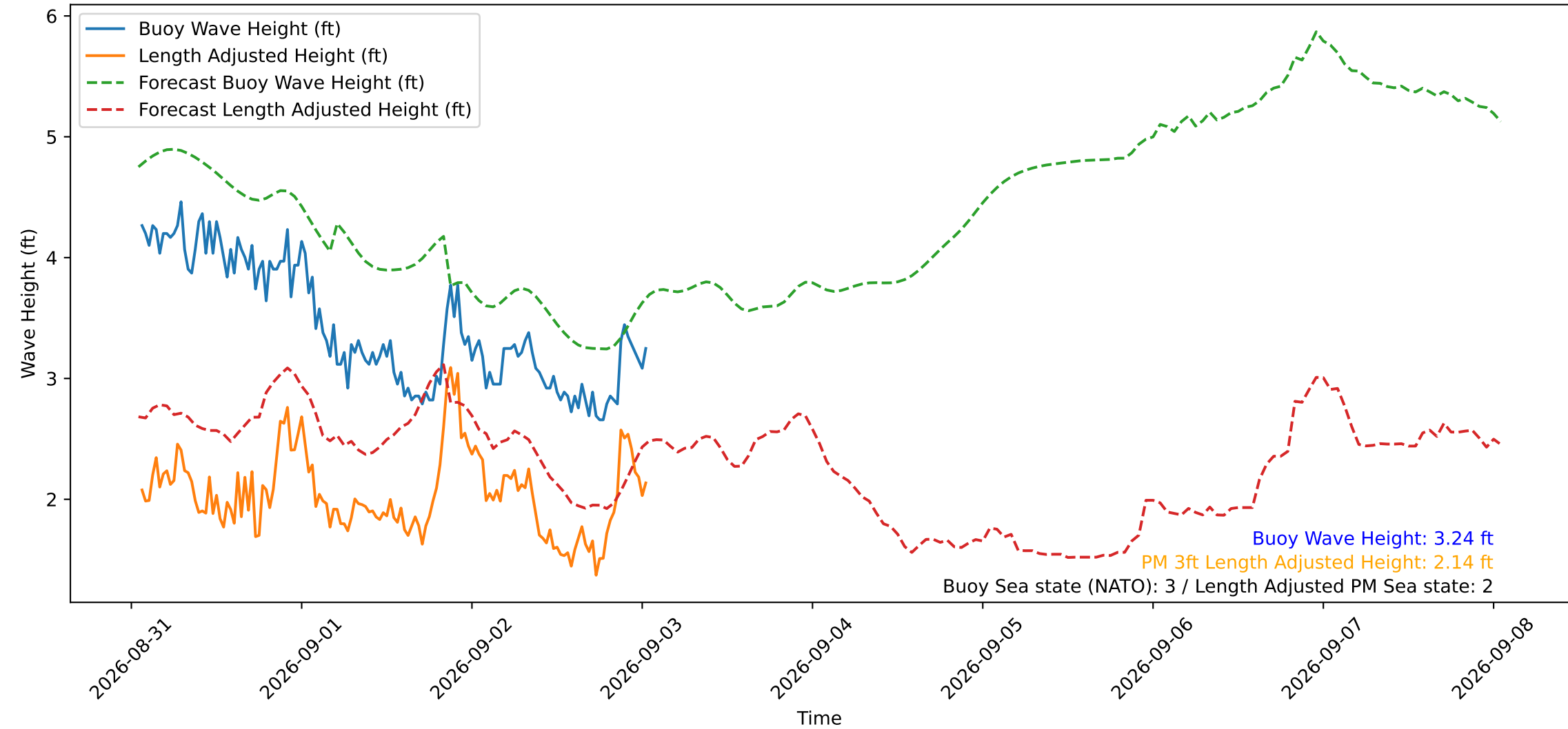
Wave Heights over Time for Green Beach at 2026-09-03 01:11:12
