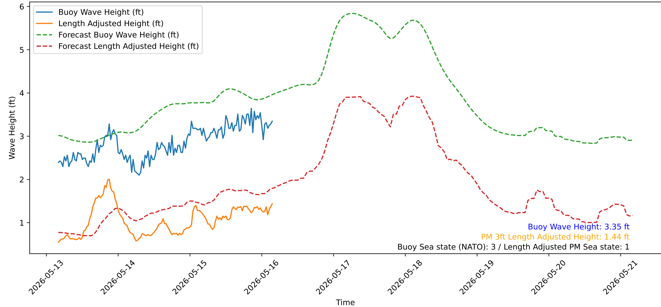
Wave Heights over Time for Green Beach at 2026-05-16 04:11:13
