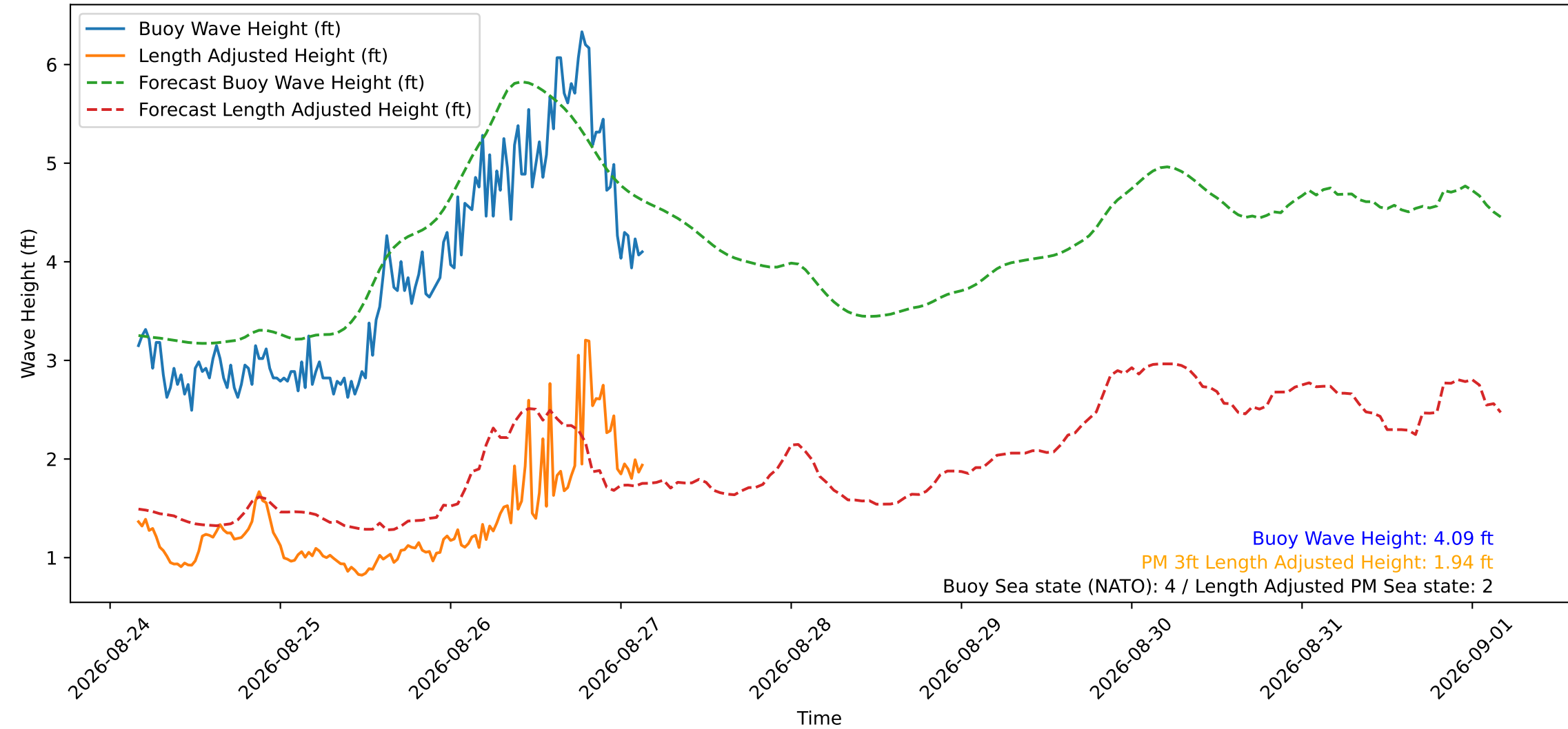
Wave Heights over Time for Green Beach at 2026-08-27 03:51:15
