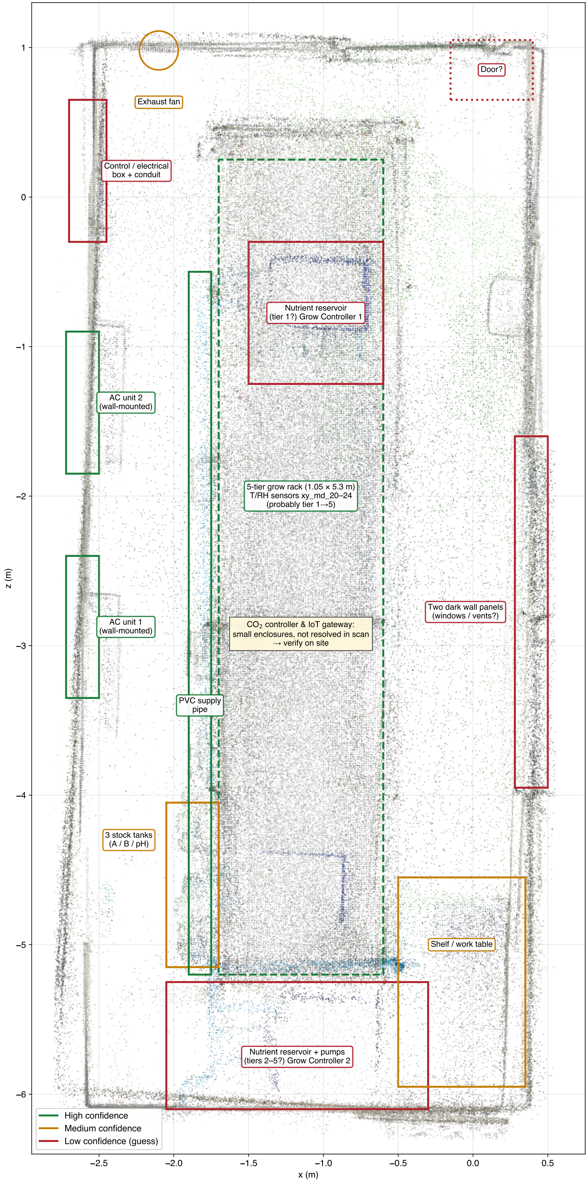
SIS-KU PFAL — plan view of LiDAR point cloud (0.02–2.4 m above floor) with inferred equipment locations
