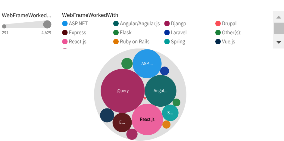
Top 10 WebFrameWorkedWith.
