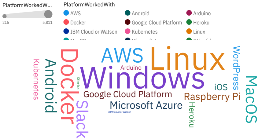
PlatformWorkedWith
