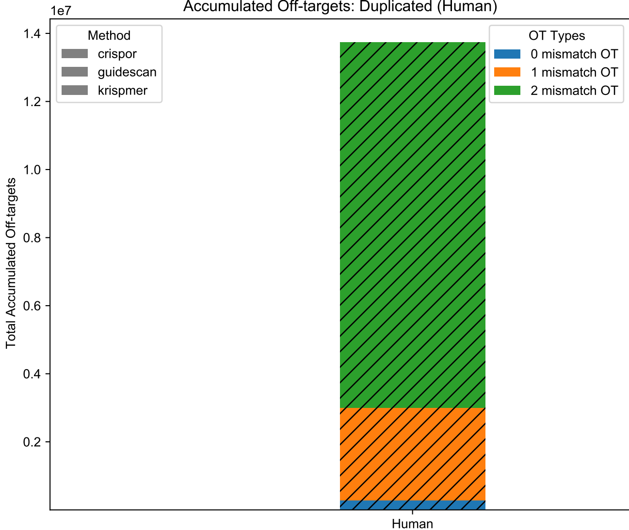
Accumulated Off-targets: Duplicated (Human)
