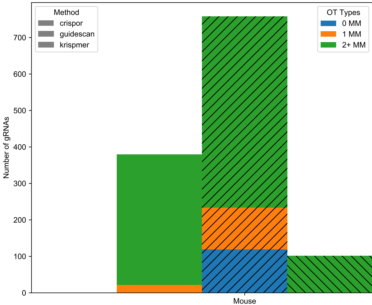
gRNAs with Off-targets: Intergenic (Mouse)
