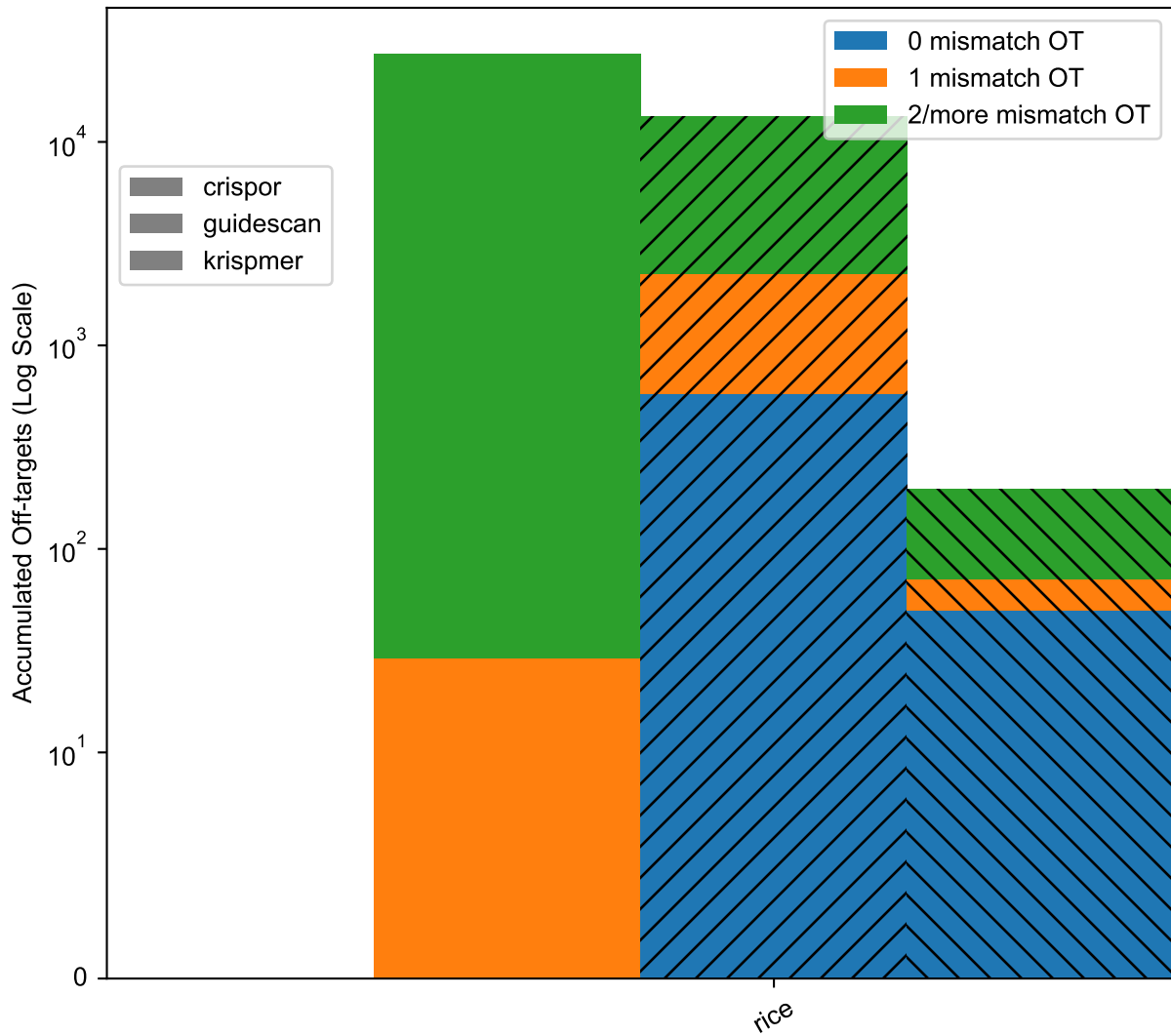
Accumulated Off-targets in protein coding regions
