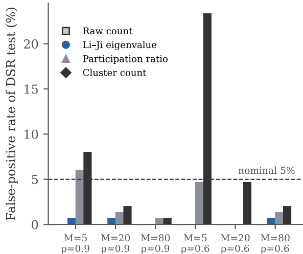
(b) Zero-skill winners declared significant
