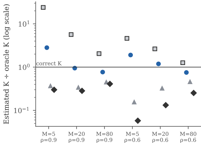
(a) Accuracy of effective-K estimates
