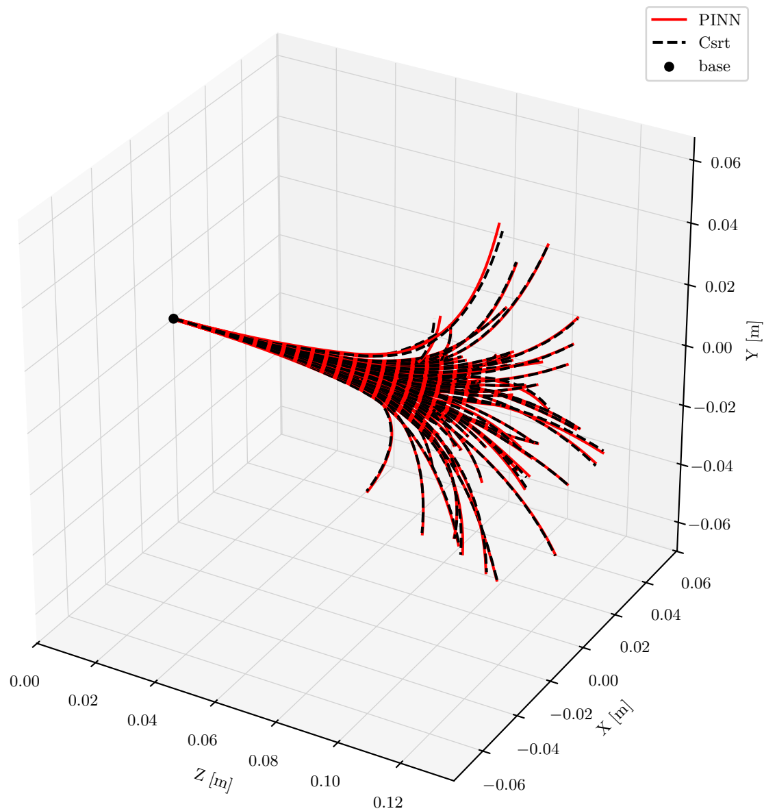
3D Backbone
