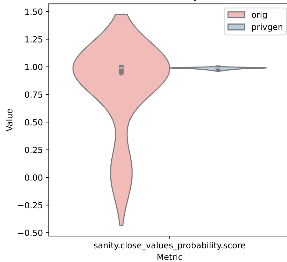
CloseValuesProbability: maximize
