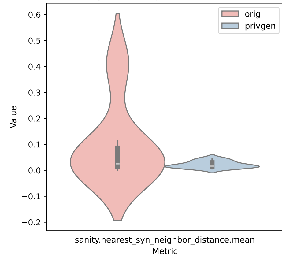
NearestSyntheticNeighborDistance: minimize
