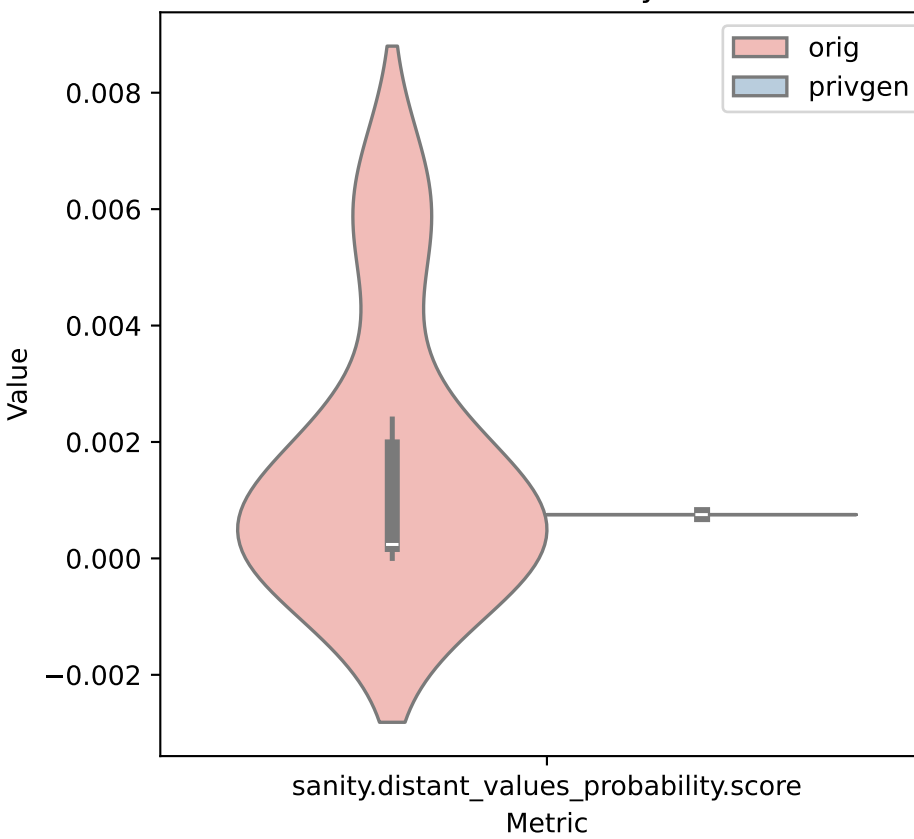
DistantValuesProbability: minimize
