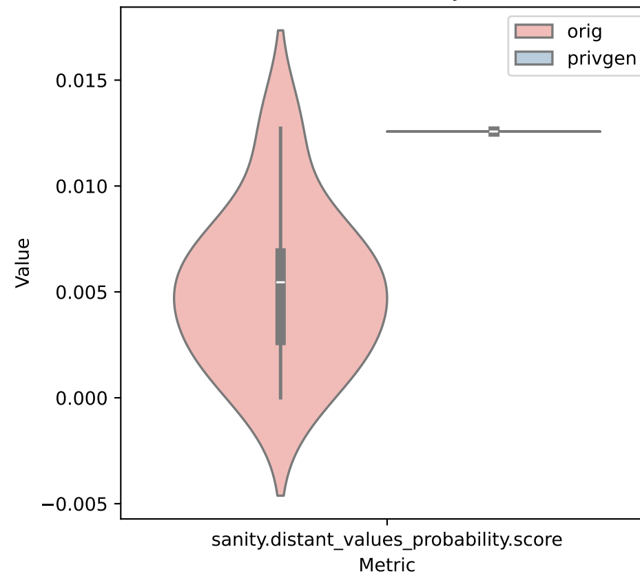
DistantValuesProbability: minimize
