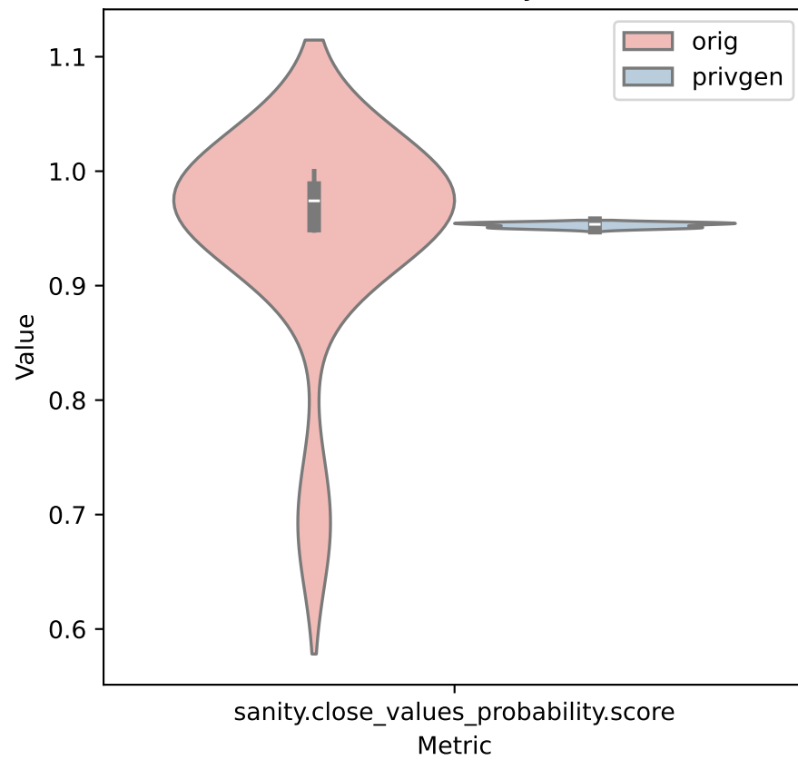
CloseValuesProbability: maximize
