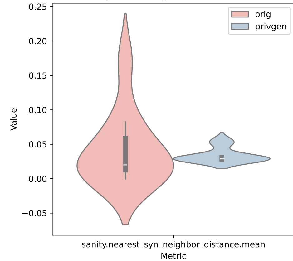
NearestSyntheticNeighborDistance: minimize
