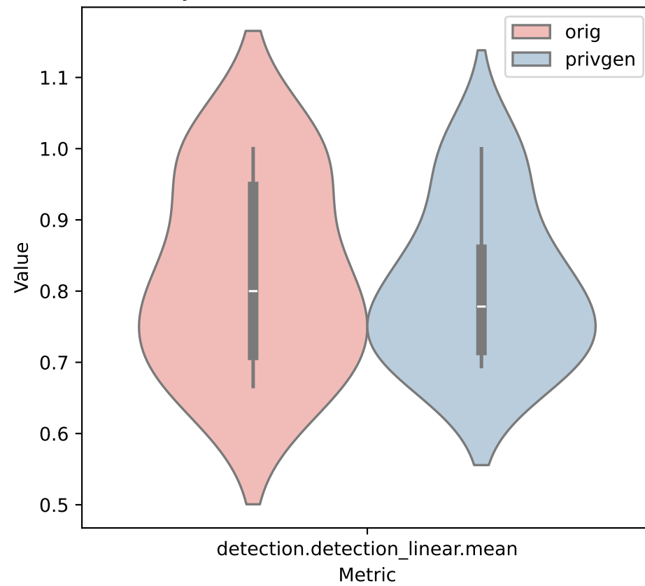
SyntheticDetectionLinear: minimize
