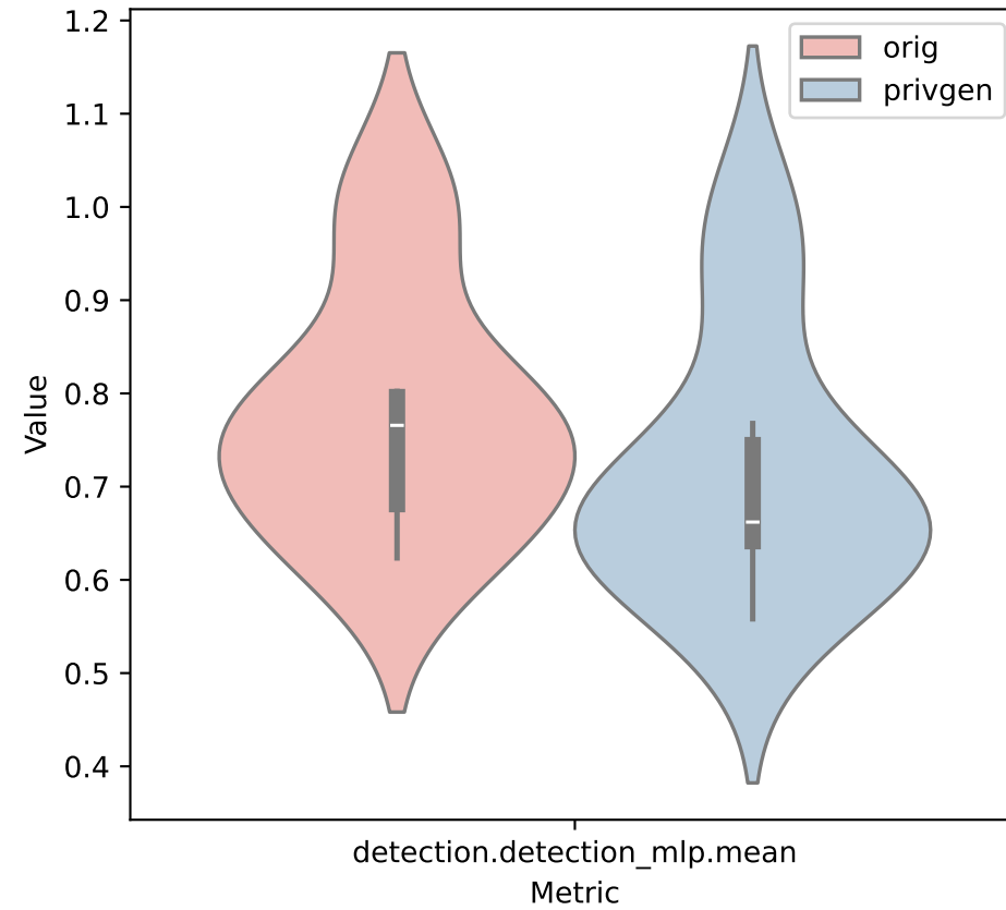
SyntheticDetectionMLP: minimize
