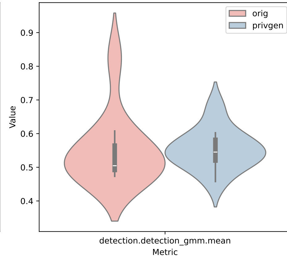
SyntheticDetectionGMM: minimize
