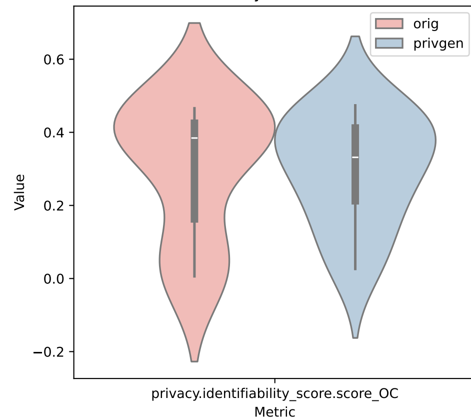
IdentifiabilityScore: minimize
