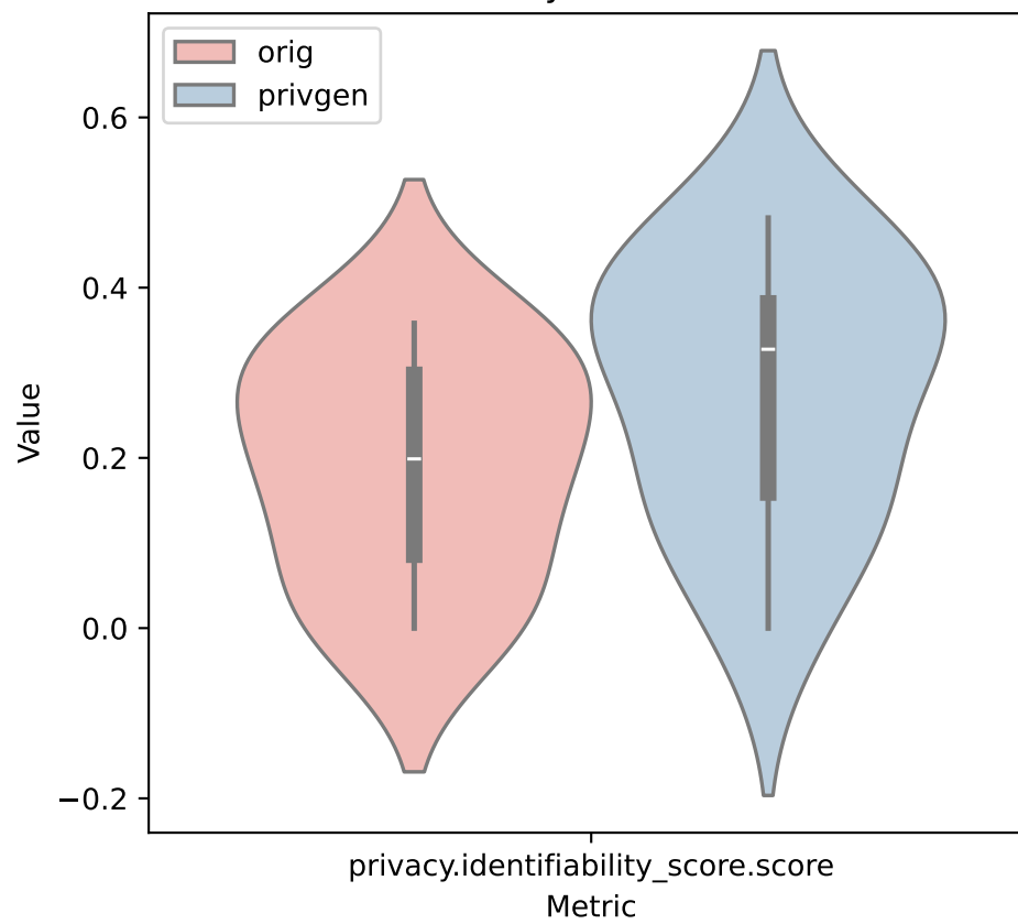
IdentifiabilityScore: minimize
