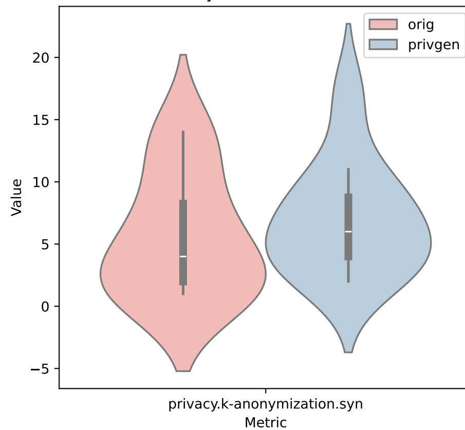
IdentifiabilityScore: minimize
