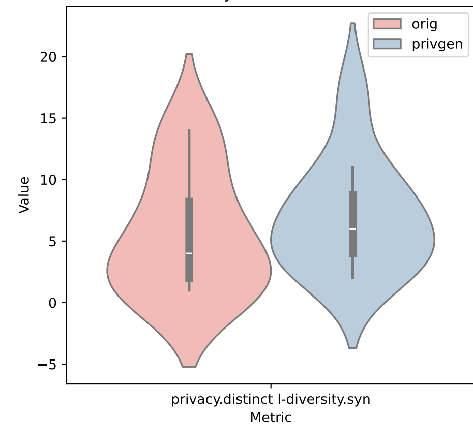
IDiversityDistinct: maximize
