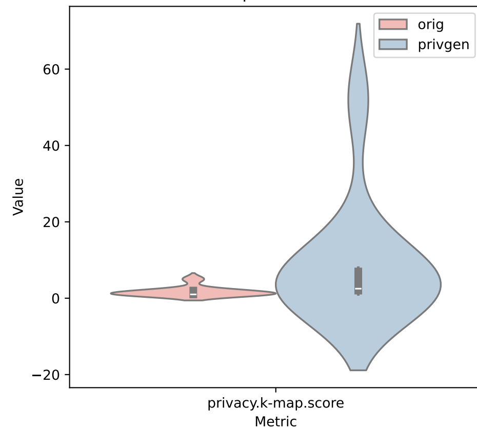
IdentifiabilityScore: minimize
