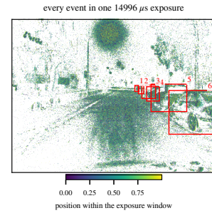
Figure 7. Every event inside one published 14 996 \mu s exposure window of zurich_city_09_a , colored by its position within that window, with that frame's released boxes numbered left to right. The frame is the median-dispersion one of 602 eligible candidate frames with at least six qualifying boxes, not the largest.
