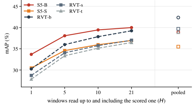
Figure 3. mAP of the five checkpoints on the common frames at H = 1, 5, 10, 21 (filled markers, equal spacing on the axis) and in the pooled released evaluation (open markers). RVT-t and S5-B coincide at the pooled position. Intervals are in Tab. 3 and the paired gaps in Tab. 4.
