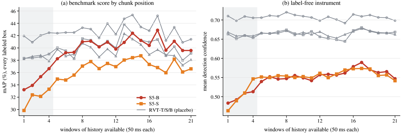
Figure 4. The chunk-position contrast at each of the 21 positions. (a) mAP over every labeled box, the top panel of main Fig. 1 at full width. (b) Mean detection confidence at the same positions, which uses neither the ground truth nor the evaluator. Both panels separate the two SSM checkpoints from the three RVT placebos in the same direction, so the contrast is present upstream of the matching rule. Shaded: the one-to-four-window block.
