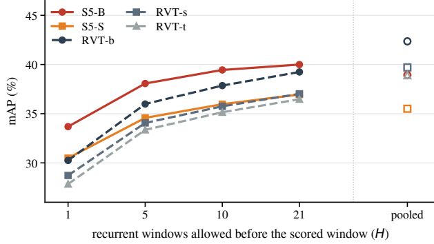
Figure 5. mAP of the five checkpoints on the common frames at H = 1, 5, 10, 21 (filled markers, equal spacing on the axis) and in the pooled released evaluation (open markers). RVT-t and S5-B coincide at the pooled position. Intervals are in main Tab. 1 and the paired gaps in Tab. 9.
