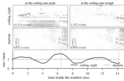
Figure 8. Top: 350 \mu s slices of the ceiling-exposure sequence zurich_city_09_a and of the daytime control, at the peak and trough of the ceiling sequence's own event rate inside its densest published exposure window. Bottom: that rate in 350 \mu s bins, each sequence normalized to its own mean. The ceiling rate moves by a factor of 3.0 between its extremes, the daytime rate by 1.1.
