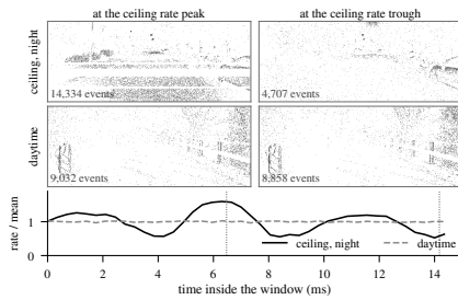
Figure 4. Top: 350 \mu\text{s} slices of the ceiling-exposure sequence zurich_city_09_a and of the daytime control, at the peak and trough of the ceiling sequence's own event rate inside its densest published exposure window. Bottom: that rate in 350 \mu\text{s} bins, each sequence normalized to its own mean. The ceiling rate moves by a factor of 3.0 between its extremes, the daytime rate by 1.1.
