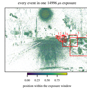
Figure 3. Every event inside one published 14996 \mu s exposure window of zurich_city_09_a , colored by its position within that window, with that frame’s released boxes numbered left to right. The frame is the median-dispersion one of 602 eligible candidate frames with at least six qualifying boxes, not the largest.
